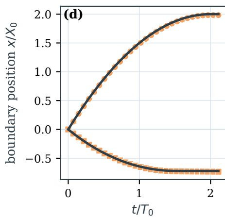
5° inclined bed
