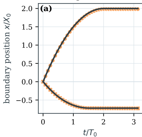
5° inclined bed
