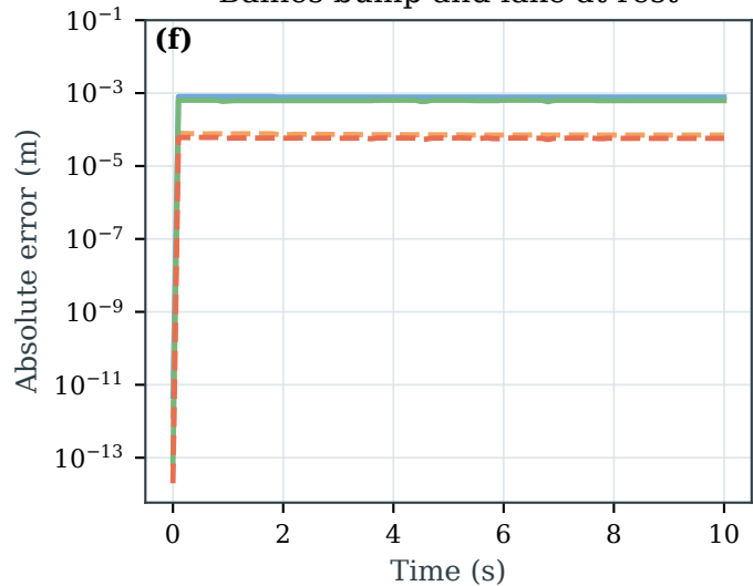
Baines bump and lake at rest
