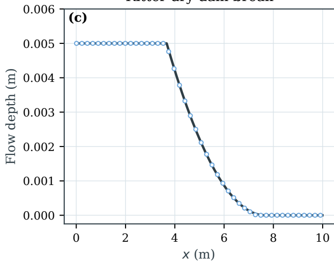
Ritter dry dam break
