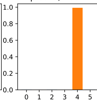
pred. 4, true 4
