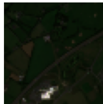
pred. 5, true 4
