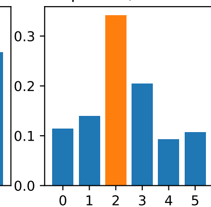
pred. 2, true 2
