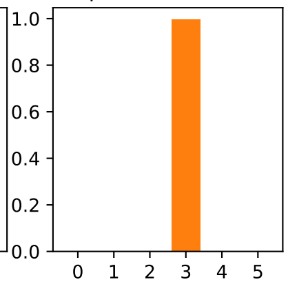
pred. 3, true 3
