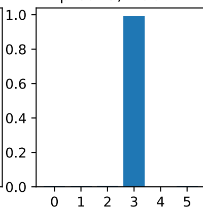
pred. 3, true -1
