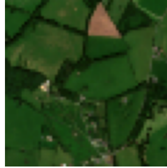
pred. 4, true 4
