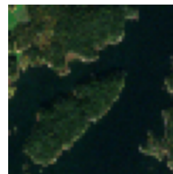
pred. 2, true -1
