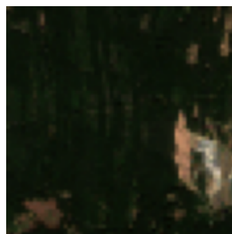
pred. 2, true 2
