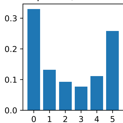
pred. 0, true -1
