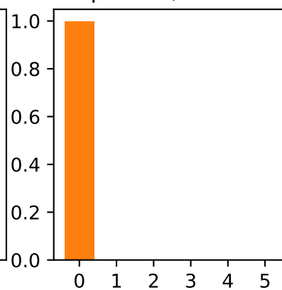
pred. 0, true 0
