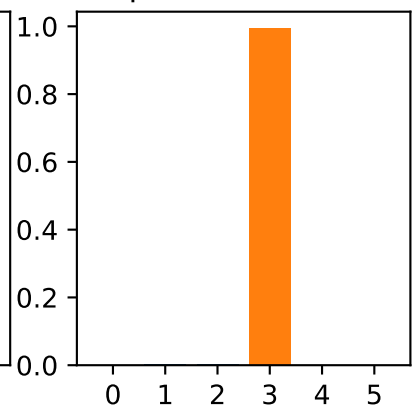
pred. 3, true 3
