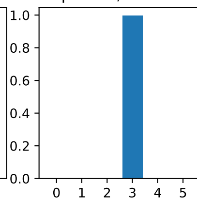
pred. 3, true -1
