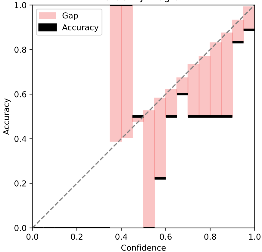
Reliability Diagram
