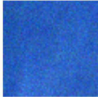
pred. 3, true -1
