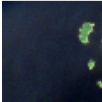
pred. 3, true 3
