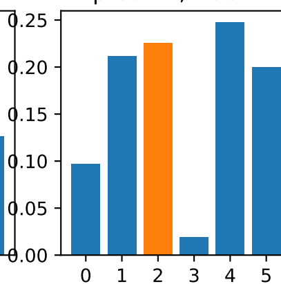
pred. -1, true 2
