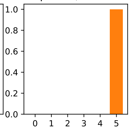
pred. 5, true 5
