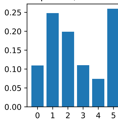
pred. 5, true -1
