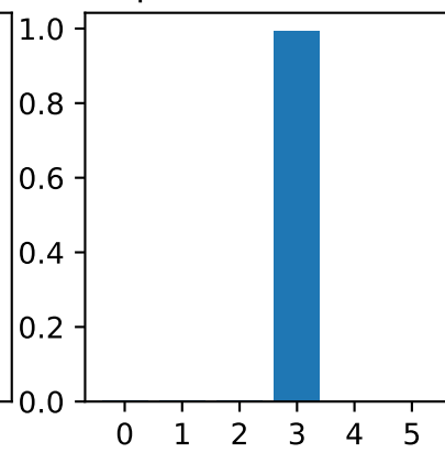
pred. 3, true -1
