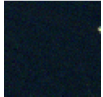
pred. 3, true 3
