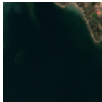
pred. 3, true -1
