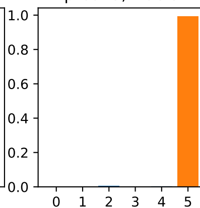
pred. 5, true 5
