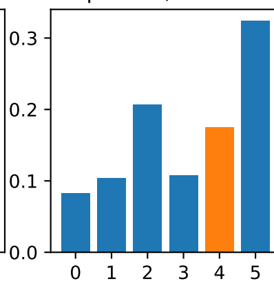
pred. 5, true 4
