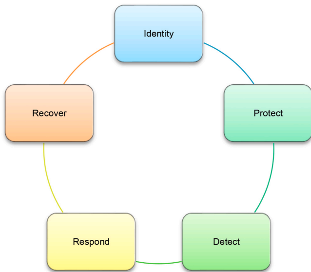
Fig. 29. Cybersecurity framework [275].
