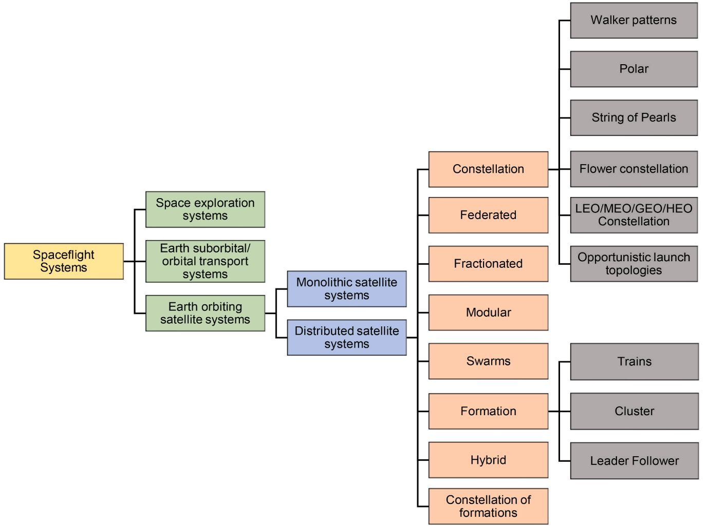
Fig. 1. Classification of spaceflight systems.
