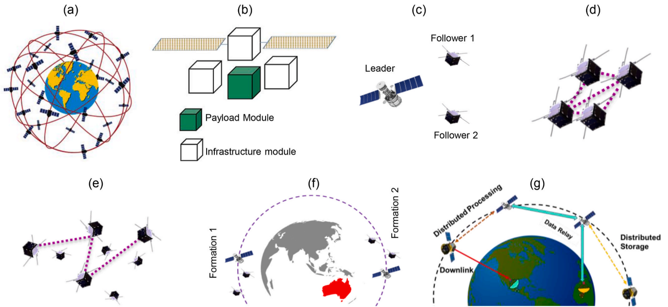
Fig. 7. DSS types (a) constellation (b) fractionated (c) formation (d) cluster (e) swarms (f) constellation of formation (g) federated.
