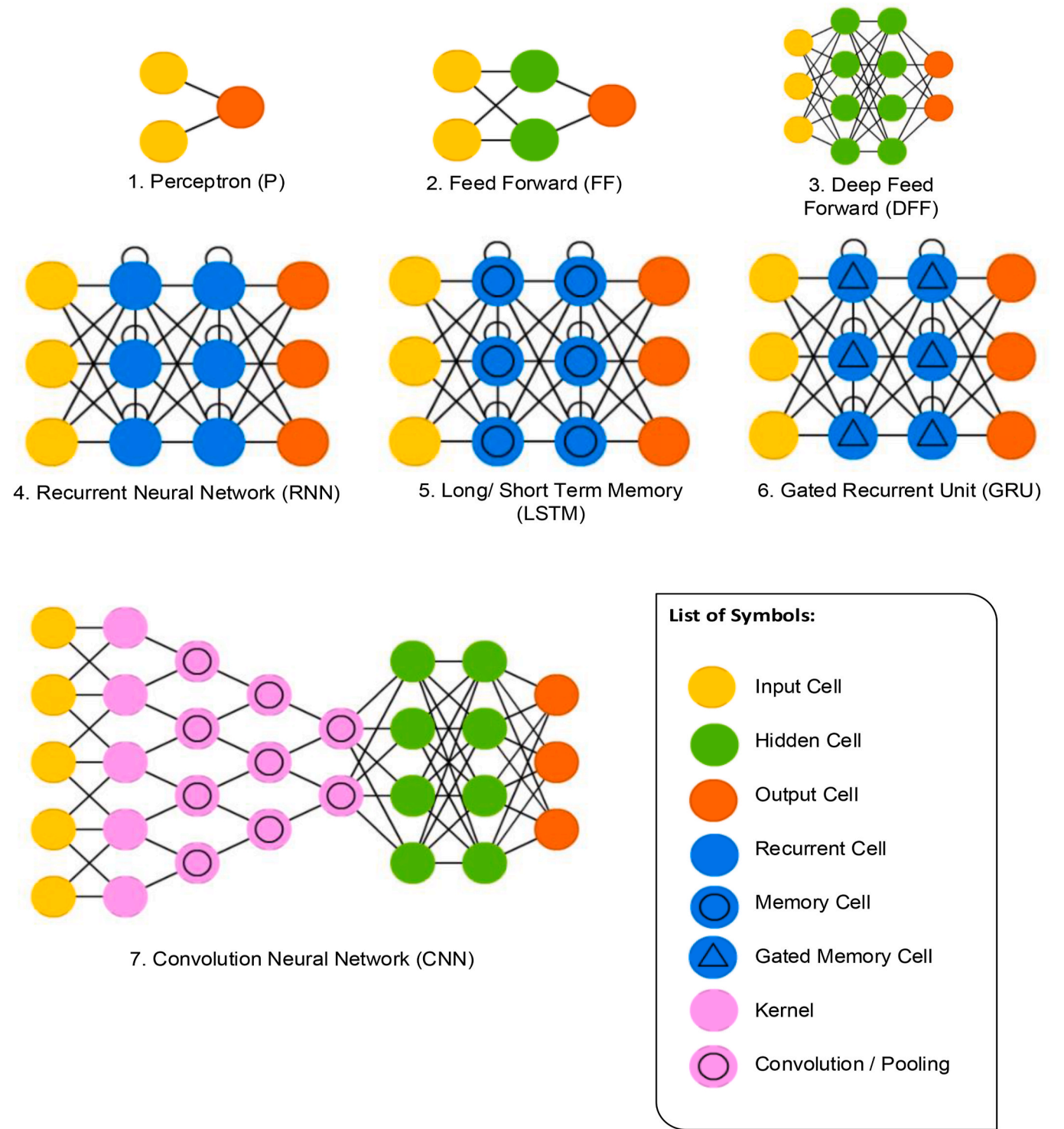
Fig. 21. Neural Network Categories [81].
