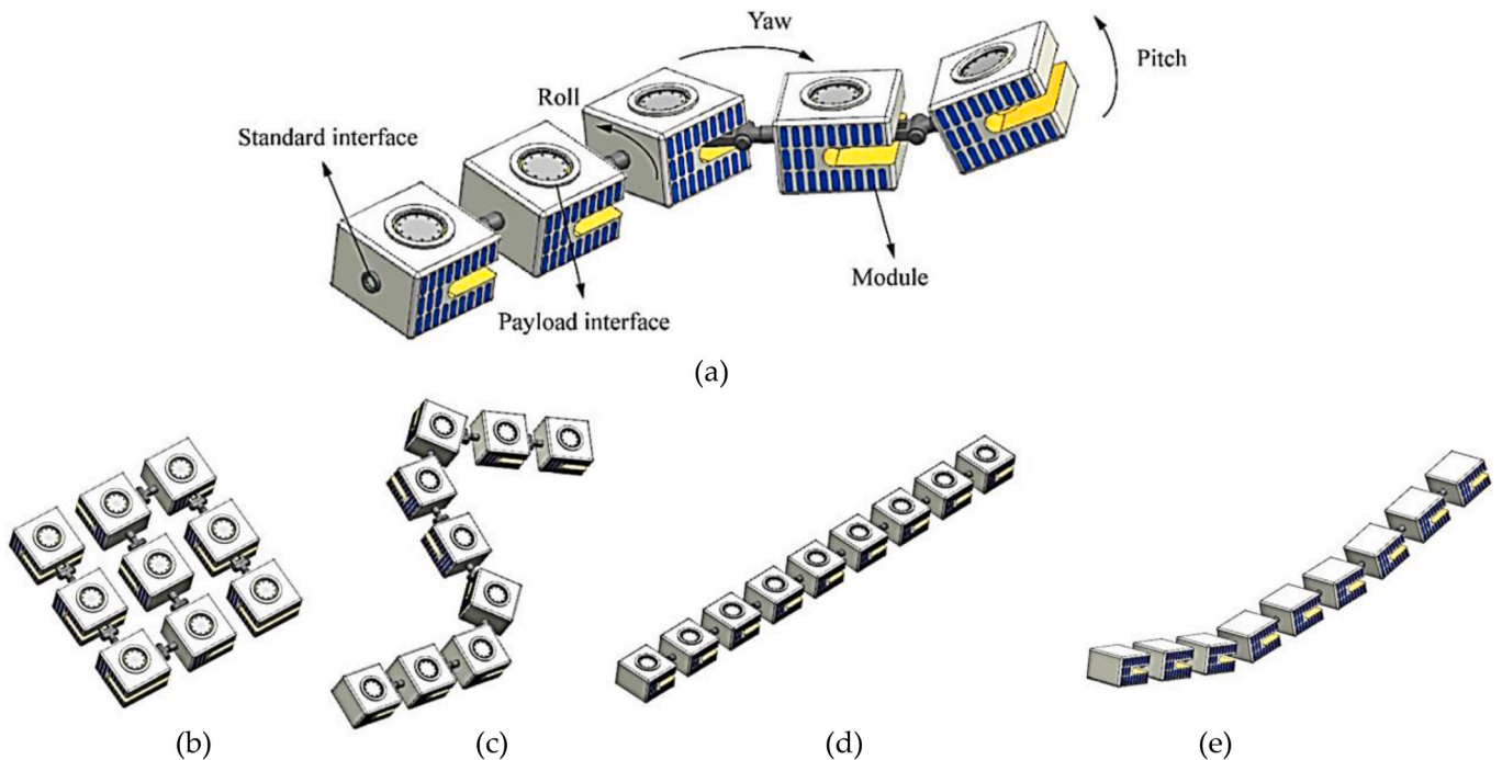
Fig. 8. Concept of SMSRS (a) and deployment stages: (b) folded state; (c) unfolding; (d) unfolded state; and (e) working configuration. Adapted from Ref. [52].
