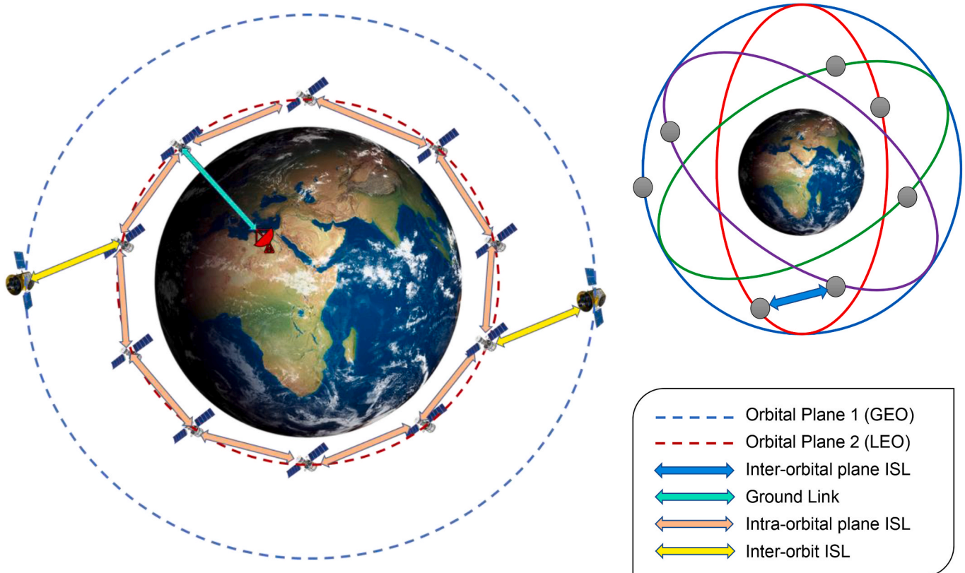
Fig. 26. Links between spacecraft and ground segment.
