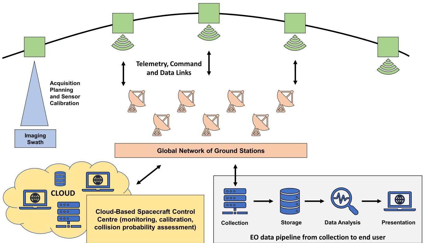
Fig. 11. DSS architecture entailing cloud-based control segment. Adapted from Ref. [20].
