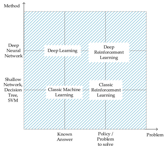
Fig. 22. Classification Standard [104].
