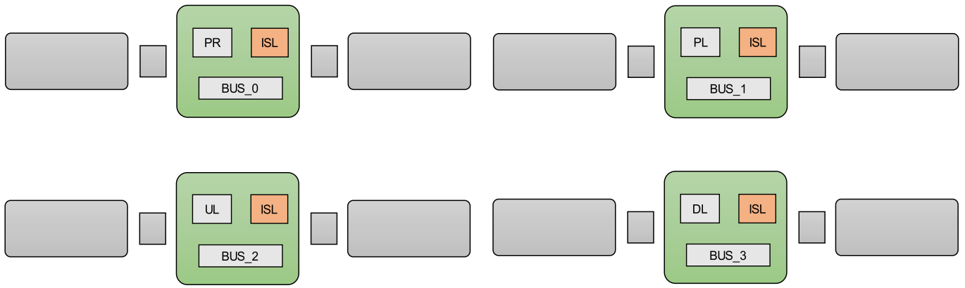
Fig. 10. DSS architecture. PR: Processor, DL: Downlink, PL: Payload are fractionated and distributed and connected through ISL. Adapted from Ref. [14].
