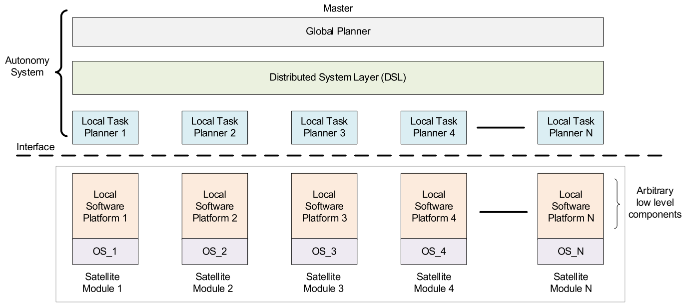
Fig. 12. Distributed software architecture. Adapted from Ref. [36].
