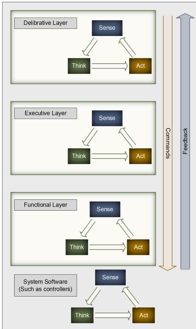
Fig. 14. The “sense-think-act” cycle autonomous system layered architecture [67].
