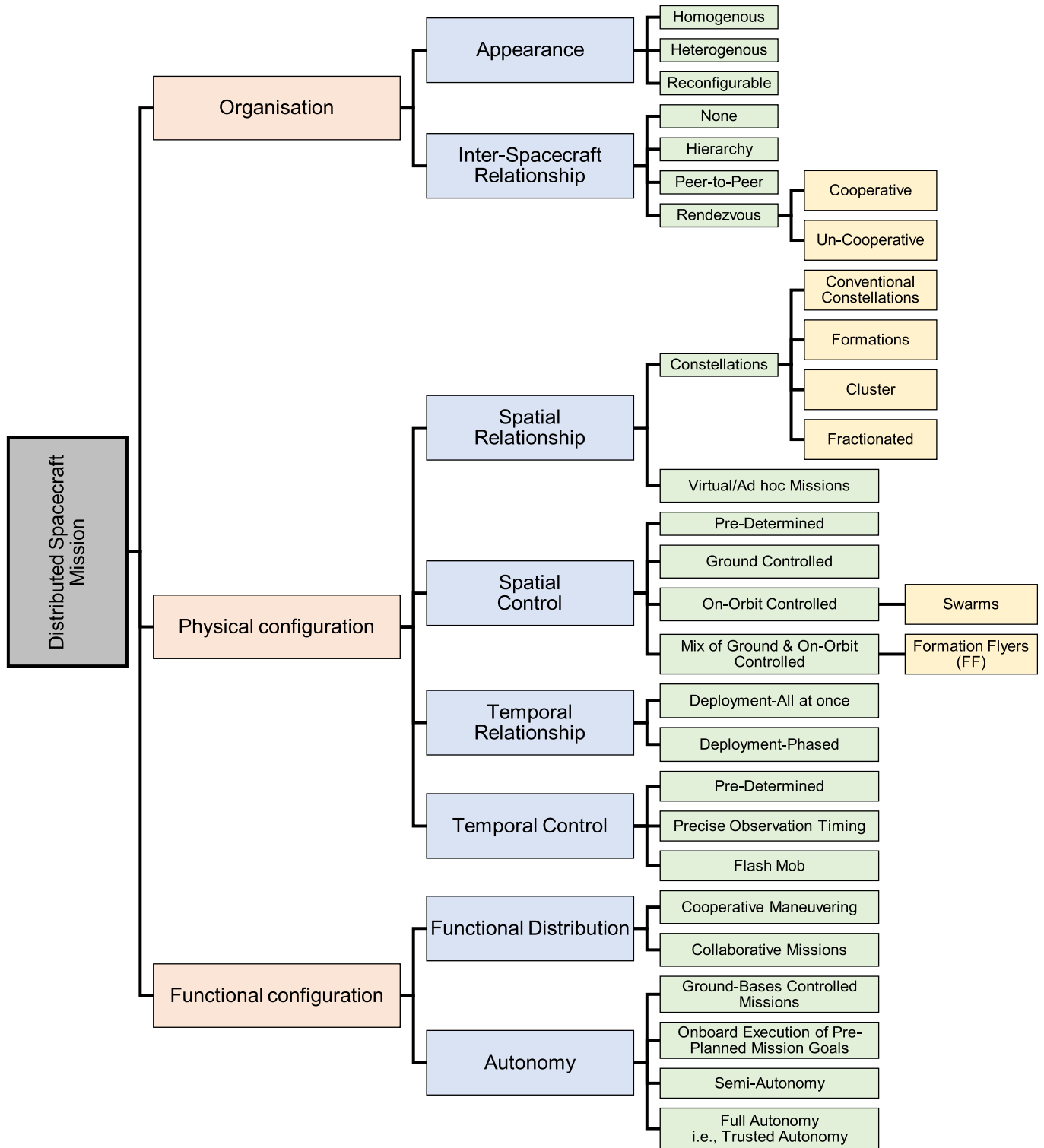
Fig. 9. DSM classification. Adapted from Ref. [62].
