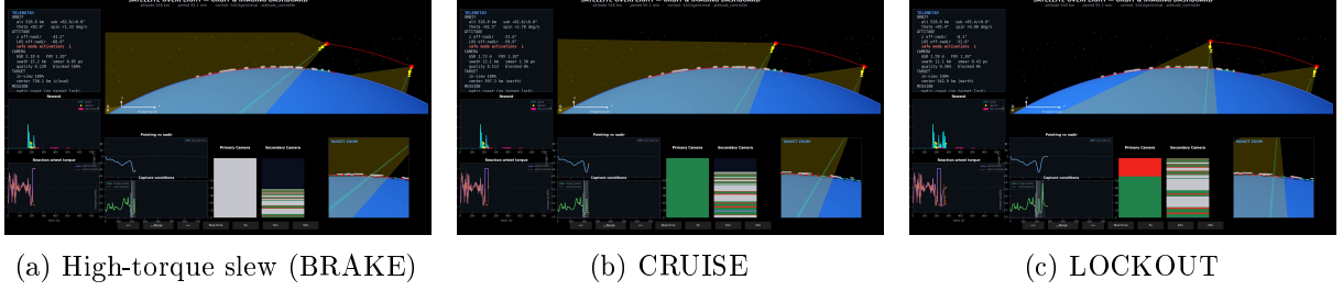
Figure 4: One attitude-safety cycle in torque-mode evaluation (same episode; panels use the recovery-phase names BRAKE / CRUISE / LOCKOUT). (a) High-torque slew: the agent commands large torque and reaches \approx 43^\circ off-nadir; safe mode activates (BRAKE) and rejects the request (applied torque drops while the agent request remains high). (b) CRUISE: onboard recovery slews the boresight back toward nadir (here \approx 24^\circ off-nadir) while agent torque stays ignored. (c) LOCKOUT: nadir hold with agent torque rejected for 60s. SETTLE (between CRUISE and LOCKOUT) is short and not shown.
