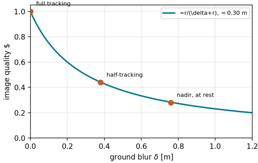
Figure 3: Normalised image quality q = r/(\delta + r) with r = 0.30 m. Annotated operating points match the nadir-at-rest, half-tracking, and full-tracking regimes above.
