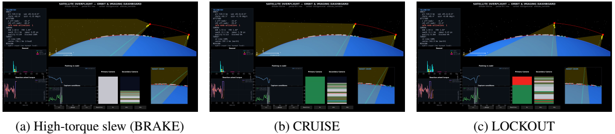
Figure 4: One attitude-safety cycle in torque-mode evaluation (same episode; panels use the recovery-phase names BRAKE / CRUISE / LOCKOUT). (a) High-torque slew: the agent commands large torque and reaches \approx 43^\circ off-nadir; safe mode activates (BRAKE) and rejects the request (applied torque drops while the agent request remains high). (b) CRUISE: onboard recovery slews the boresight back toward nadir (here \approx 24^\circ off-nadir) while agent torque stays ignored. (c) LOCKOUT: nadir hold with agent torque rejected for 60 s. SETTLE (between CRUISE and LOCKOUT) is short and not shown.
