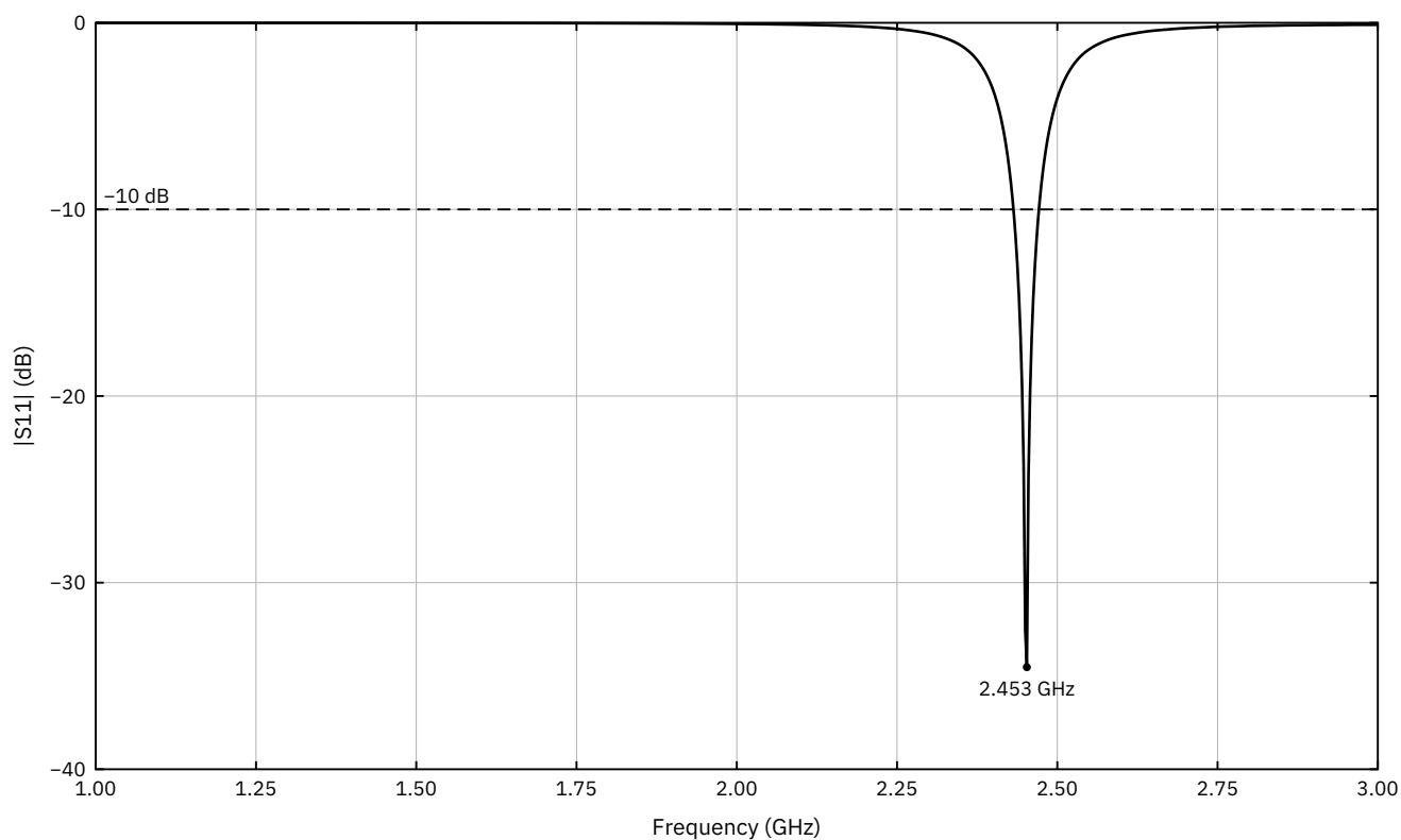
Figure 2. |S_{11}| versus frequency; the dashed line marks -10 dB and the dots the best-match frequencies.
