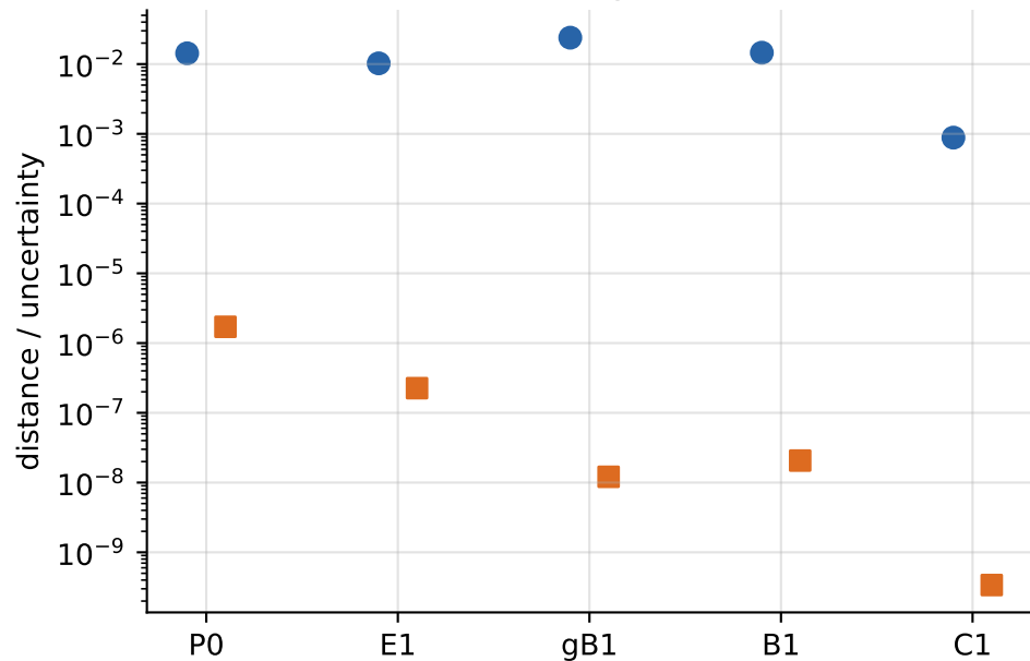
Metric density distance
