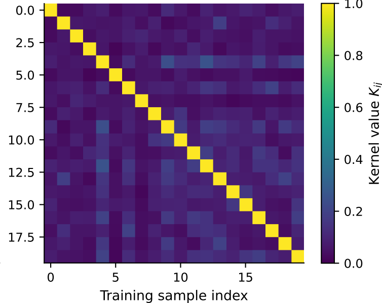
(c) IBM QPU K_{\text{train}}
