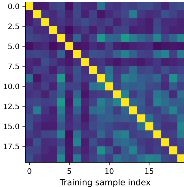
(a) Ideal K_{\text{train}}
