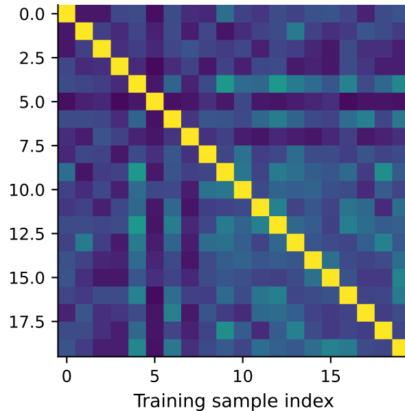
(b) Finite-shot K_{\text{train}}
