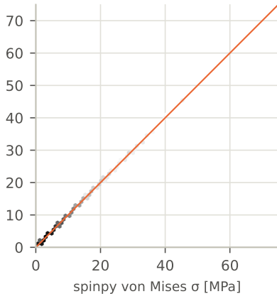
Spinodoid · \max |\Delta|/\max = 3\text{e-}08
