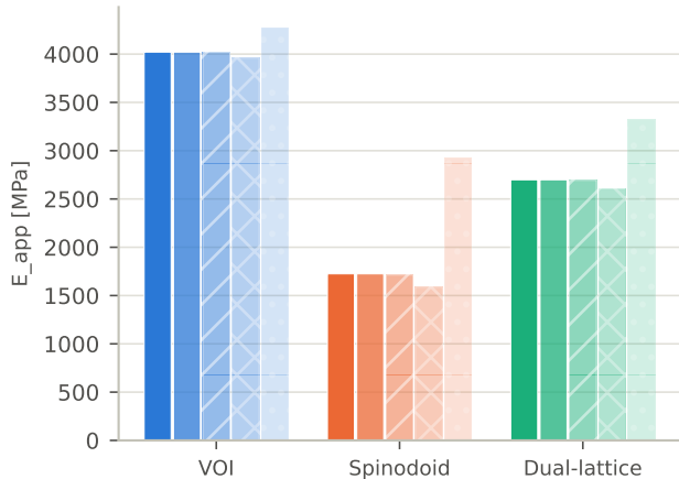
App test ( 40^3 , sliding, 20 GPa, 1 MPa)
