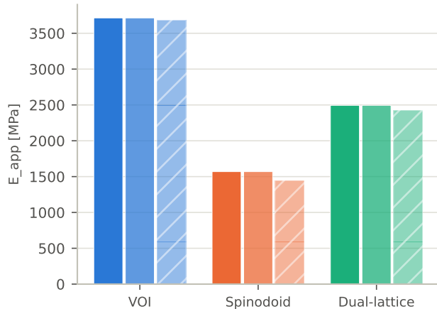
Tapia et al. protocol ( 40^3 , fixed, 18 GPa, 100 N)
