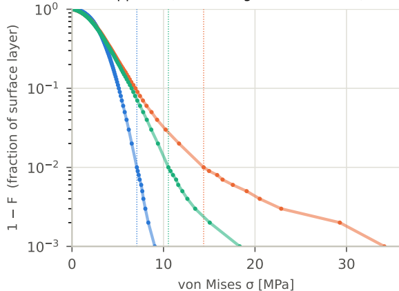
App test ( 40^3 , sliding, 20 GPa, 1 MPa)
