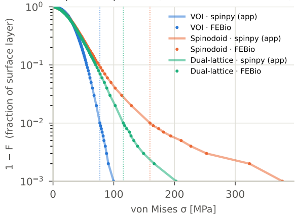
Tapia et al. protocol ( 40^3 , fixed, 18 GPa, 100 N)
