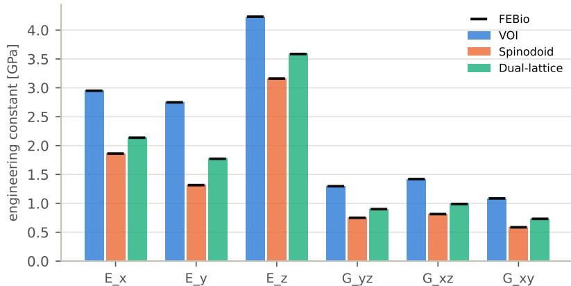
Periodic tensor ( 32^3 )
