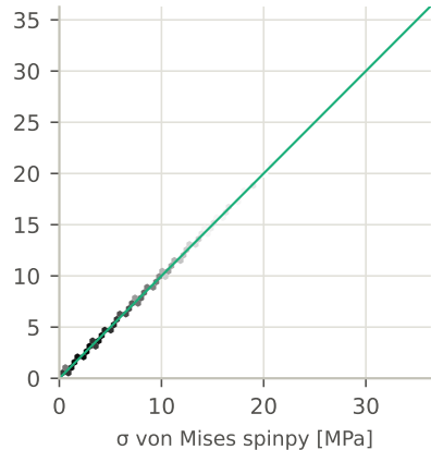
Dual-lattice · \max |\Delta|/\max = 3\text{e-}08
