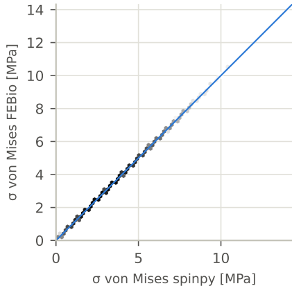
VOI · \max |\Delta|/\max = 7\text{e-}08
