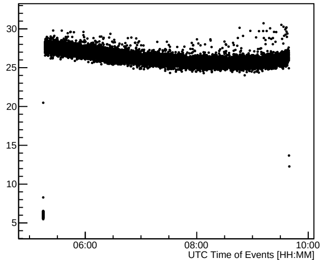
Average Pedestal RMS [ADC Counts]
