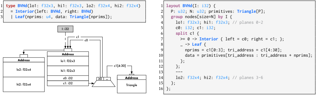
Fig. 12. BVH with DOP-14 bounding volumes [46] specified in Scion.
