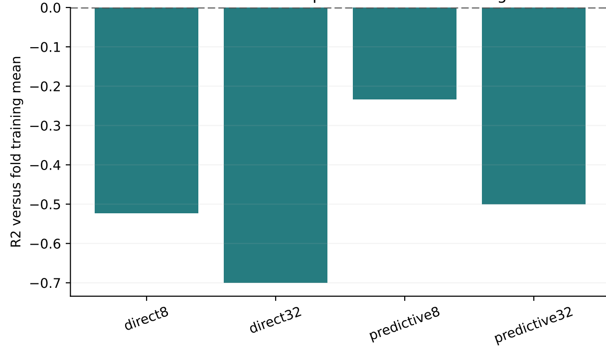
Absolute future CT1: improvement over training mean
