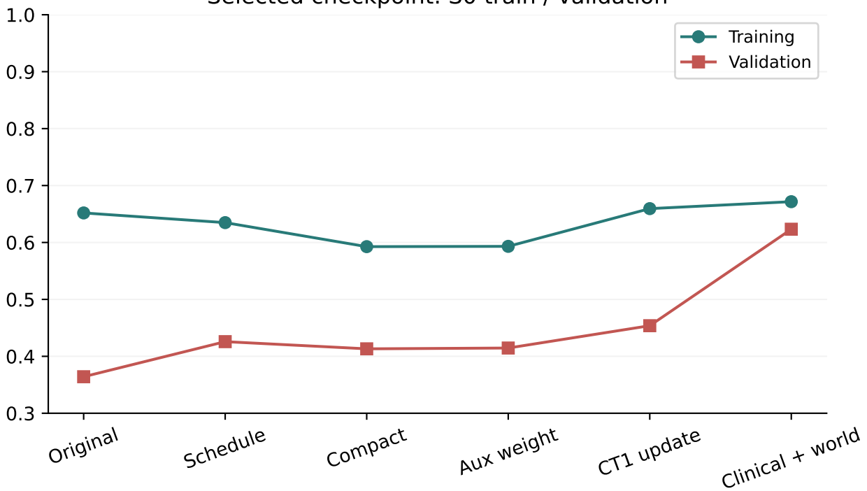
Selected checkpoint: S0 train / validation
