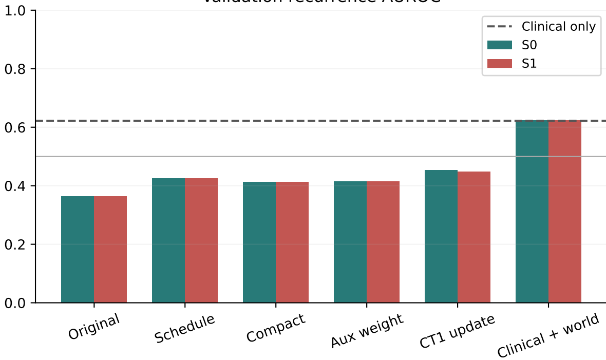
Selected checkpoint: S0 train / validation
