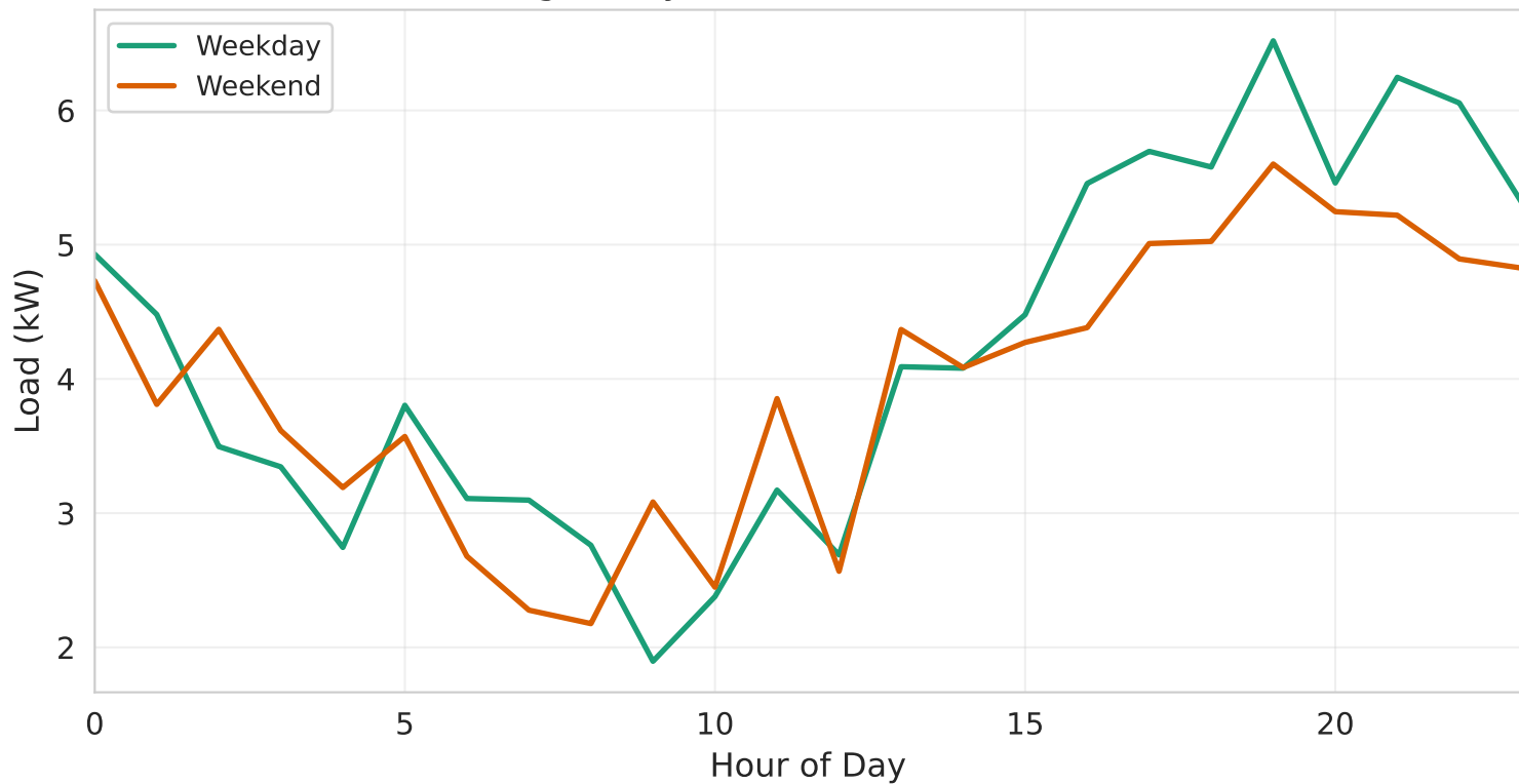
Average Daily Load Profile – Site S1 Bihar
