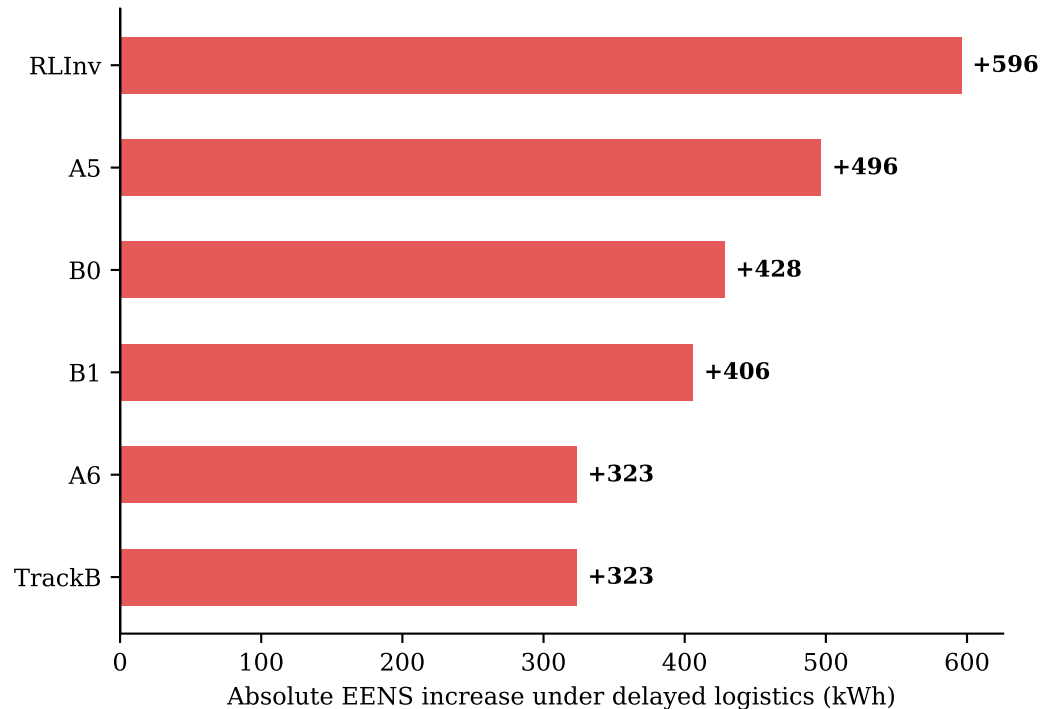
Policy Sensitivity to Logistics Delay (absolute EENS increase; lower = more robust)
