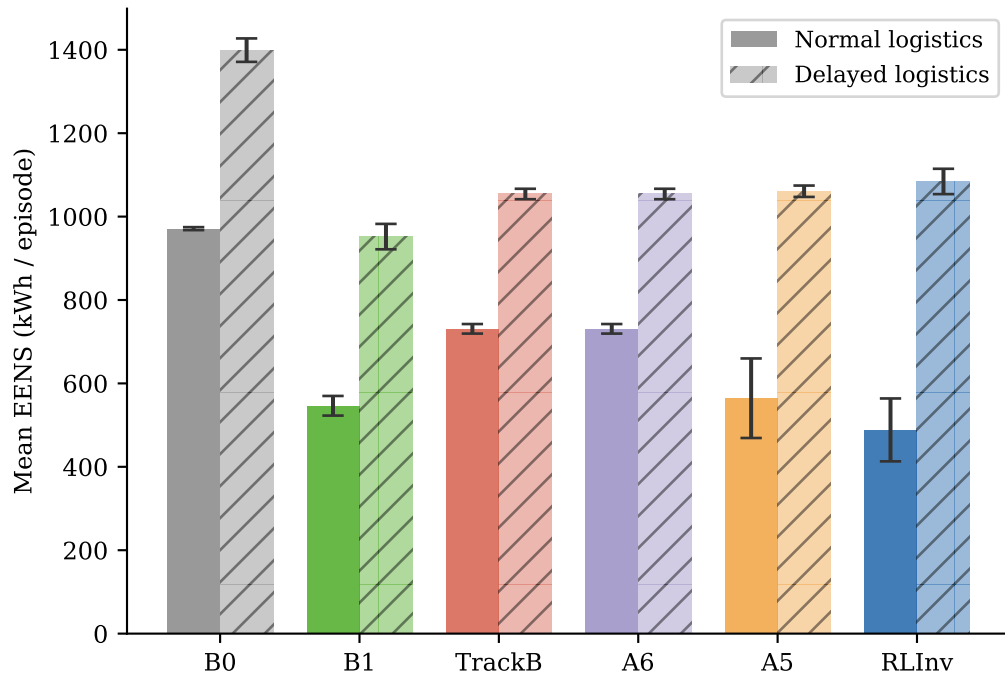
Normal vs Delayed Logistics (constrained sites, n = 3 seeds)
