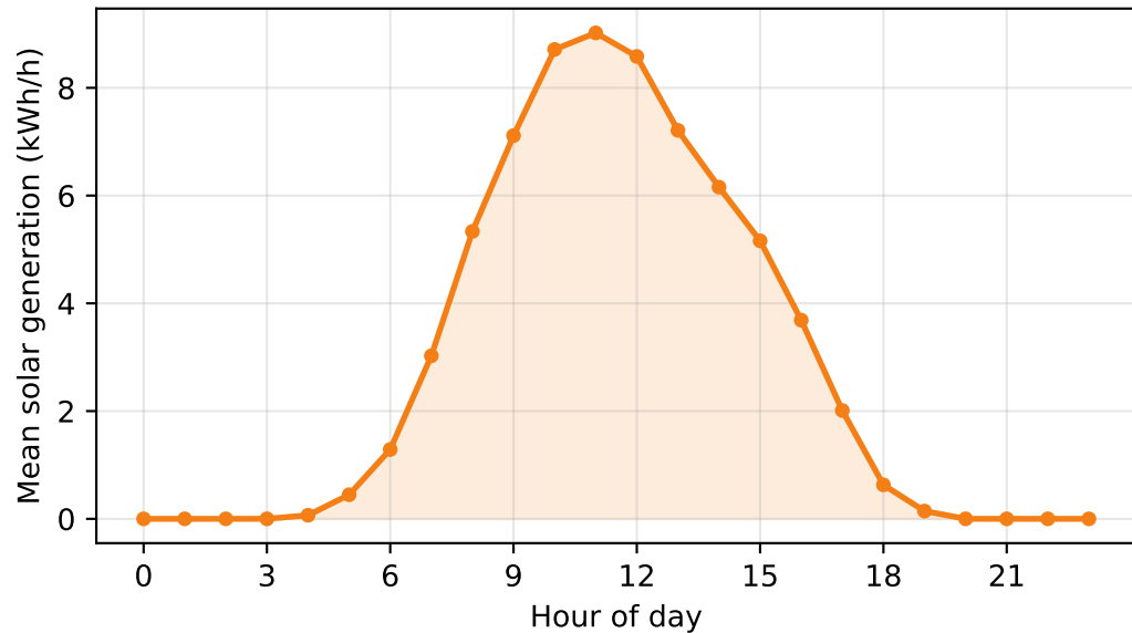
Solar generation
