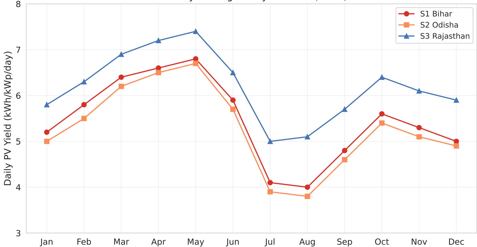
Monthly Average Daily PV Yield (2023)
