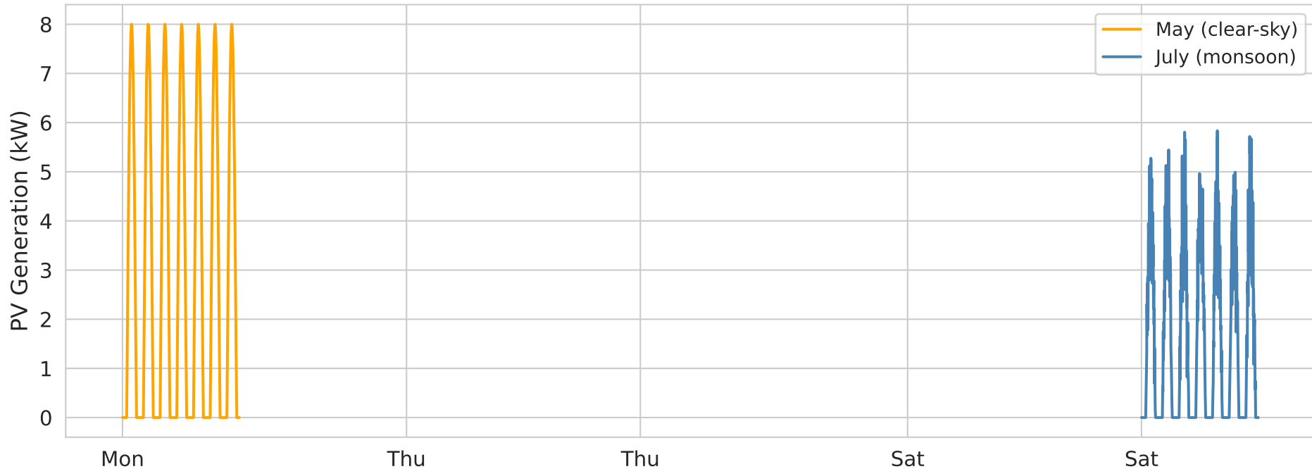
One-Week PV Generation Trace - Site S1 Bihar
