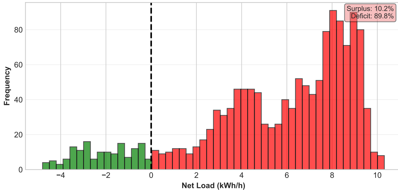
Net Load Distribution
