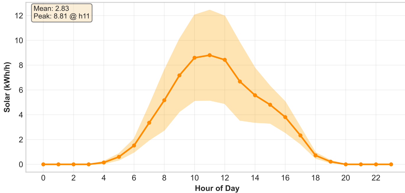
Solar Profile (Mean ± Std)
