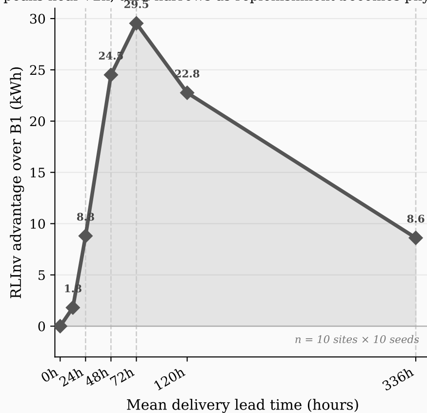
(b) RLInv Advantage over B1 as Delivery Delay Increases Advantage peaks near 72h, then narrows as replenishment becomes physically constrained
