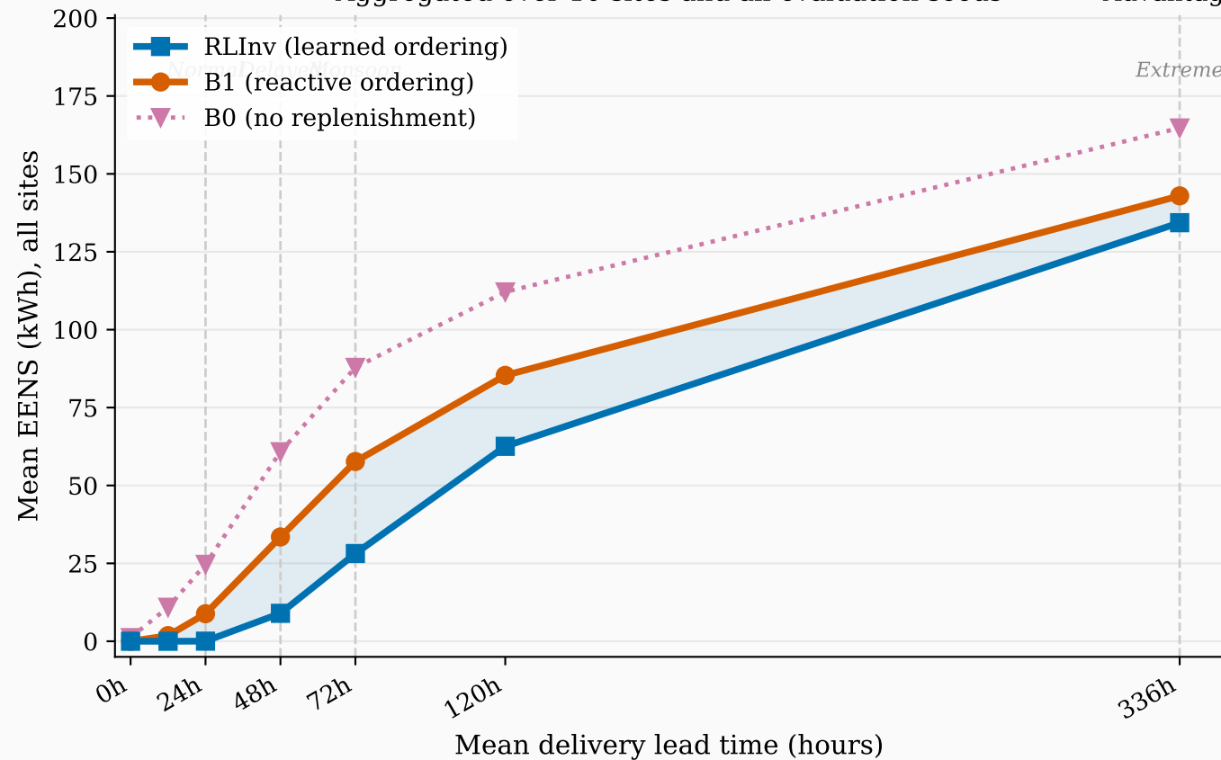
(a) Policy Performance under Increasing Delivery Delays Aggregated over 10 sites and all evaluation seeds
