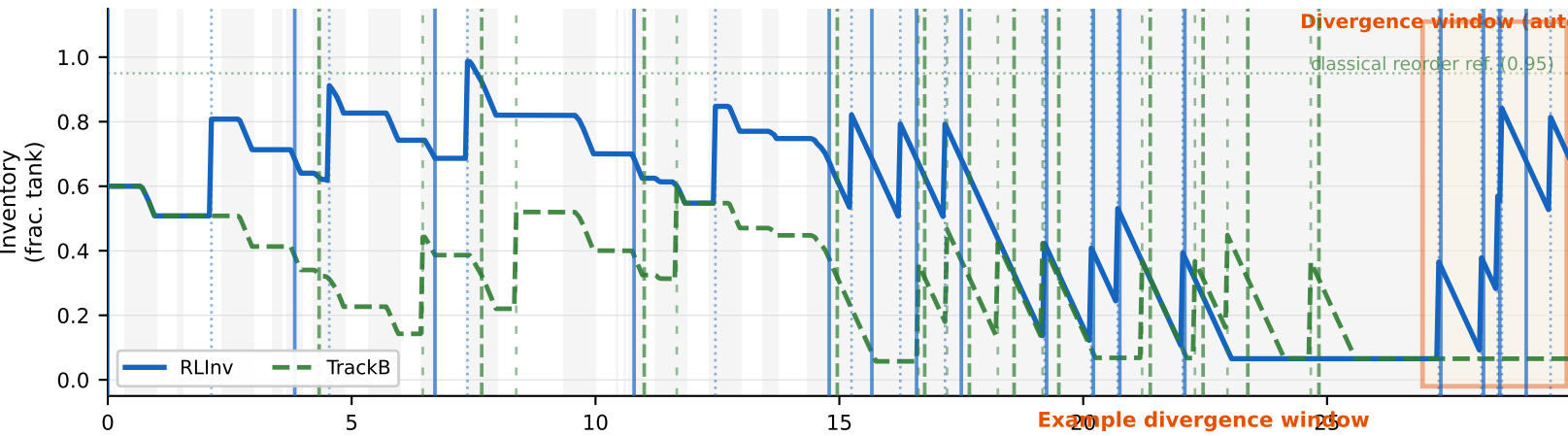
Normal logistics (mean lead = 24 h) ① Diesel Inventory (solid=order · dotted=arrival)
