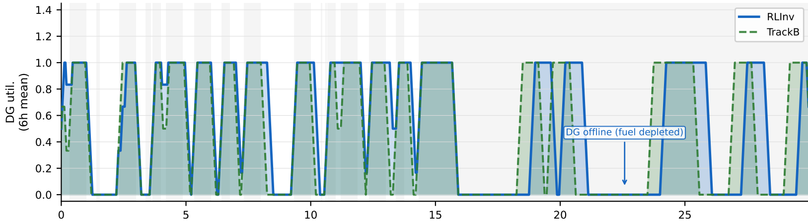
③ Diesel Generator Usage
