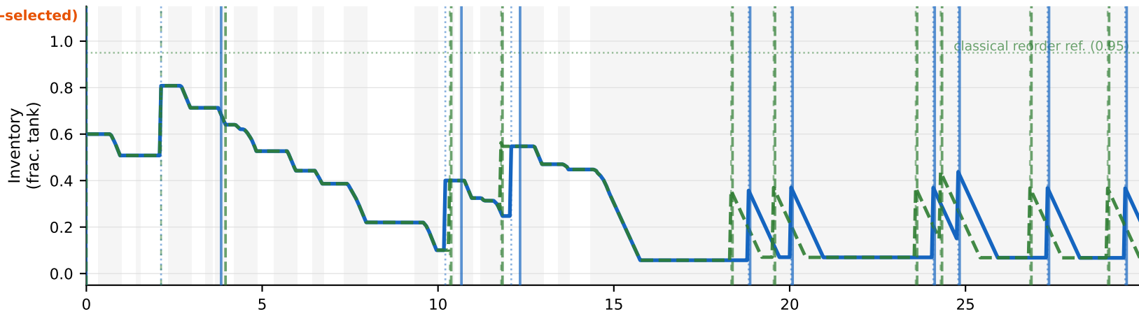
Delayed logistics (mean lead = 48 h) — robustness check ① Diesel Inventory (solid=order · dotted=arrival)
