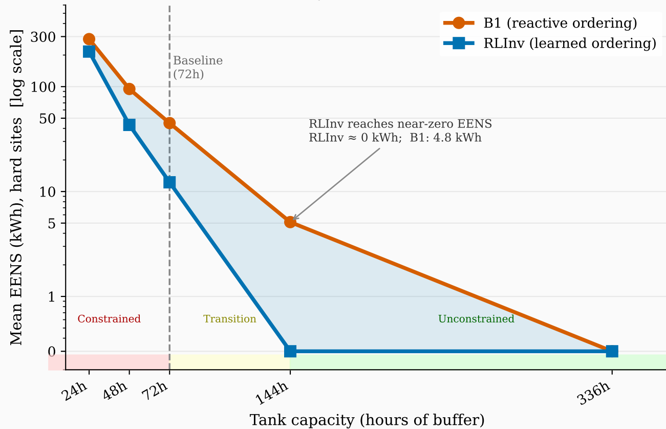
(a) EENS by Policy vs Tank Capacity Scenario: Delayed (mean lead time = 48h)
