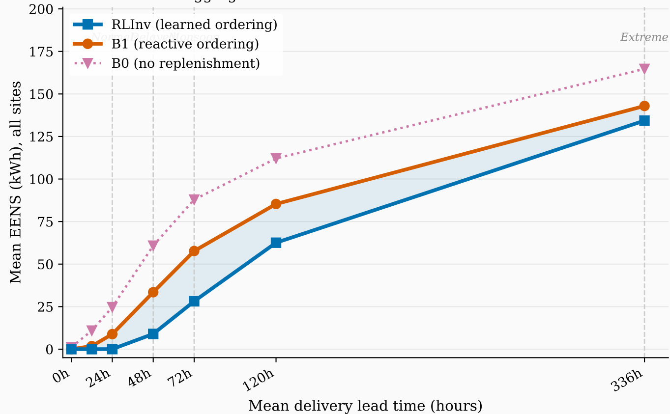
(a) EENS vs Mean Delivery Lead Time Aggregated over 10 sites and all evaluation seeds
