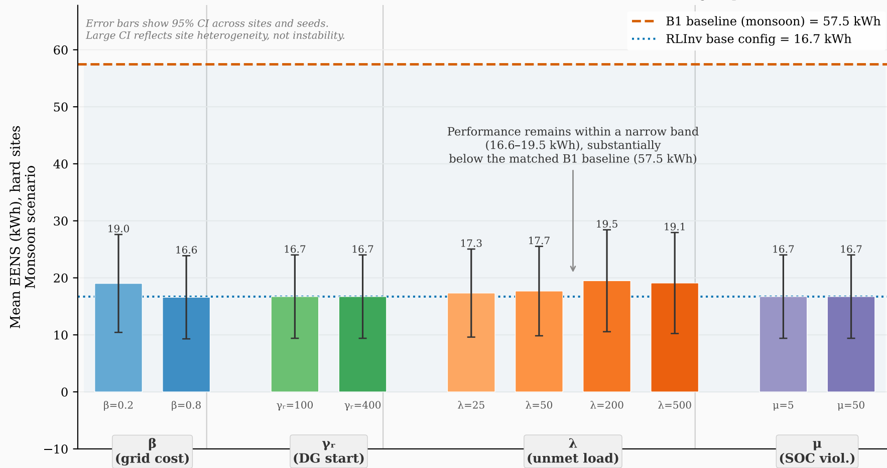
(a) Reward Weight Robustness — Monsoon Scenario All variants evaluated on hard sites (site2/5/7), 3 seeds \times 400k training steps
