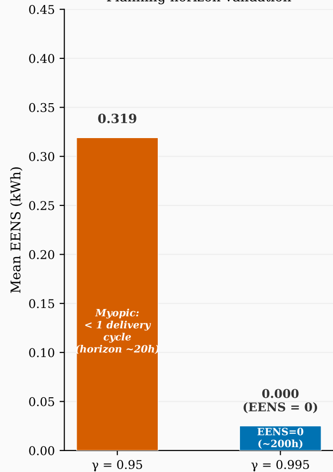
(b) Discount Factor \gamma Planning horizon validation
