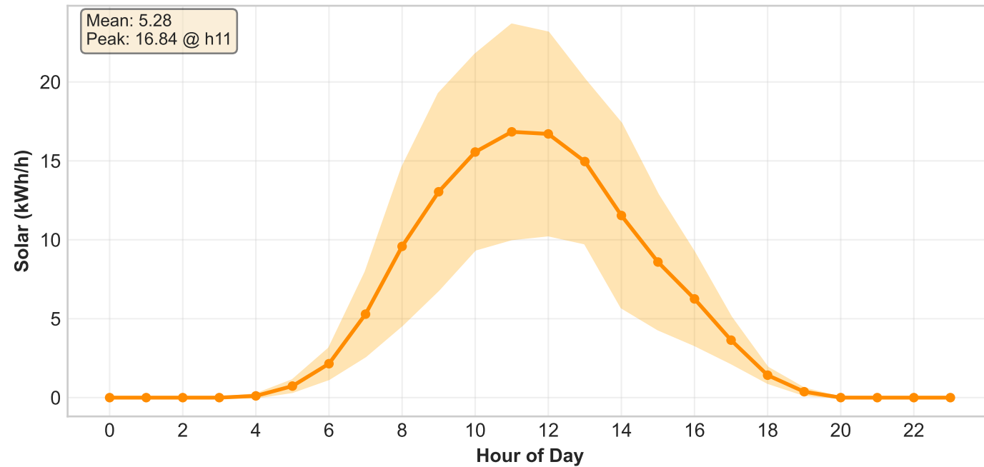
Solar Profile (Mean ± Std)
