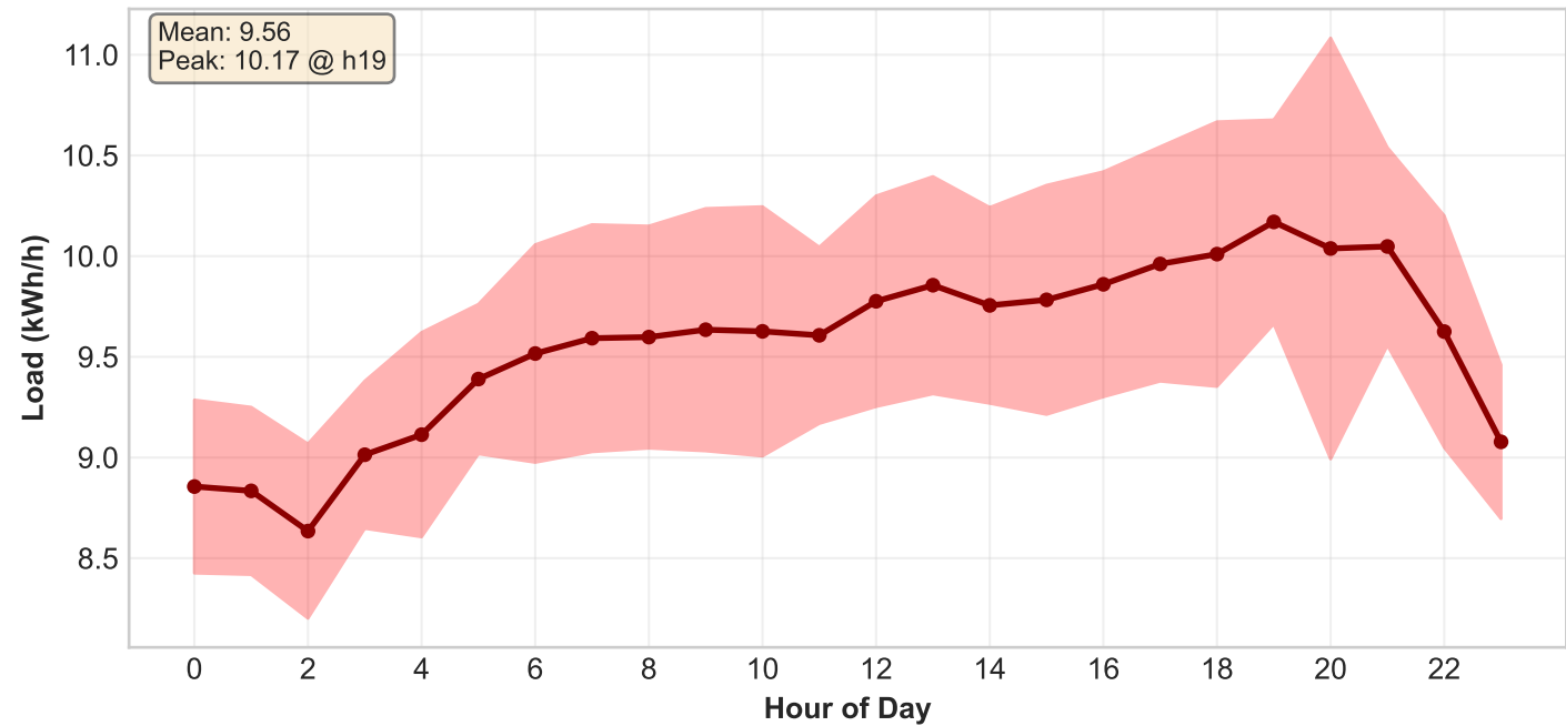
Load Profile (Mean ± Std)
