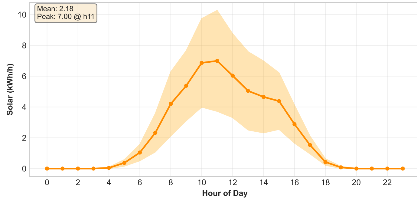
Solar Profile (Mean \pm Std)
