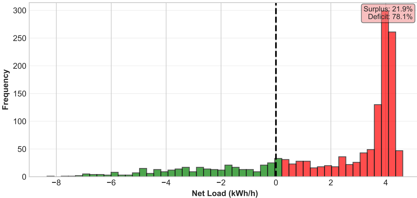
Net Load Distribution
