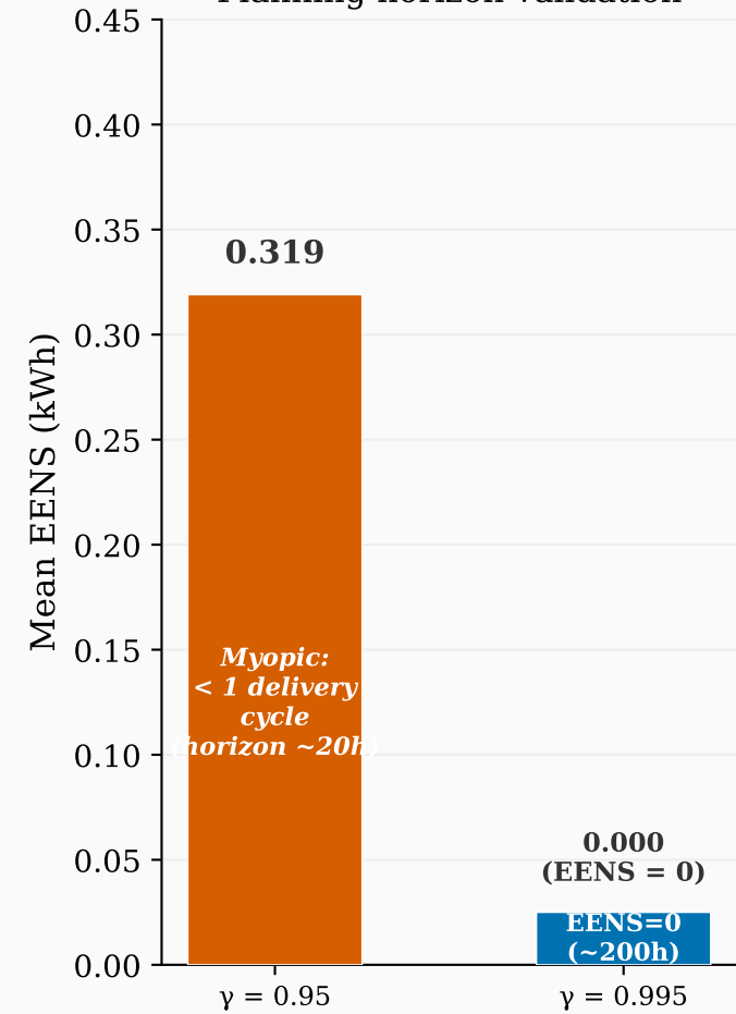
(b) Discount Factor \gamma Planning horizon validation
