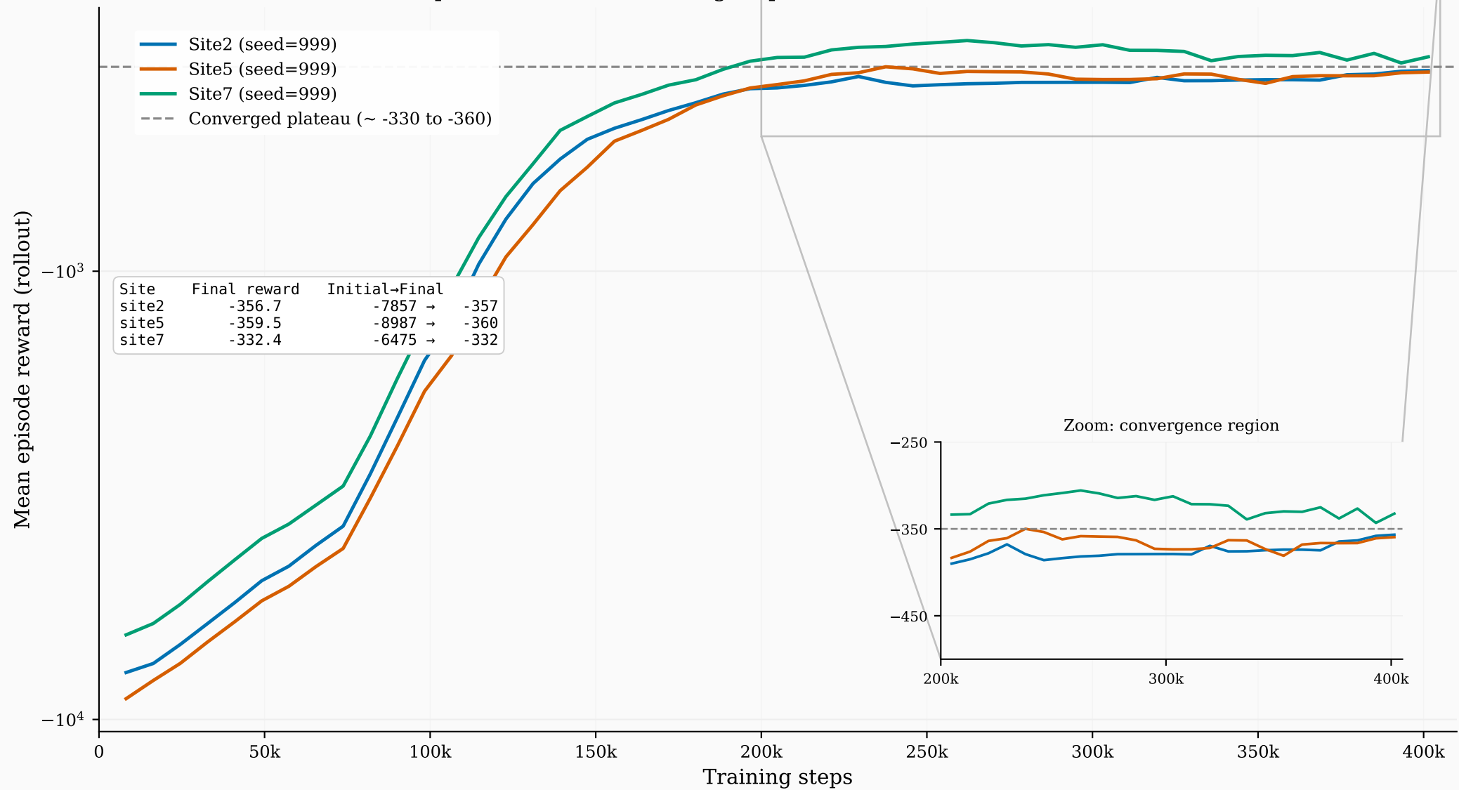
RLInv Training Dynamics under the Normal Training Scenario Mean episode reward vs training steps across three hard sites, seed = 999
