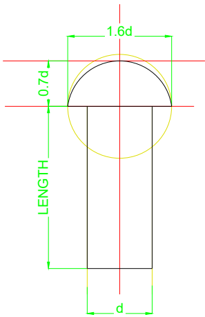
SNAP HEAD
