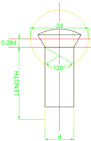
CONTERSUNK HEAD
