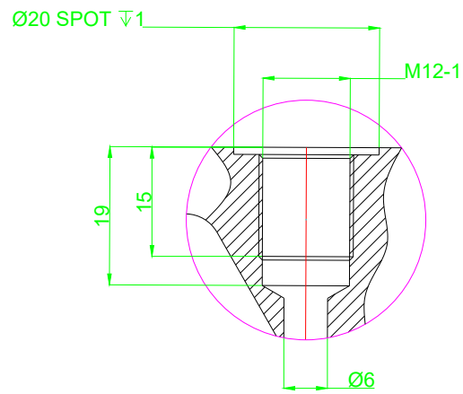
DETAIL VIEW- A SCALE 1:1
