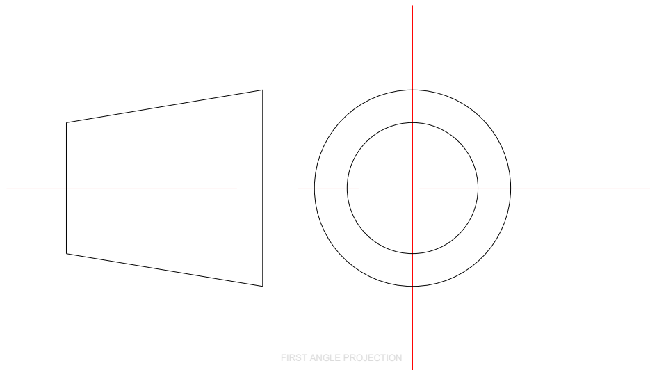
FIRST ANGLE PROJECTION
