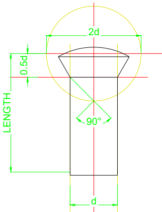
FLAT COUNTERSUNK HEAD 90°
