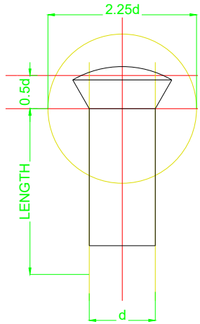
MUSHROOM HEAD
