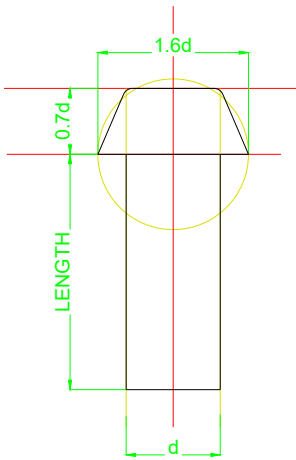
PAN HEAD
