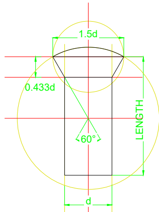
ROUND COUNTERSUNK HEAD 60°
