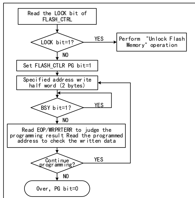
Figure 46-1 FLASH program
