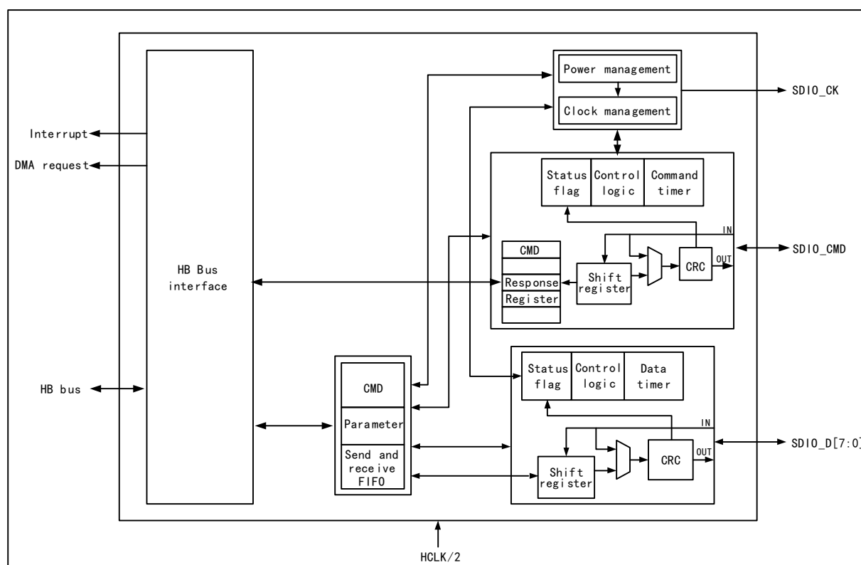
Figure 32-1 SDIO structure diagram
