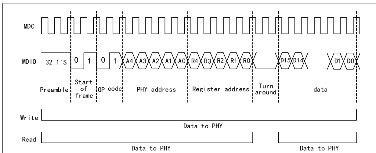
Figure 31-3 SMI interface read and write time diagram
