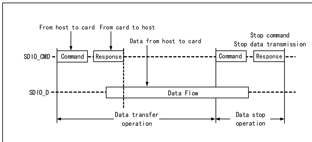
Figure 32-8 SDIO data stream write timing (Taking SDIO card as an example)
