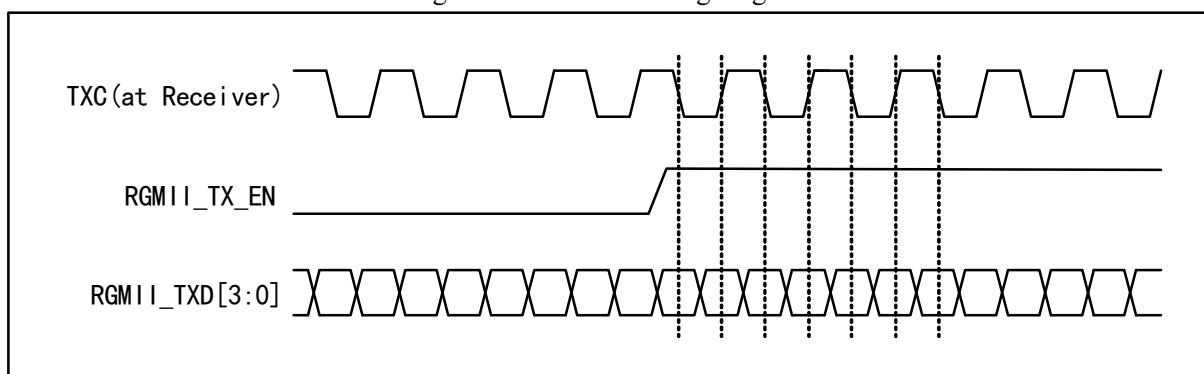
Figure 31-4 RGMII timing diagram
