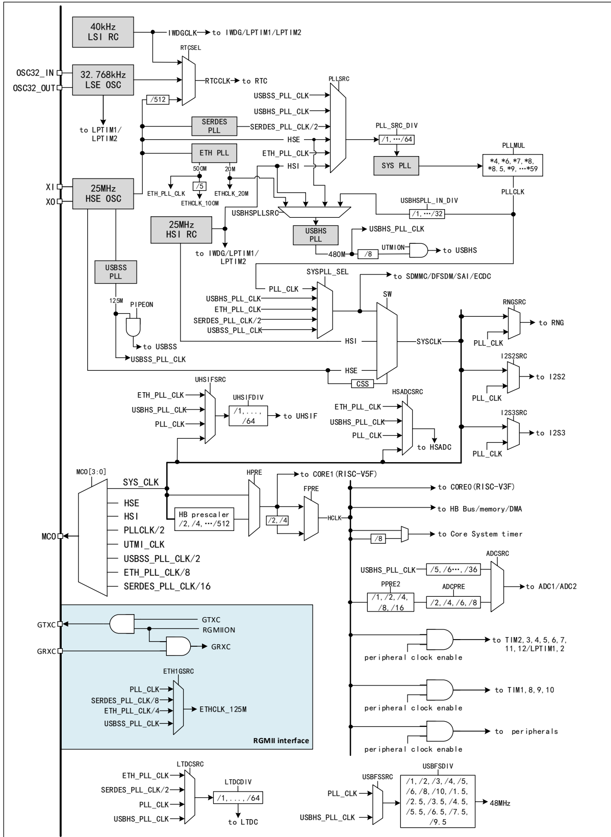
Figure 3-2 Clock tree block diagram
