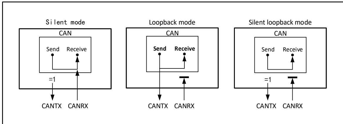
Figure 28-2 CAN 3 test modes of the bus
