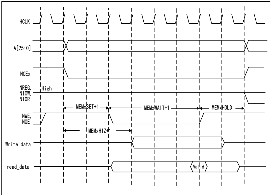
Figure 40-21 General memory access waveform of NAND Flash controller
