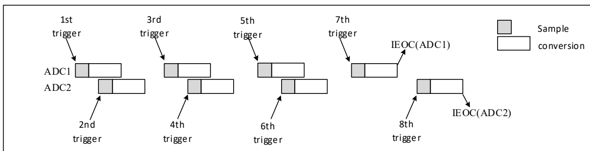
Figure 11-11 Alternating trigger conversions for each ADC injection channel in discontinuous mode
