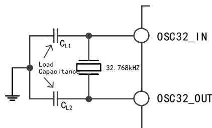
Figure 3-5 Low-speed external crystal circuit
