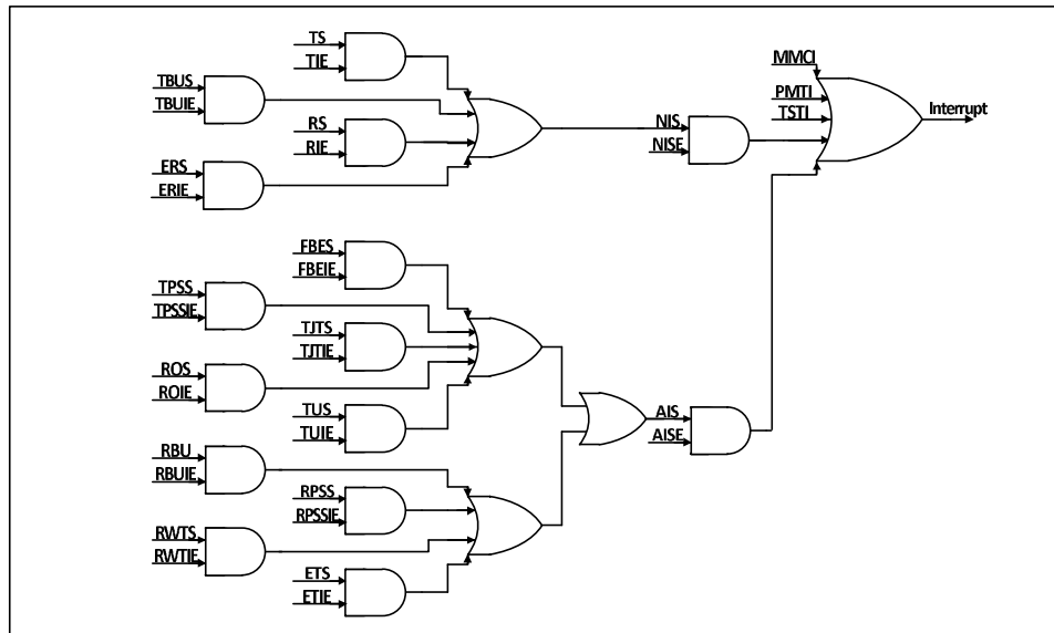
Figure 31-11 Interrupt schematic
