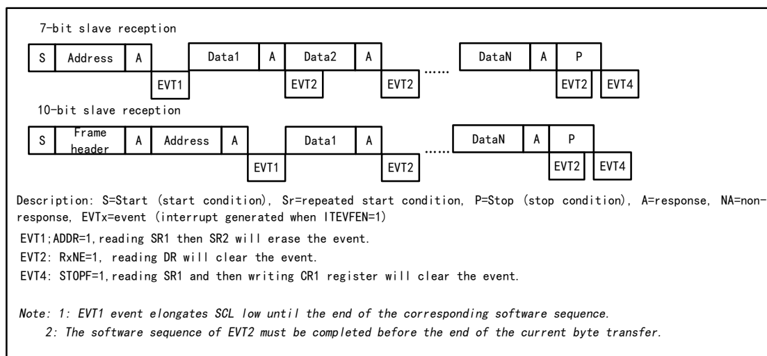
Figure 21-7 Receiver transmission sequence diagram
