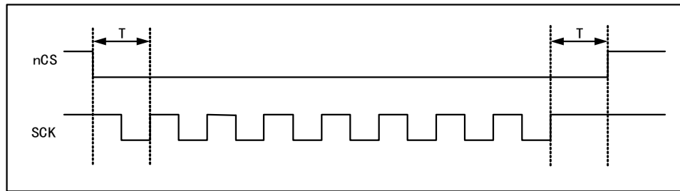
Figure 37-5 nCS with CKMODE = 1 ( T = \text{SCK period} )
