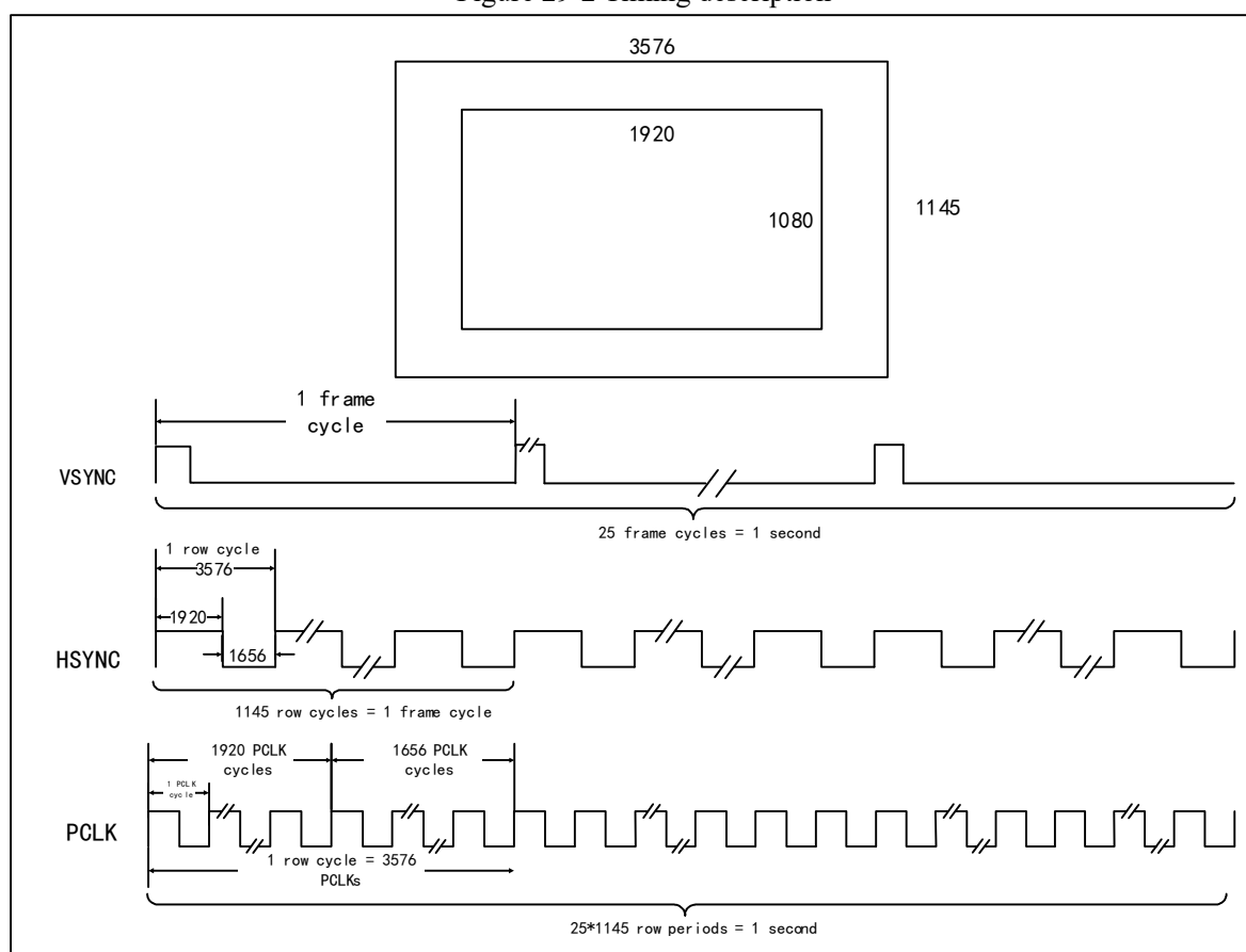
Figure 29-2 Timing description
