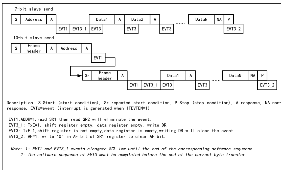
Figure 21-6 Slave transmitter transmission sequence diagram
