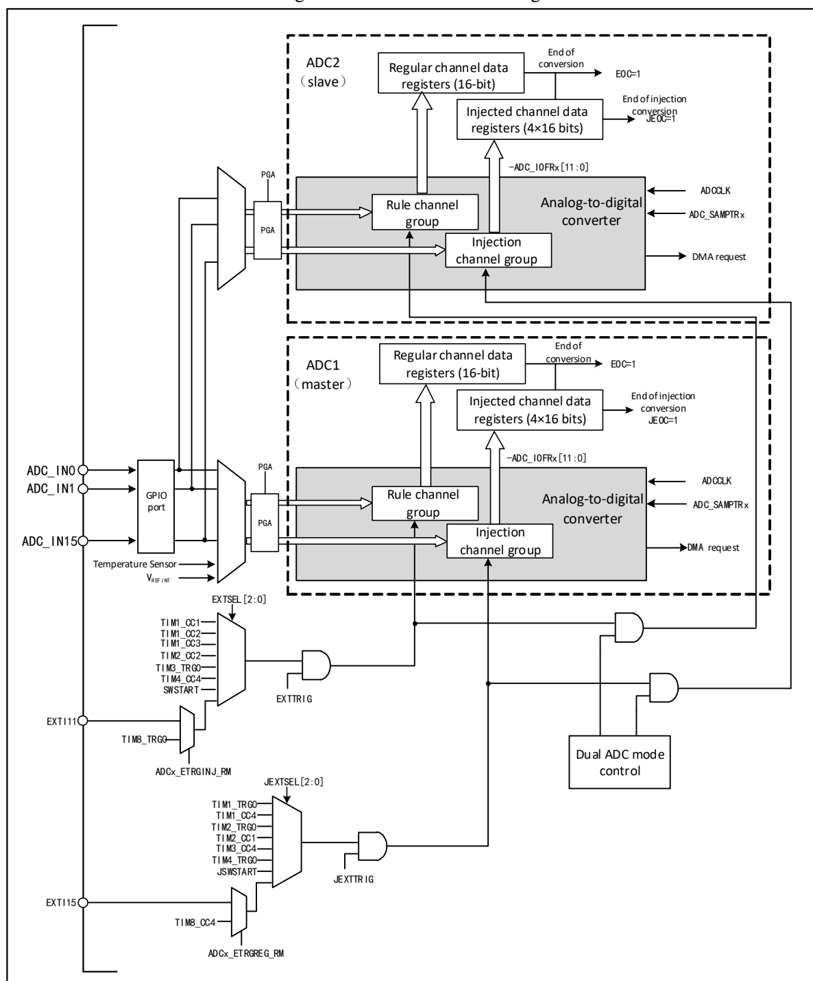
Figure 11-5 Dual ADC block diagram
