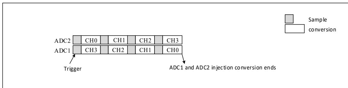
Figure 11-6 Channel synchronous injection conversion
