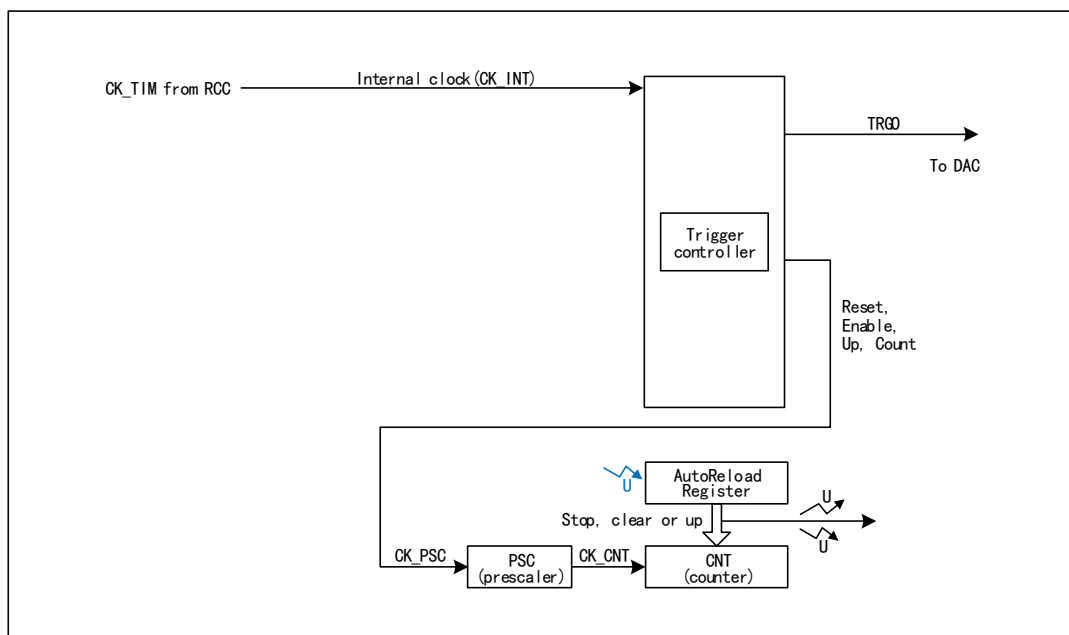
Figure 16-1 Block diagram of the structure of the basic timer
