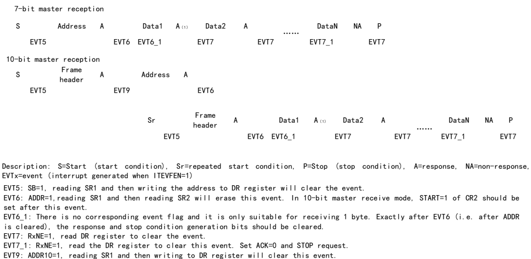
Figure 21-5 Receiver transmission sequence diagram
