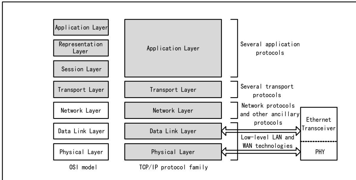
Figure 31-1 Position of Ethernet Transceivers in OSI Model and TCP/IP Model
