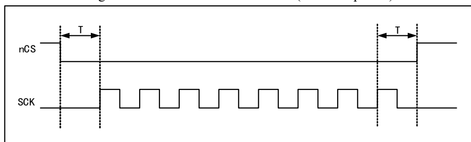
Figure 37-4 nCS with CKMODE = 0 (T = SCK period)
