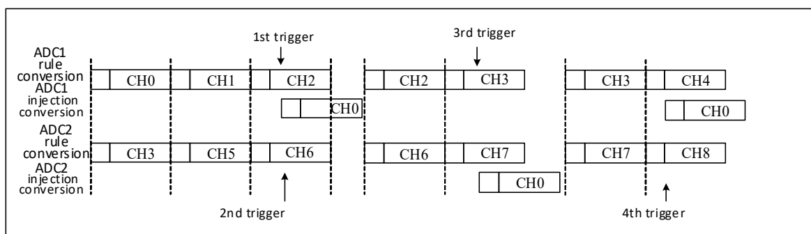
Figure 11-13 Trigger event occurs during injection conversion
