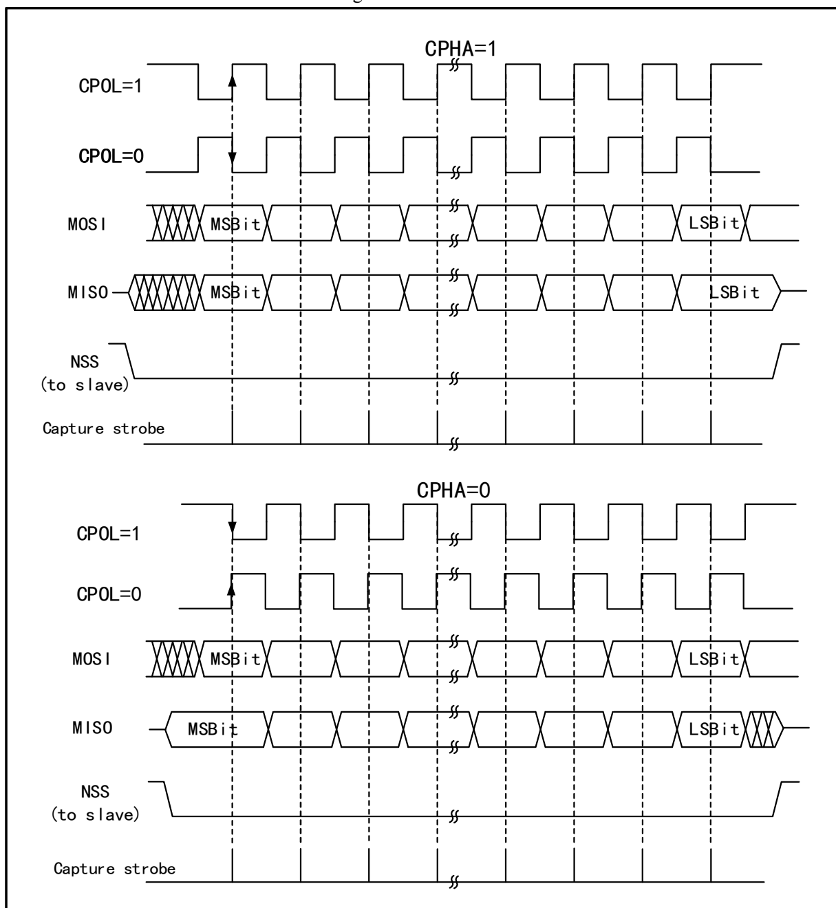
Figure 23-2 SPI model
