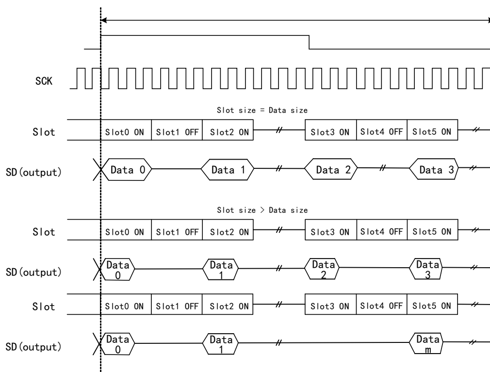
Figure 36-14 Three-State strategy on output data line with I2S and other protocols
