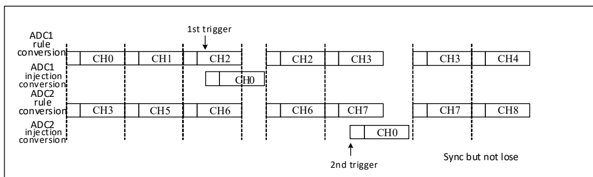
Figure 11-12 Alternating trigger injection channel switching in synchronous regular mode
