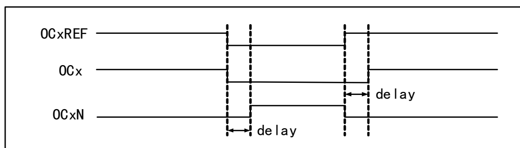
Figure 14-4 Complementary output and deadband
