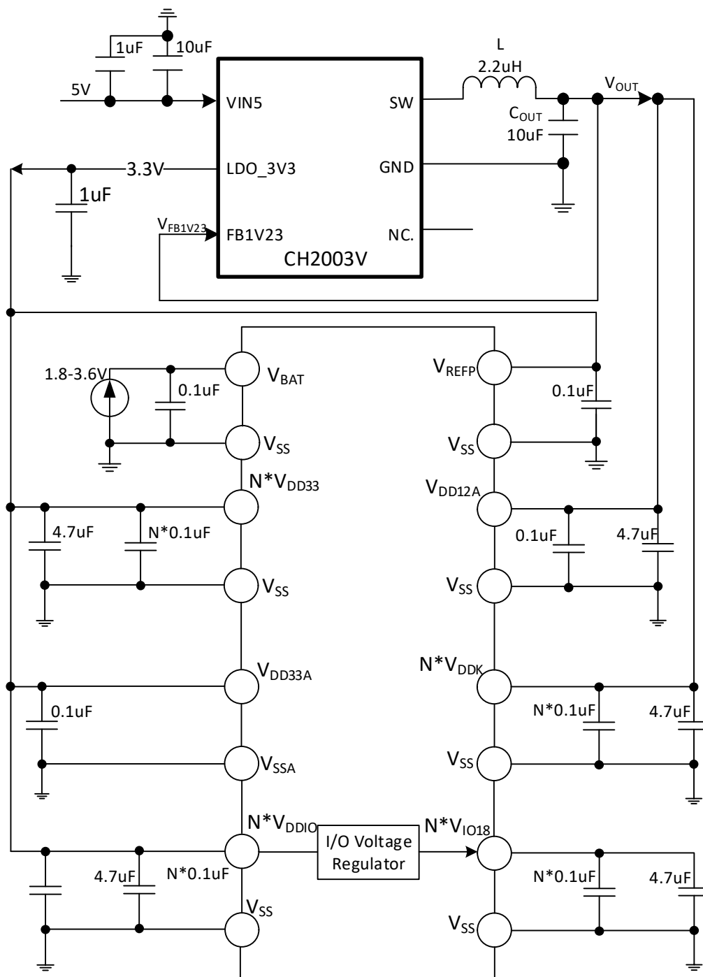
Figure 3-1-2 CH32H417 DCDC single 5V supply circuit
