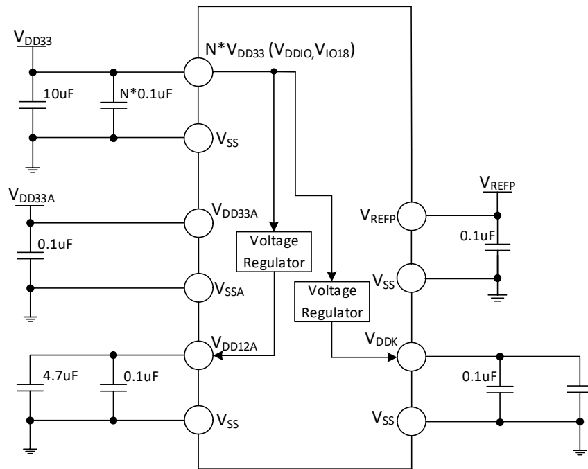
Figure 3-1-3 CH32H416 Conventional power supply typical circuit
