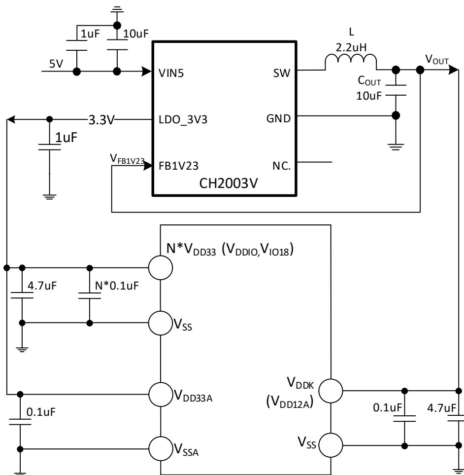
Figure 3-1-6 CH32H415 DCDC single 5V supply circuit
