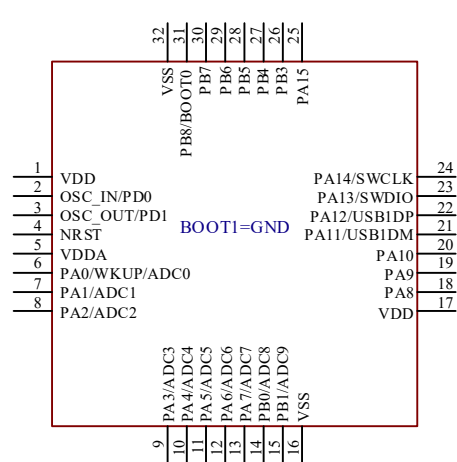
CH32V203K8T6
