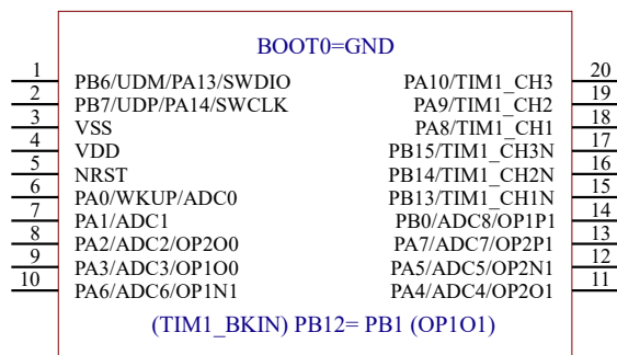
CH32V203F8P6
