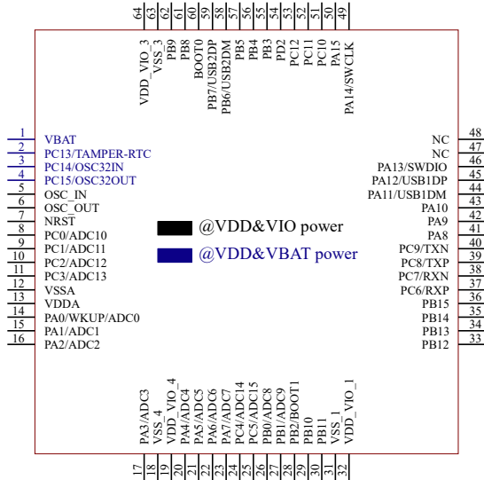
CH32V203RBT6
