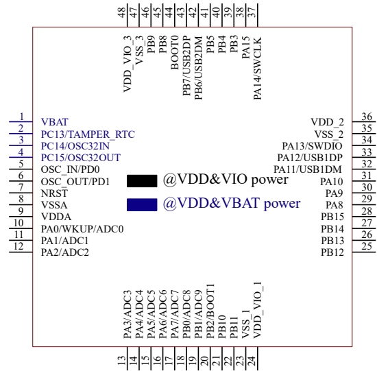
CH32V203CxT6
