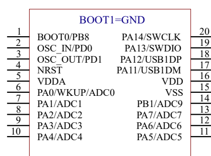
CH32V203F6P6
