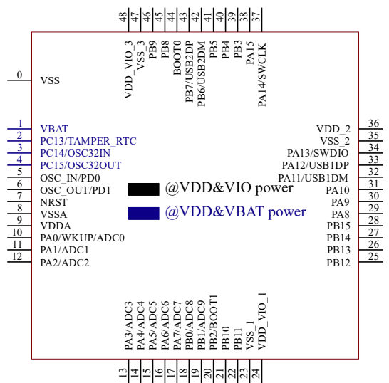
CH32V203CxU6
