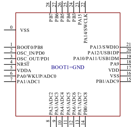
CH32V203G6U6
