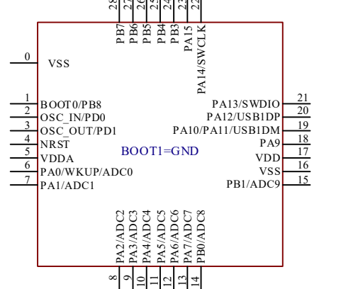
CH32V203G6U6
