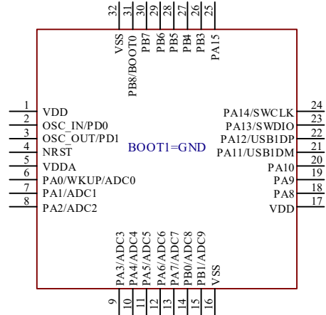
CH32V203K8T6
