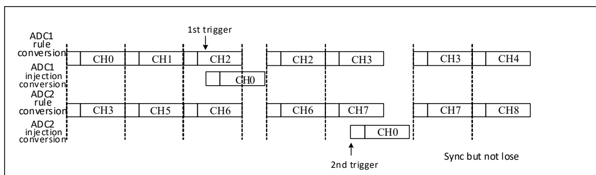
Figure 12-12 Alternating trigger injection channel switching in synchronous regular mode
