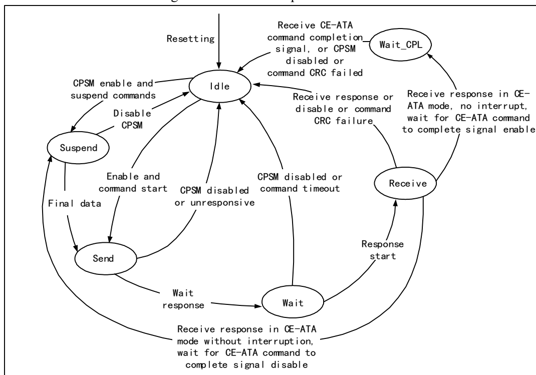
Figure 24-2 Command path state machine
