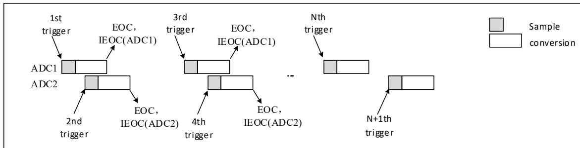
Figure 12-10 Alternate trigger conversion for each ADC injection channel group
