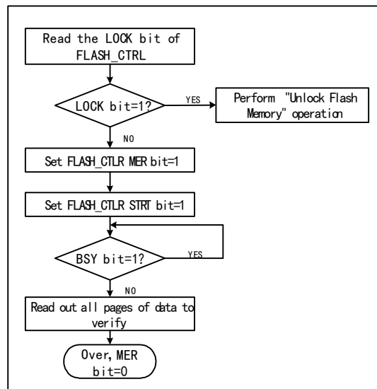
Figure 32-3 FLASH full chip erasure
