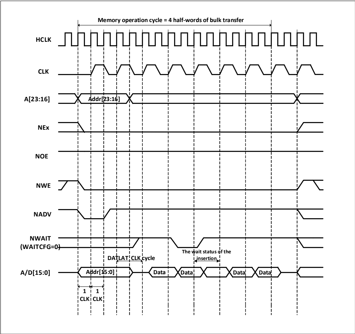
Figure 26-14 Synchronous bus multiplexing write operations (Multiplexed)
