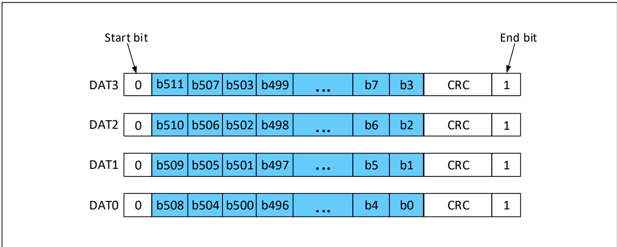
Figure 24-12 SD card 4 bus data transfer in a 512-bit word format
