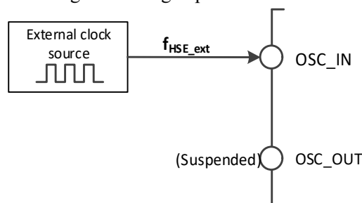
Figure 3-4 High-speed clock source circuit
