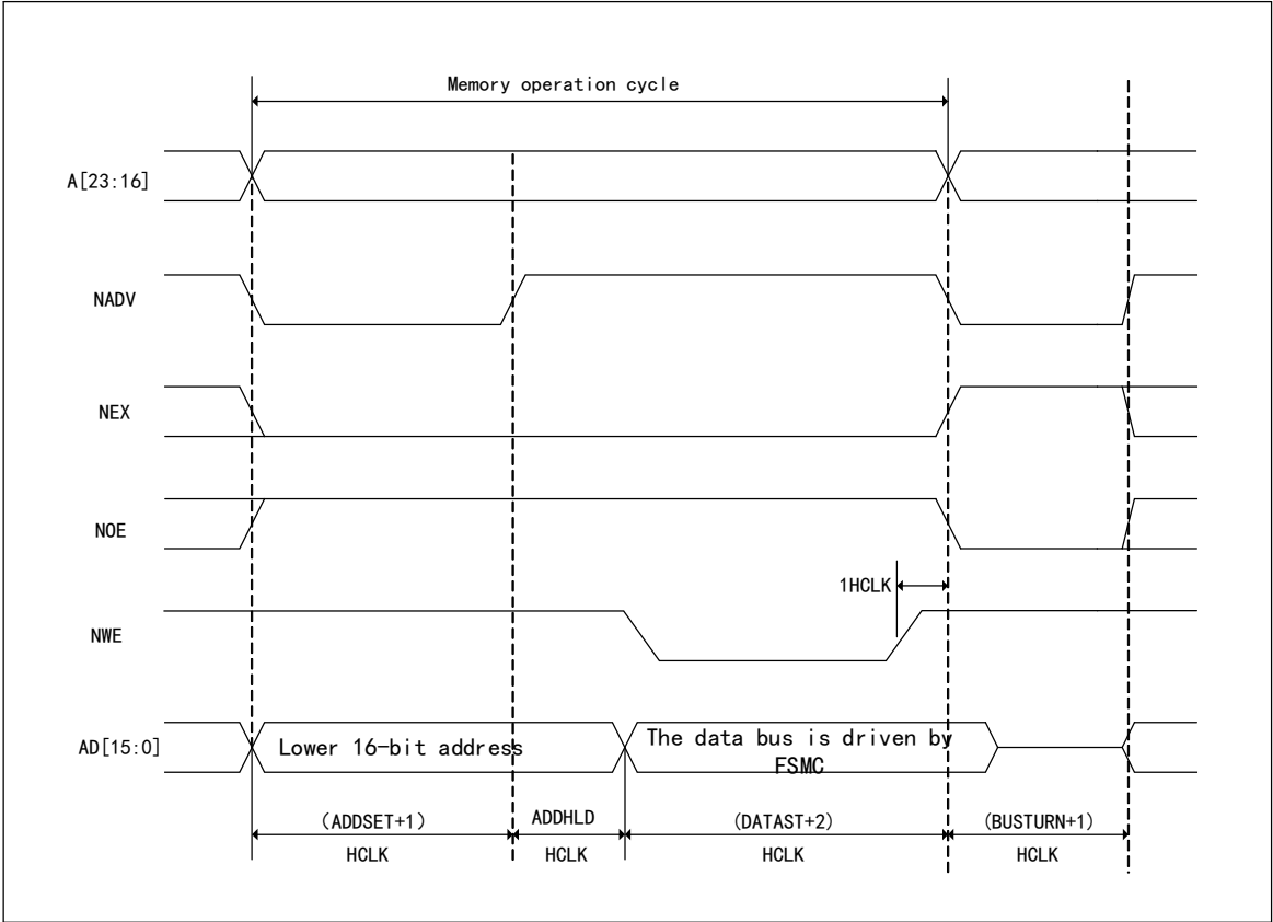
Figure 26-12 Mode D write operation (Multiplexed)
