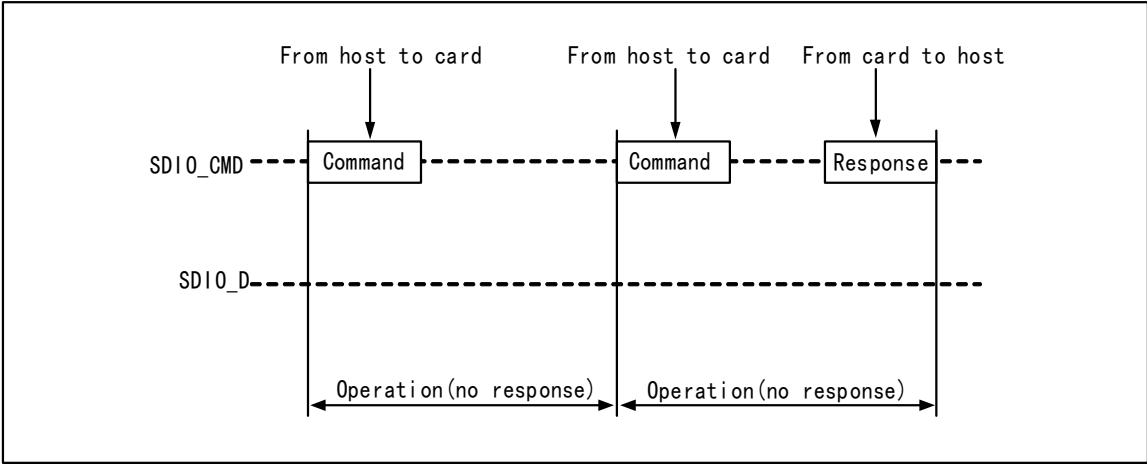
Figure 24-4 SDIO no response timing and no data timing (Taking SD card as an example)
