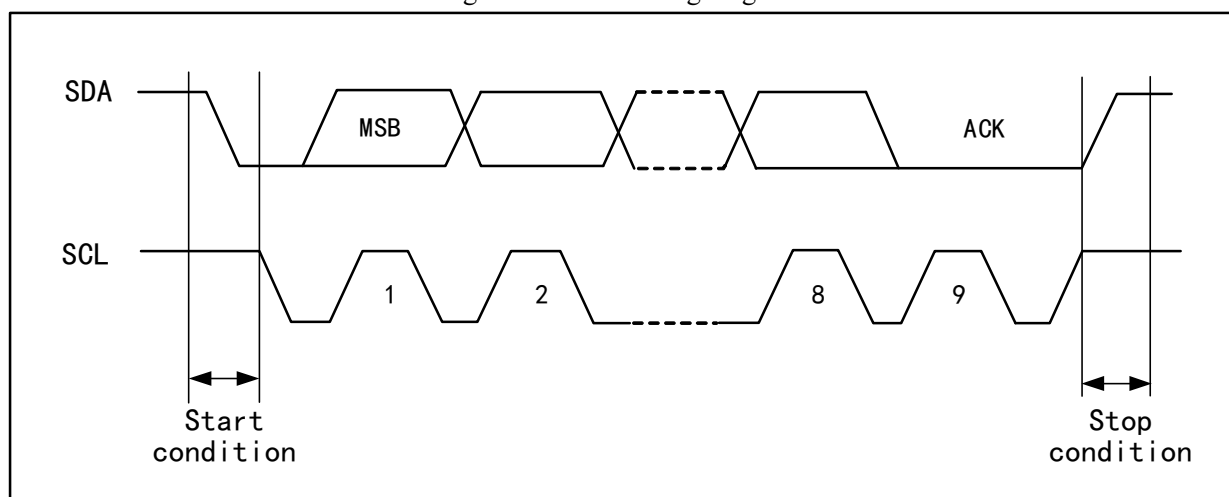
Figure 18-1 I2C timing diagram
