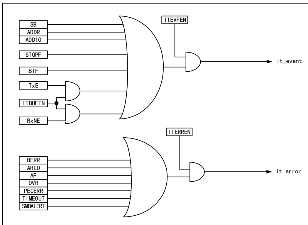
Figure 18-4 I2C interrupt request
