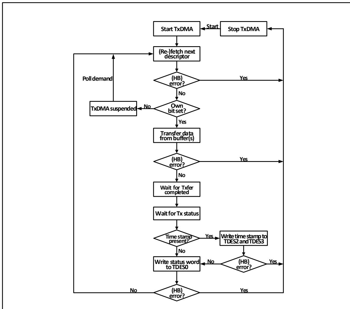
Figure 29-4 Process of transmission
