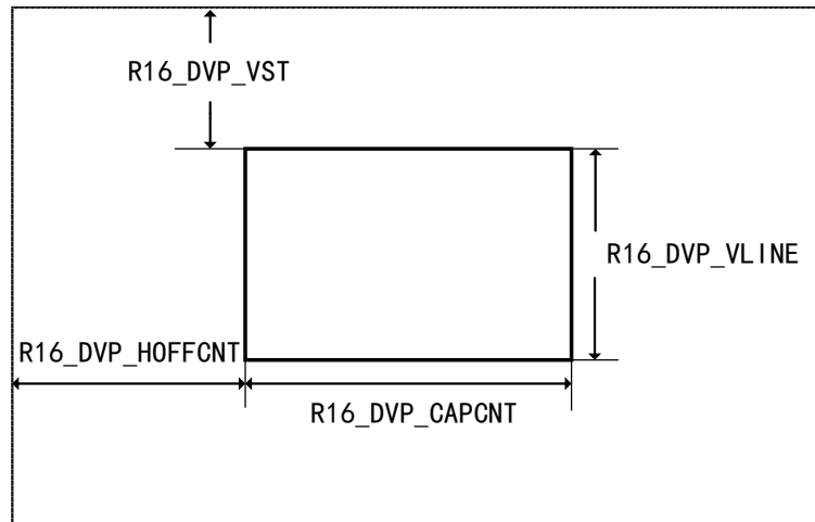
Figure 23-5 Crop window coordinates and size
