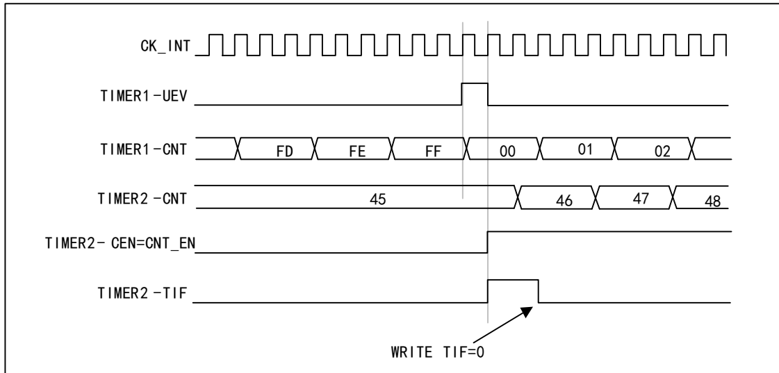
Figure 14-13 Using the update event of timer 1 to trigger timer 2
