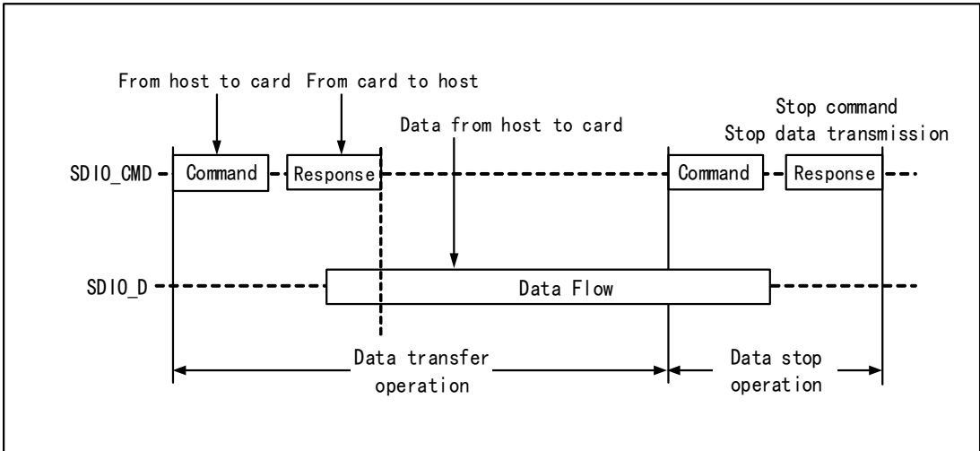
Figure 24-8 SDIO data stream write timing (Taking SDIO card as an example)
