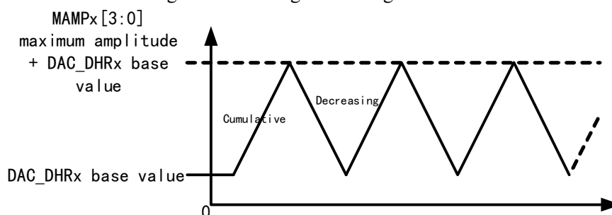
Figure 13-4 Triangular wave generation
