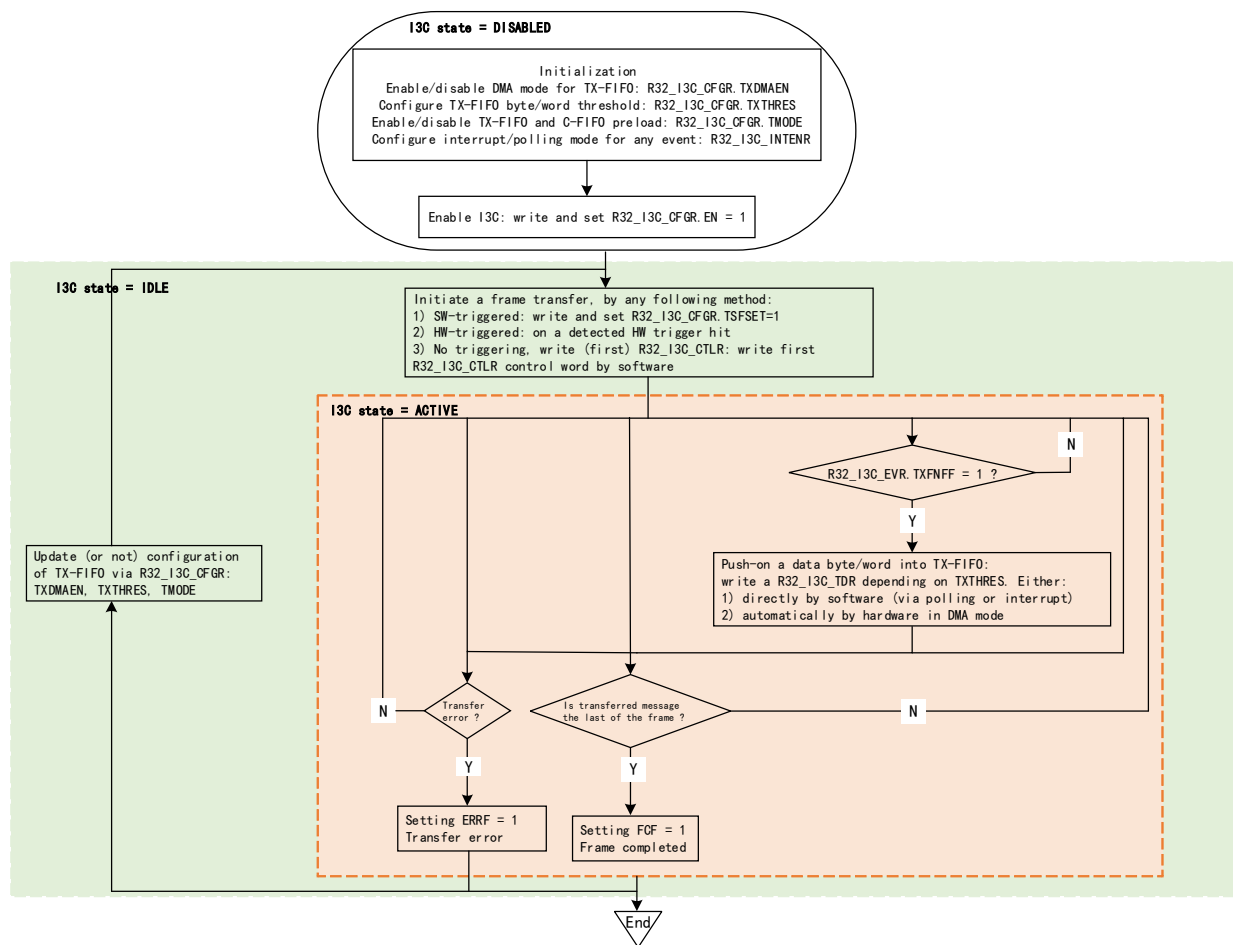
Figure 19-10 TX-FIFO management (as master)
