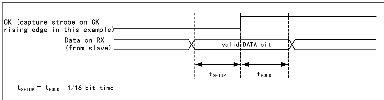
Figure 17-3 Data sample hold time
