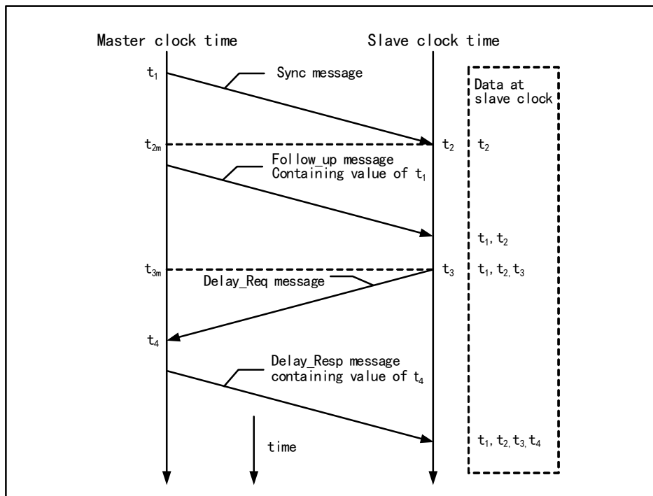
Figure 29-1 IEEE1588 PTP protocol synchronization message timing diagram
