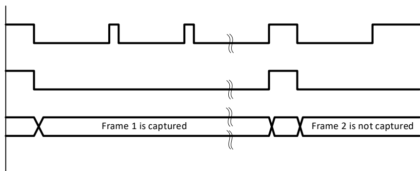
Figure 23-3 Single frame capture waveform in Snapshot mode
