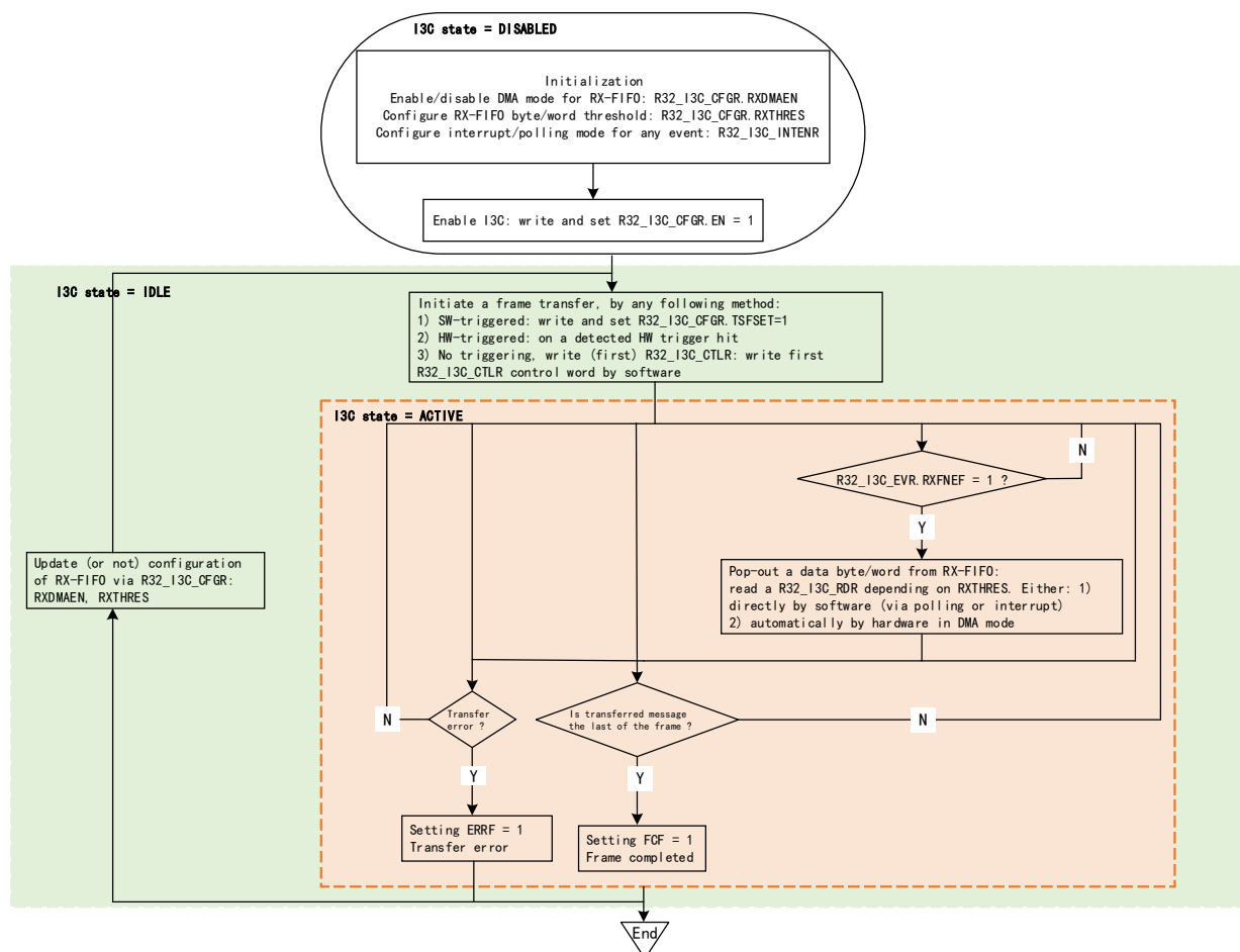
Figure 19-11 RX-FIFO management (as master)
