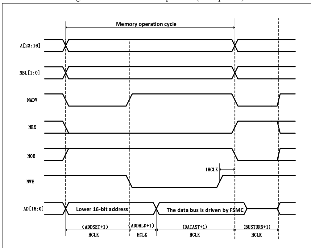
Figure 26-6 Mode A write operation (Multiplexed)
