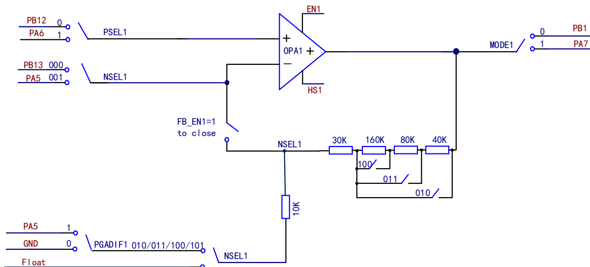
Figure 21-1 OPA structure diagram
