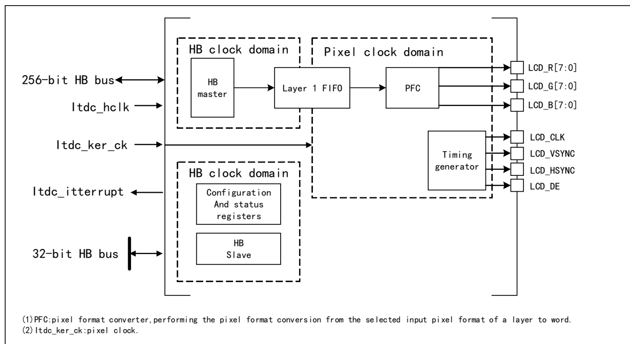
Figure 27-1 Structural block diagram of LTDC
