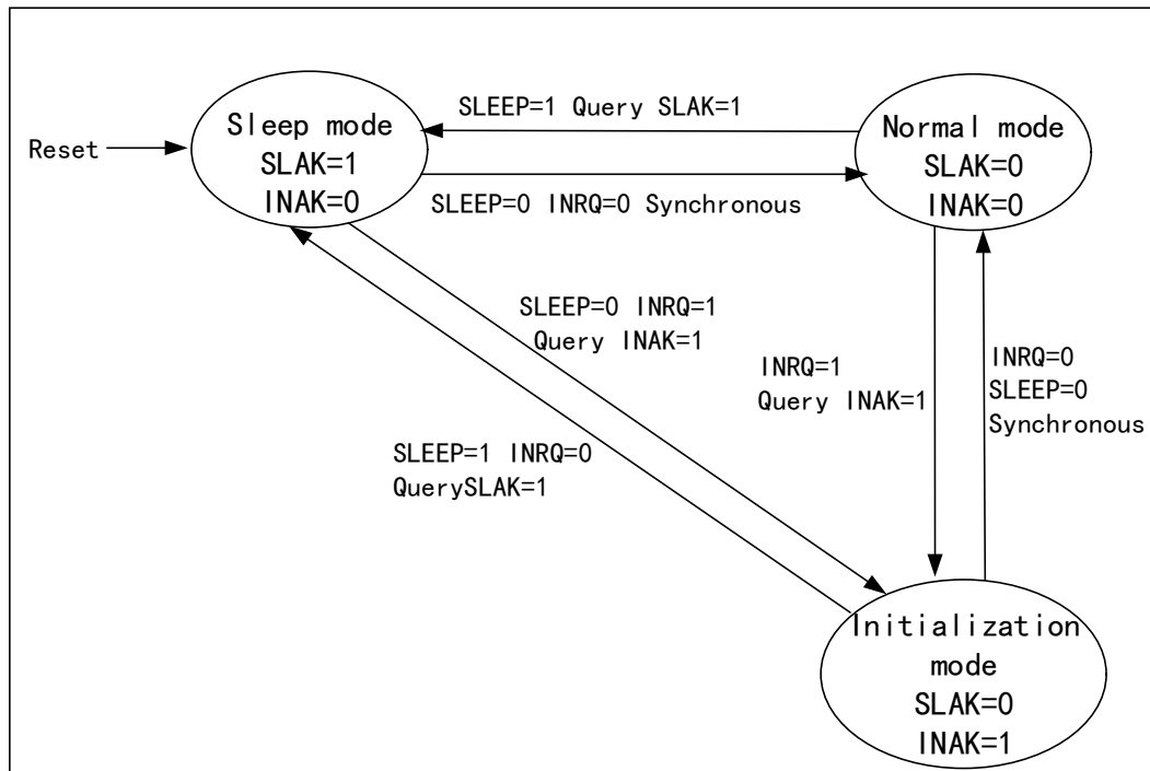
Figure 25-1 CAN operating mode switch
