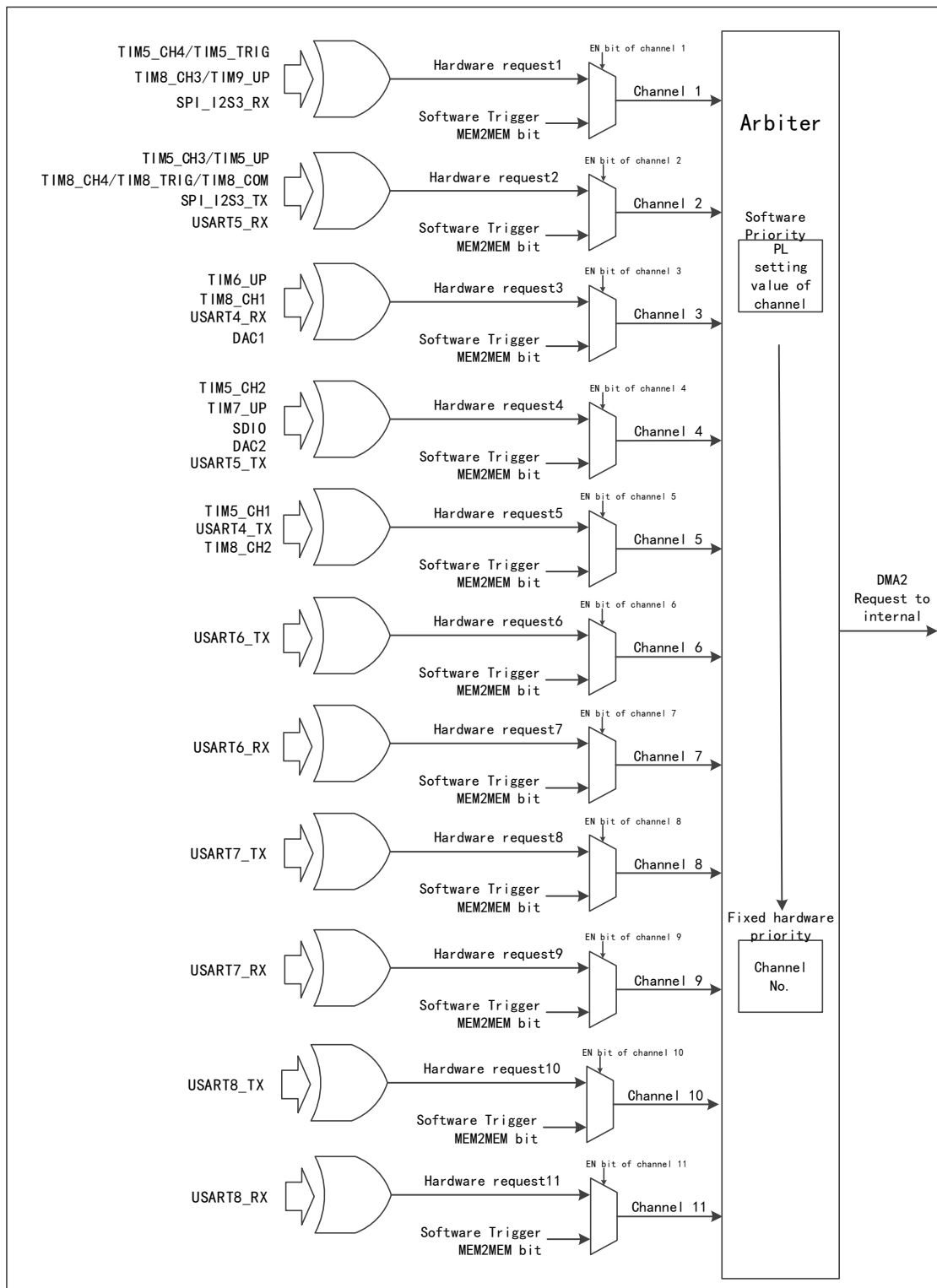
Figure 11-2 DMA2 request mapping
