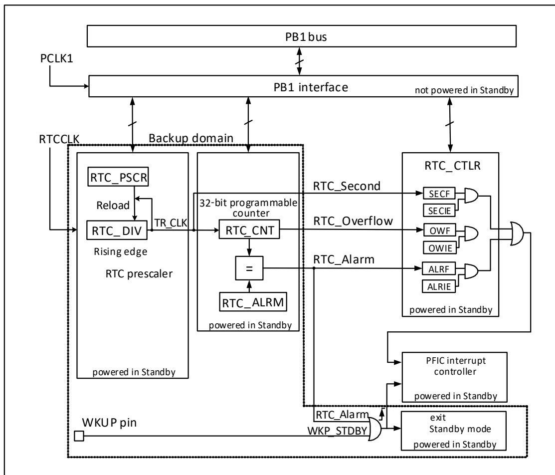
Figure 6-1 RTC structure diagram
