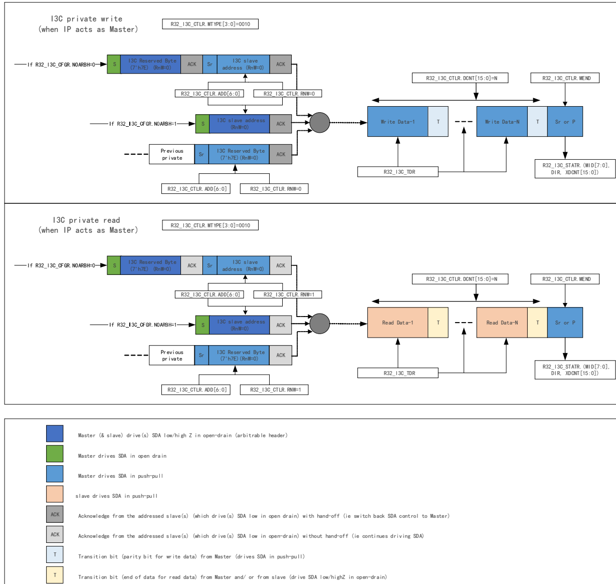
Figure 19-5 I3C private read/write message (as master devices)
