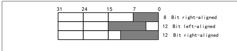
Figure 13-2 Data formats in single channel mode
