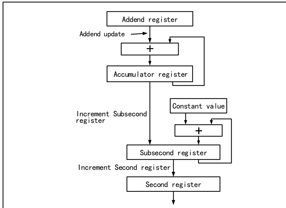
Figure 29-2 Process for updating time using fine correction
