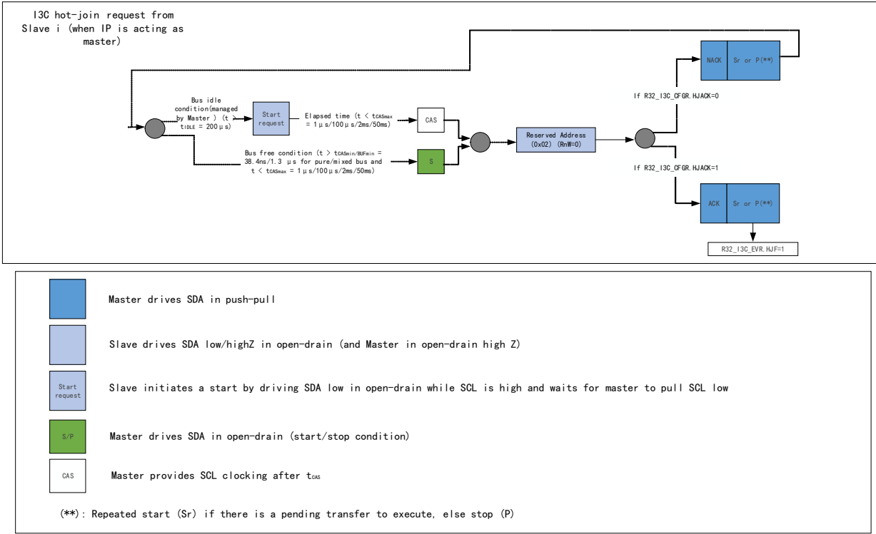
Figure 19-8 I3C hot join request transfer (as master devices)
