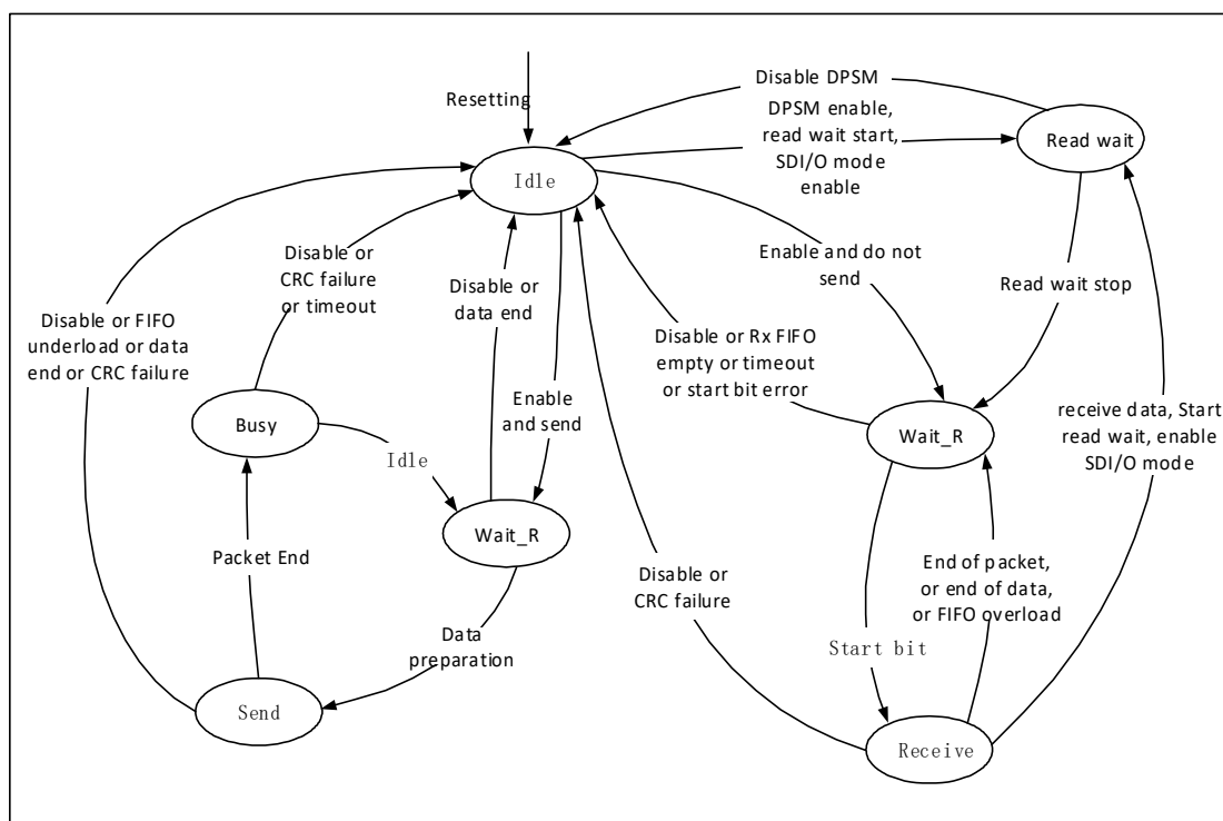
Figure 24-3 Data path state machine
