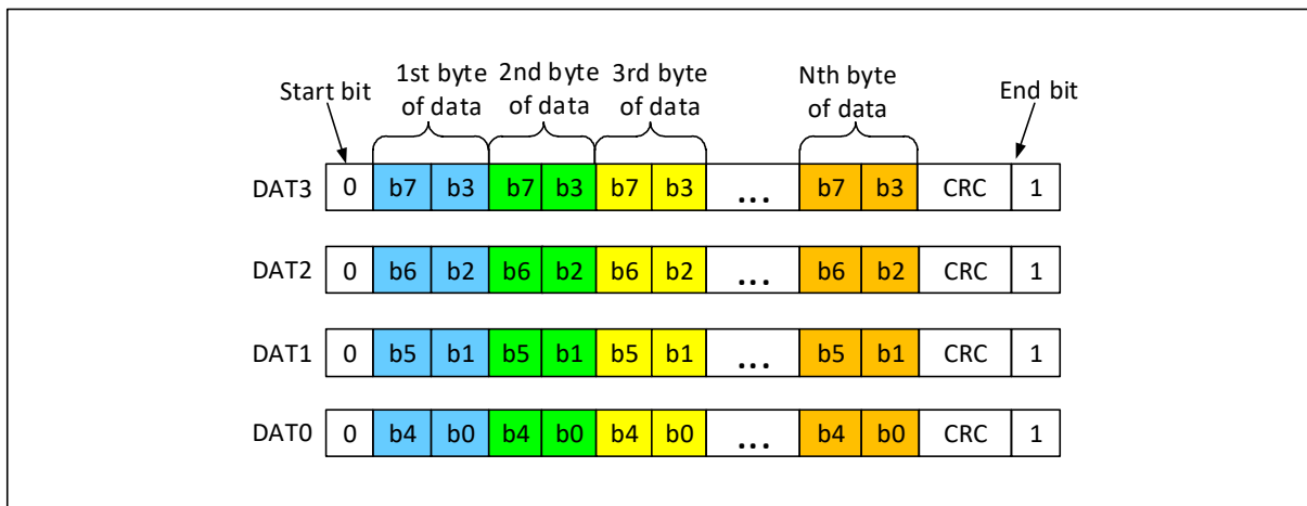
Figure 24-10 SD card 4 bus data transfer byte format
