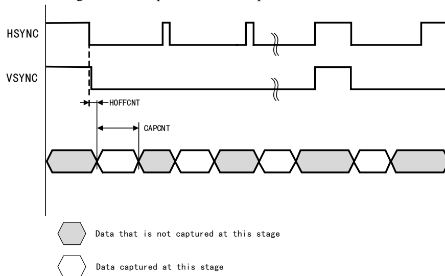
Figure 23-6 Crop window data capture waveform
