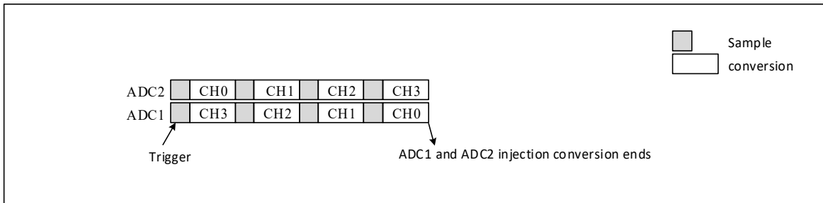
Figure 12-6 4-channel synchronous injection conversion
