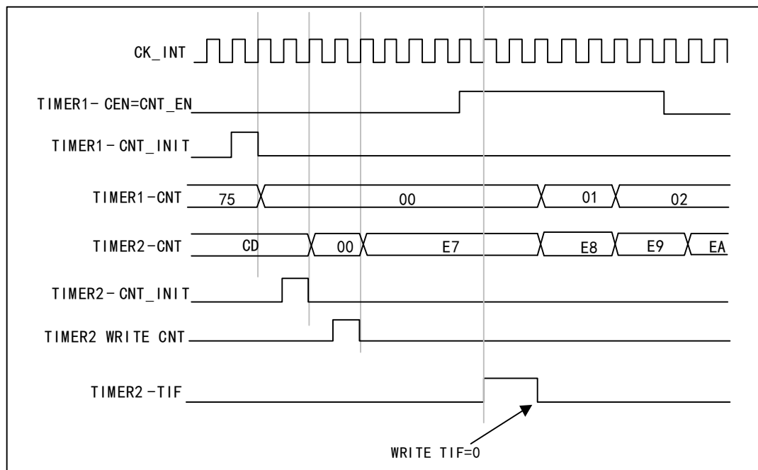
Figure 14-14 Use the enable signal of timer 1 to trigger timer 2
