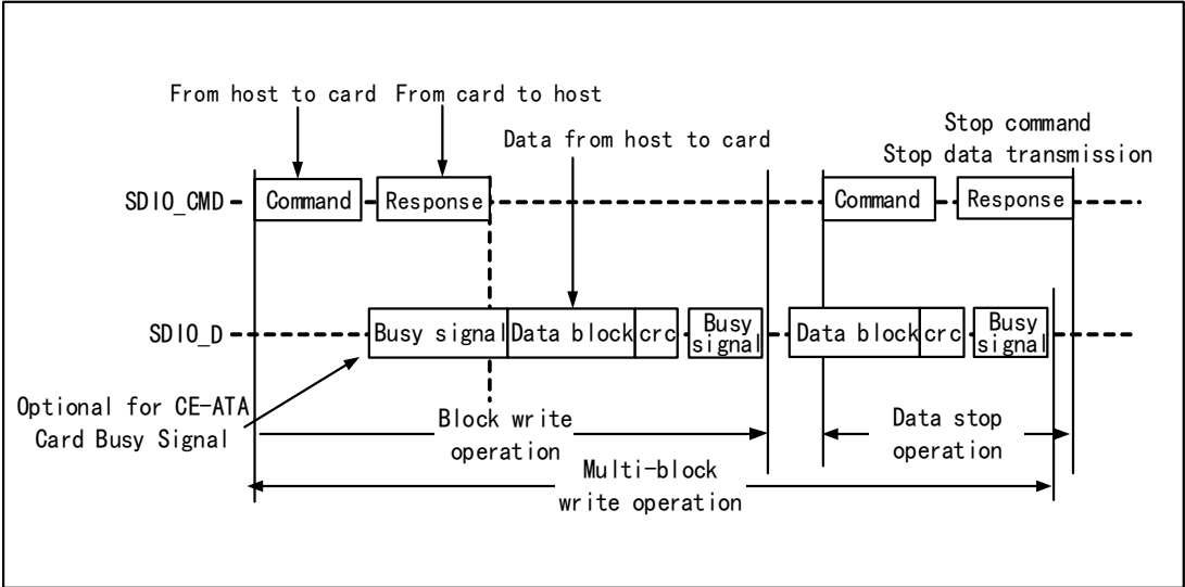
Figure 24-6 SDIO multi-block write timing (Taking SD card as an example)
