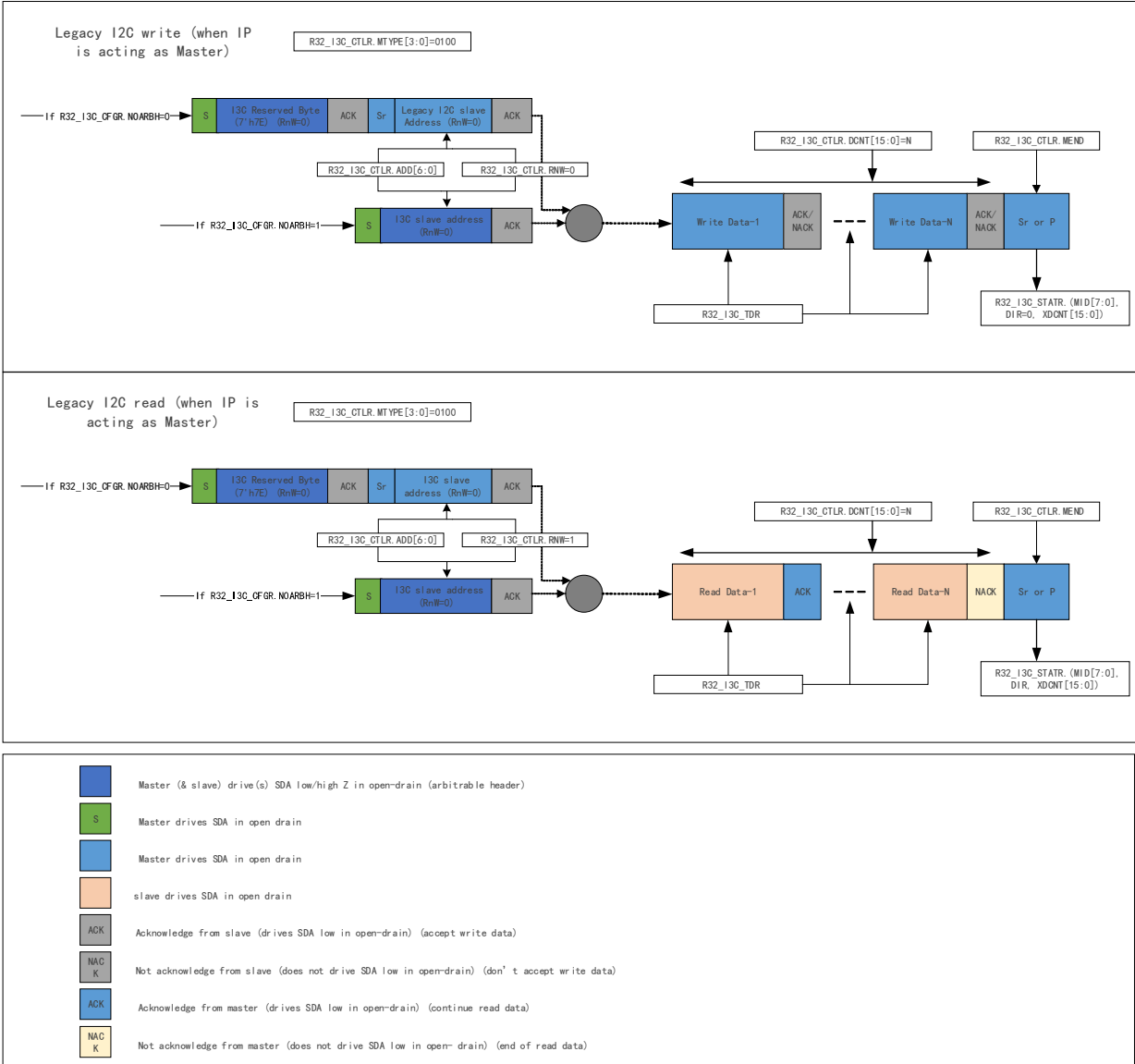
Figure 19-6 Traditional I2C read/write message (as master devices)
