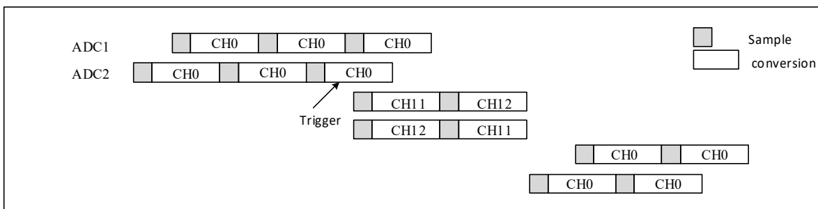
Figure 12-14 Trigger injection group switching under alternate switching
