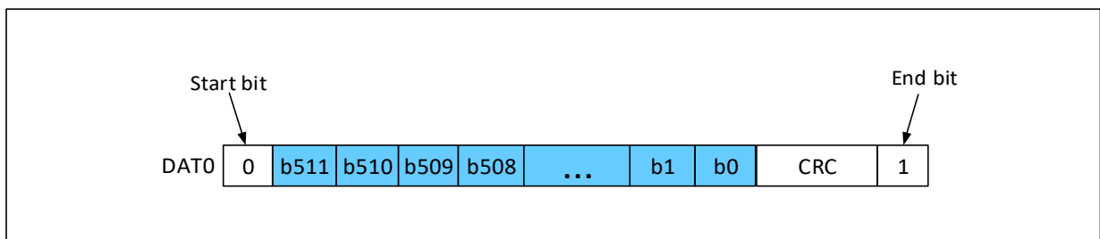
Figure 24-11 SD card single bus data transfer in a 512-bit word format
