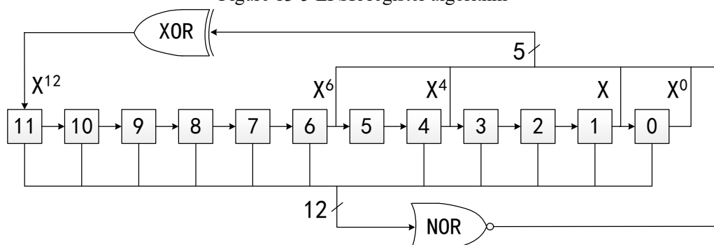
Figure 13-5 LFSR register algorithm
