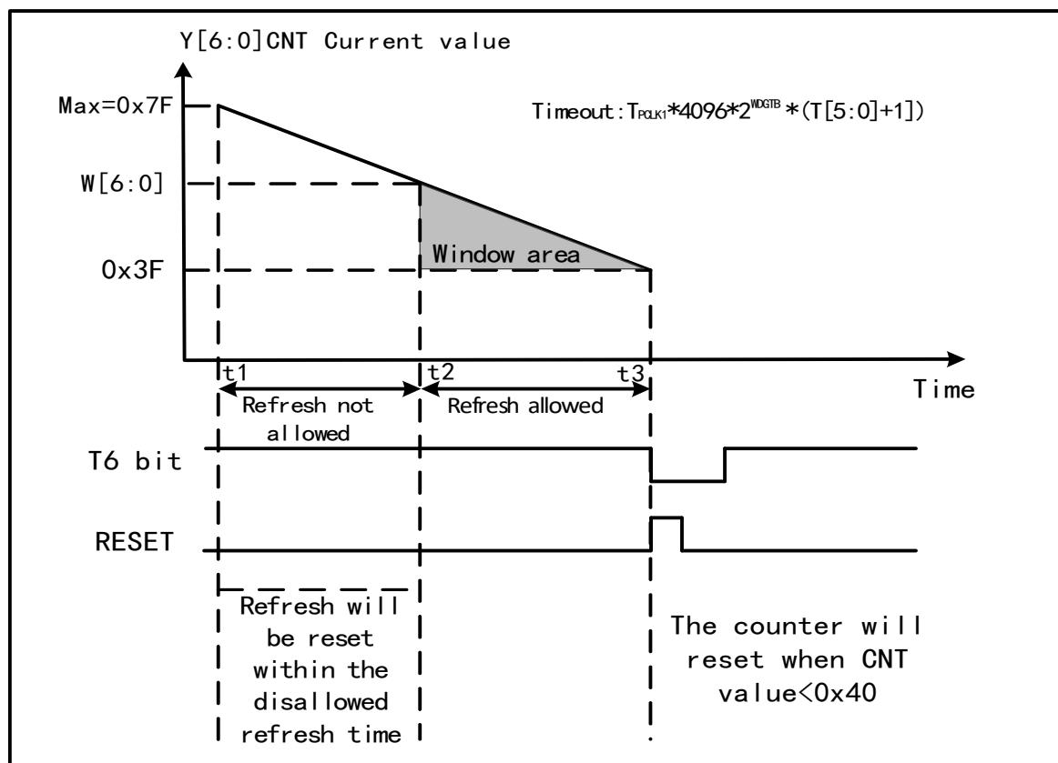
Figure 8-2 Counting mode of window watchdog
