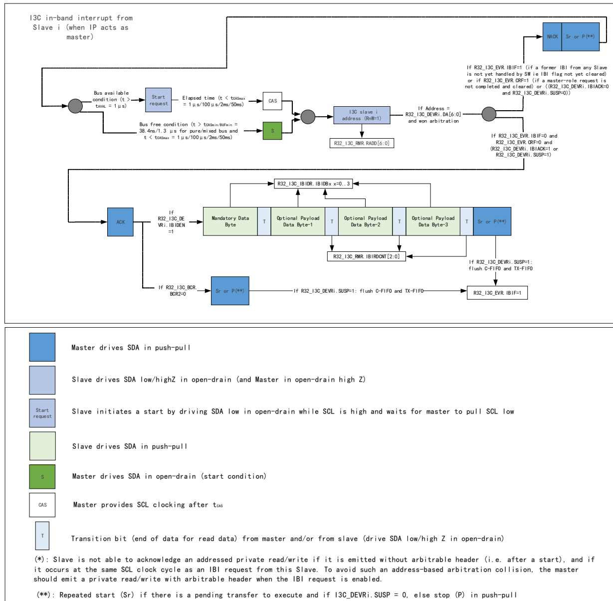
Figure 19-7 I3C IBI Transfer (as master devices)
