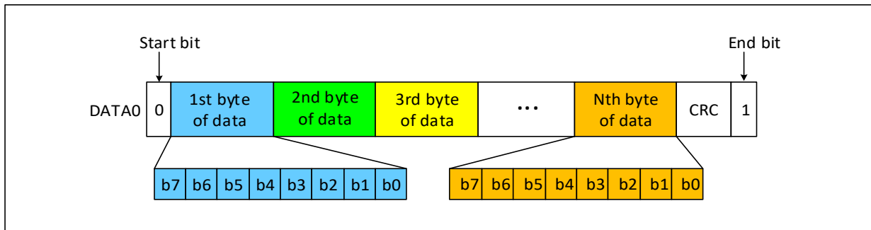
Figure 24-9 SD card single bus data transfer byte format
