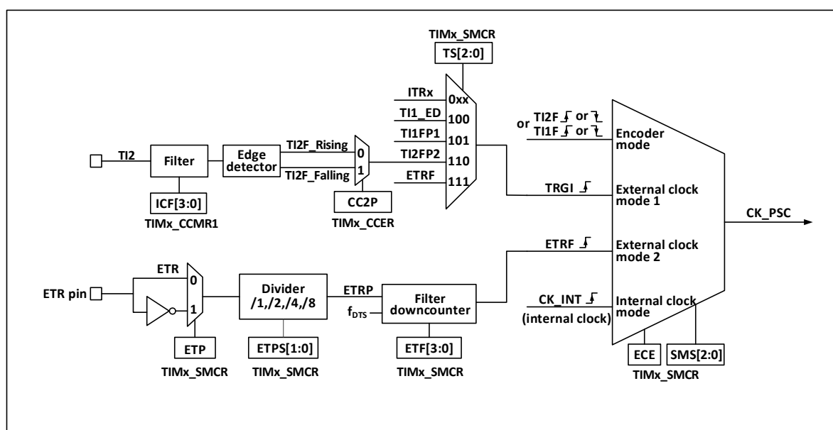
Figure 15-2 Block diagram of general-purpose timer source
