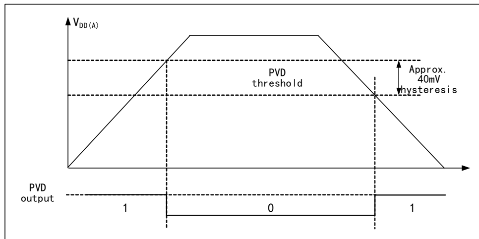
Figure 2-3 Schematic diagram of PVD operation
