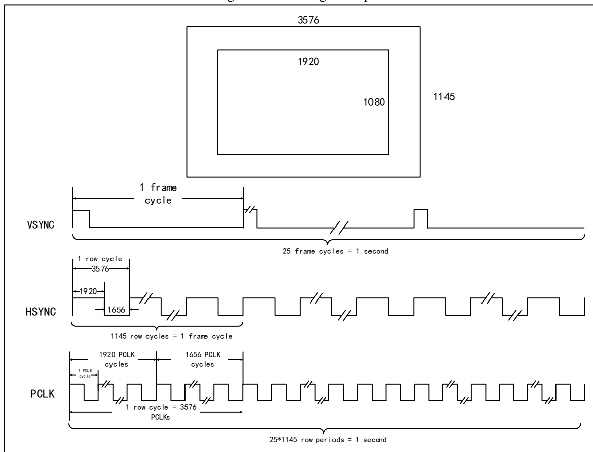
Figure 23-2 Timing description
