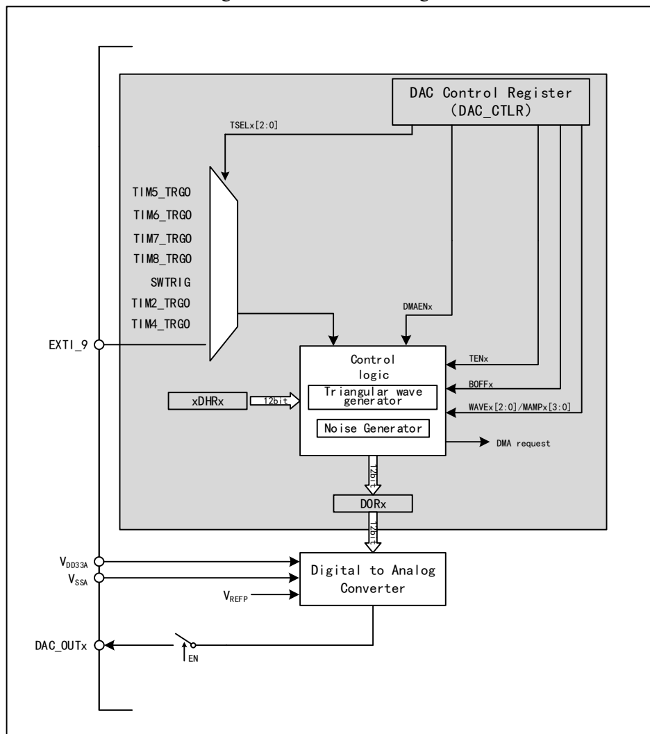
Figure 13-1 DAC block diagram
