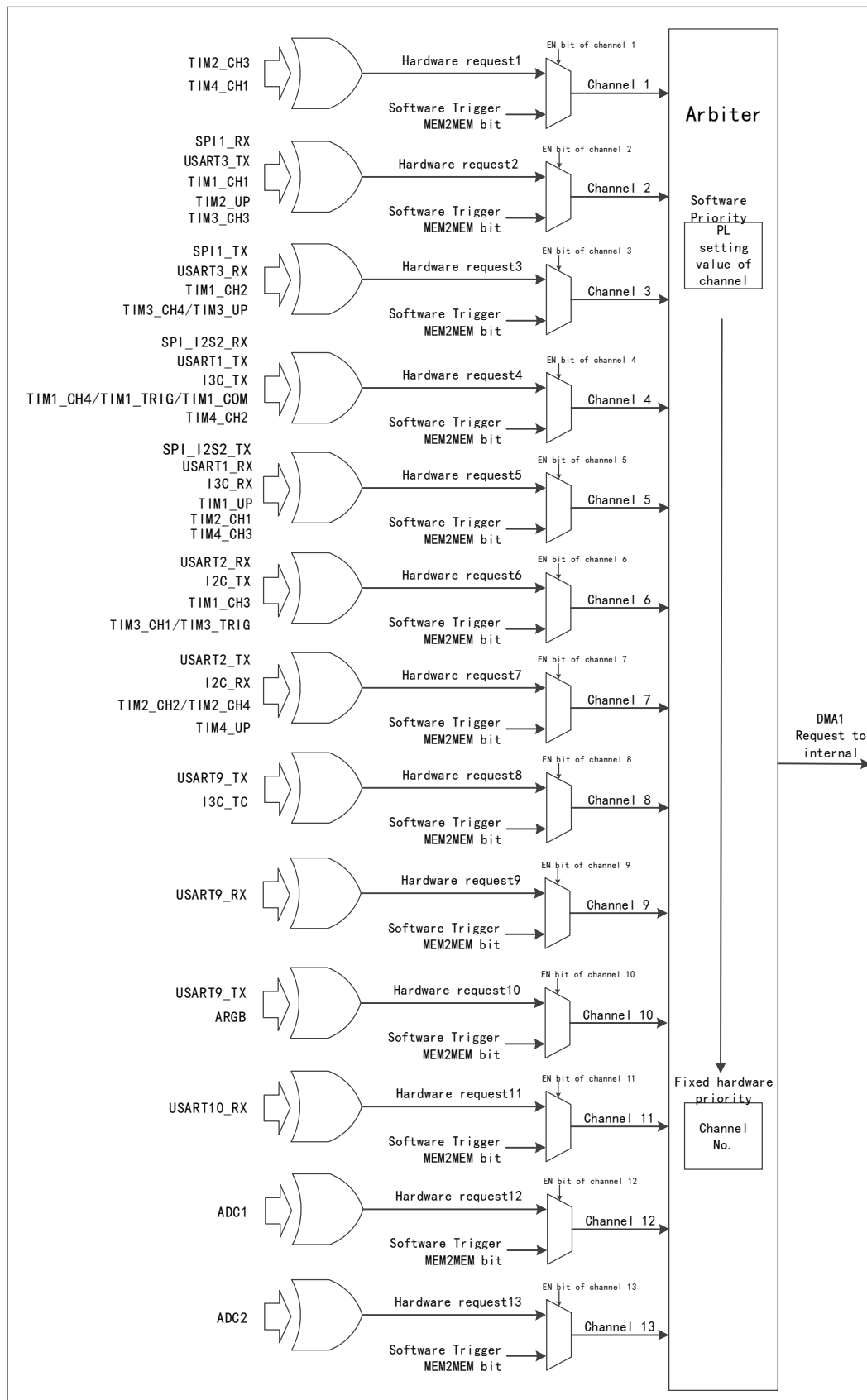
Figure 11-1 DMA1 request mapping
