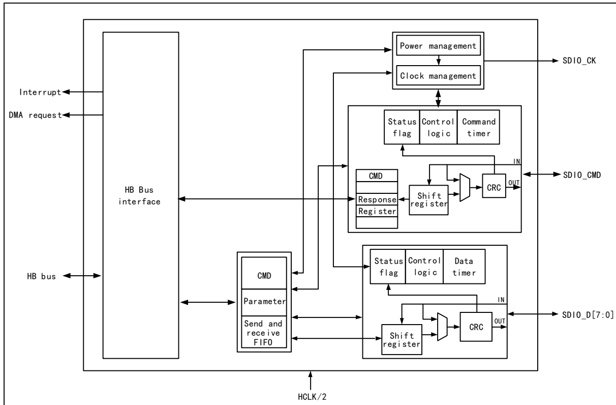
Figure 24-1 SDIO structure diagram
