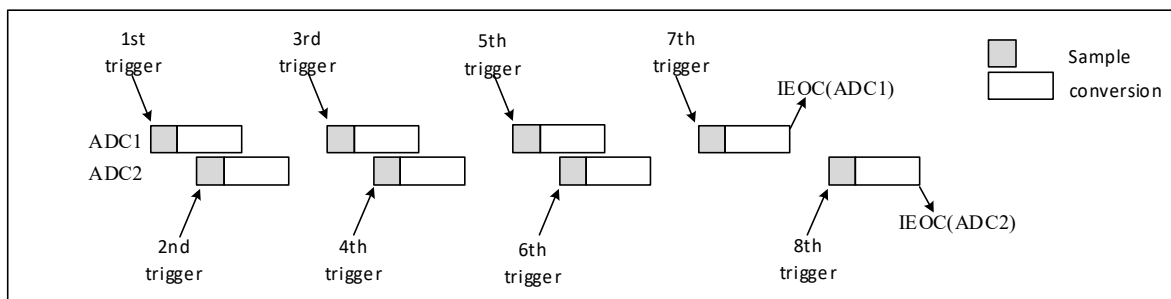
Figure 12-11 Alternating trigger transitions for each ADC injection channel in discontinuous mode
