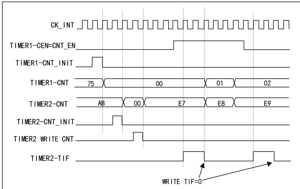
Figure 14-12 Use the enable signal of timer 1 to implement gating control on timer 2
