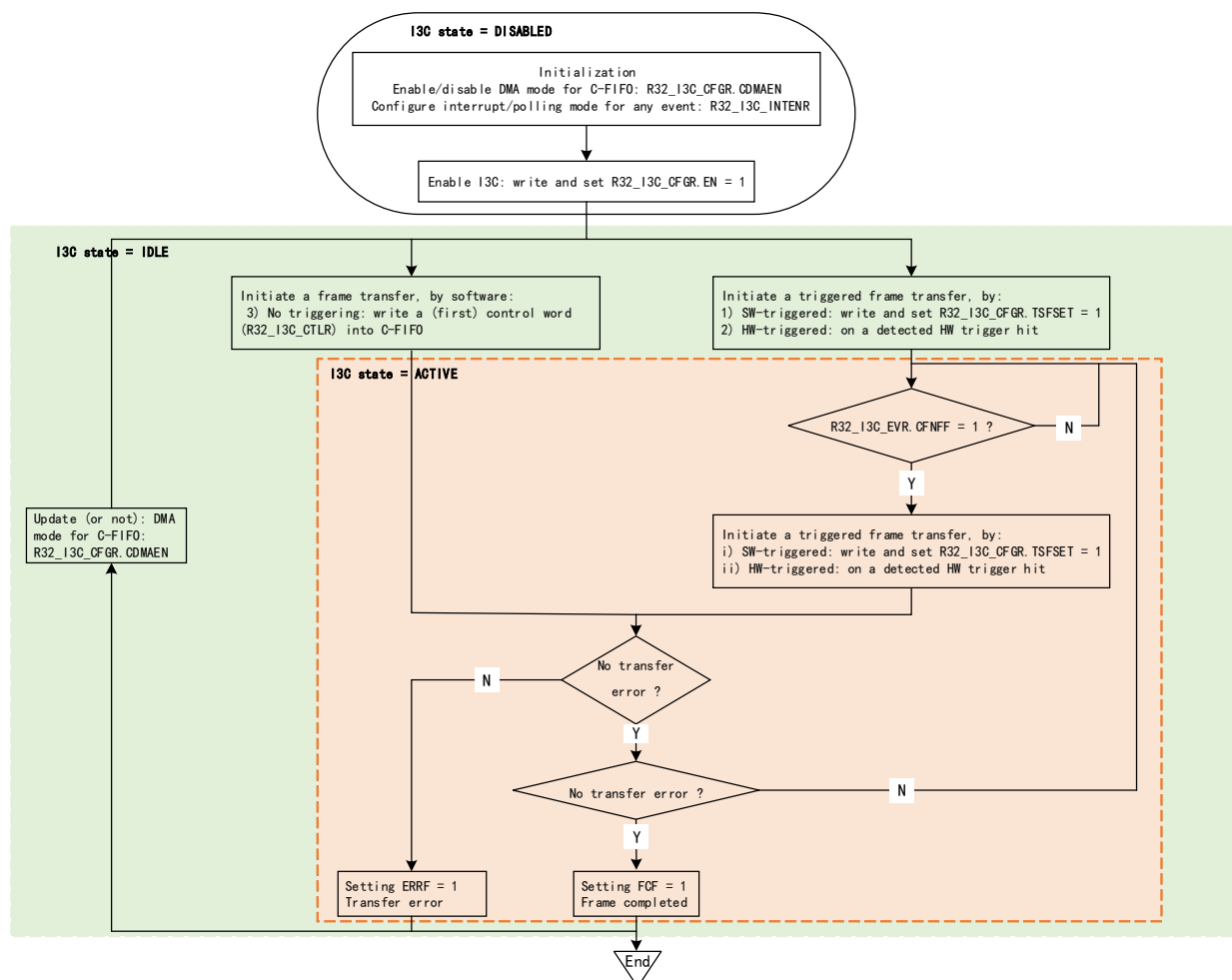
Figure 19-9 C-FIFO management (as master)
