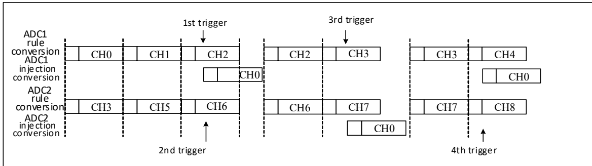
Figure 12-13 Trigger event occurs during injection transition
