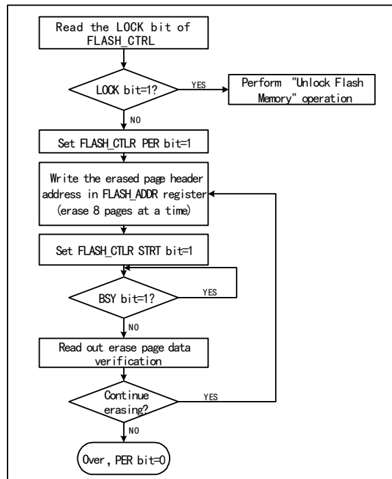
Figure 32-2 FLASH page erasure
