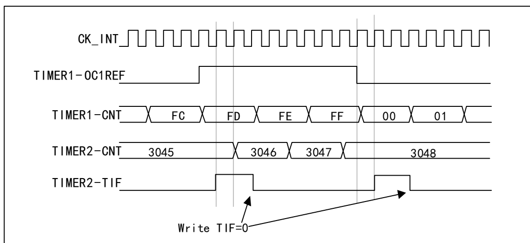
Figure 14-11 Use OC1REF of timer 1 to implement gating control of timer 2
