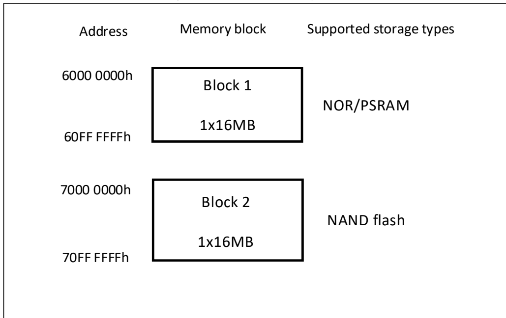
Figure 26-2 FSMC memory block
