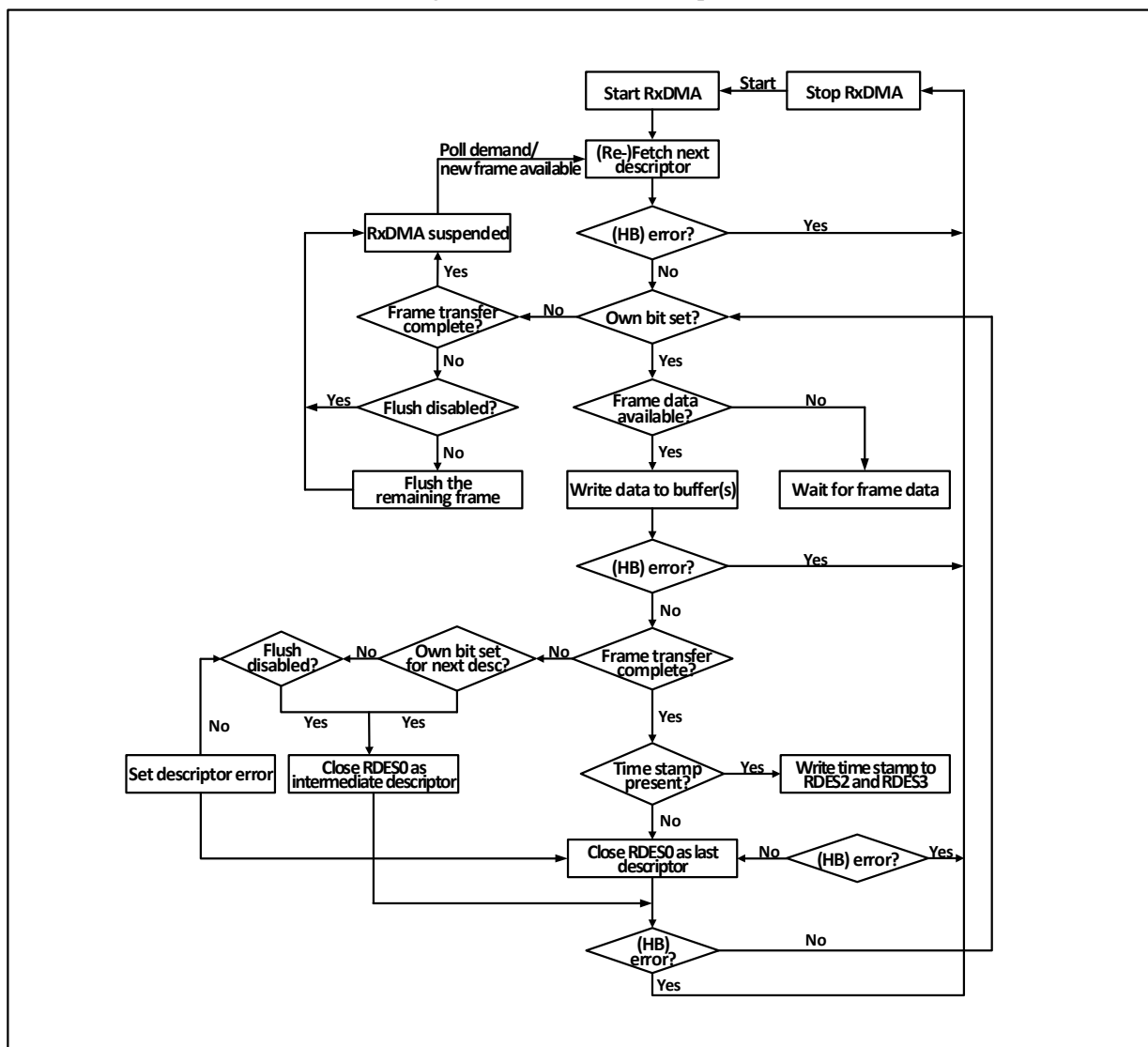
Figure 29-5 Process of reception
