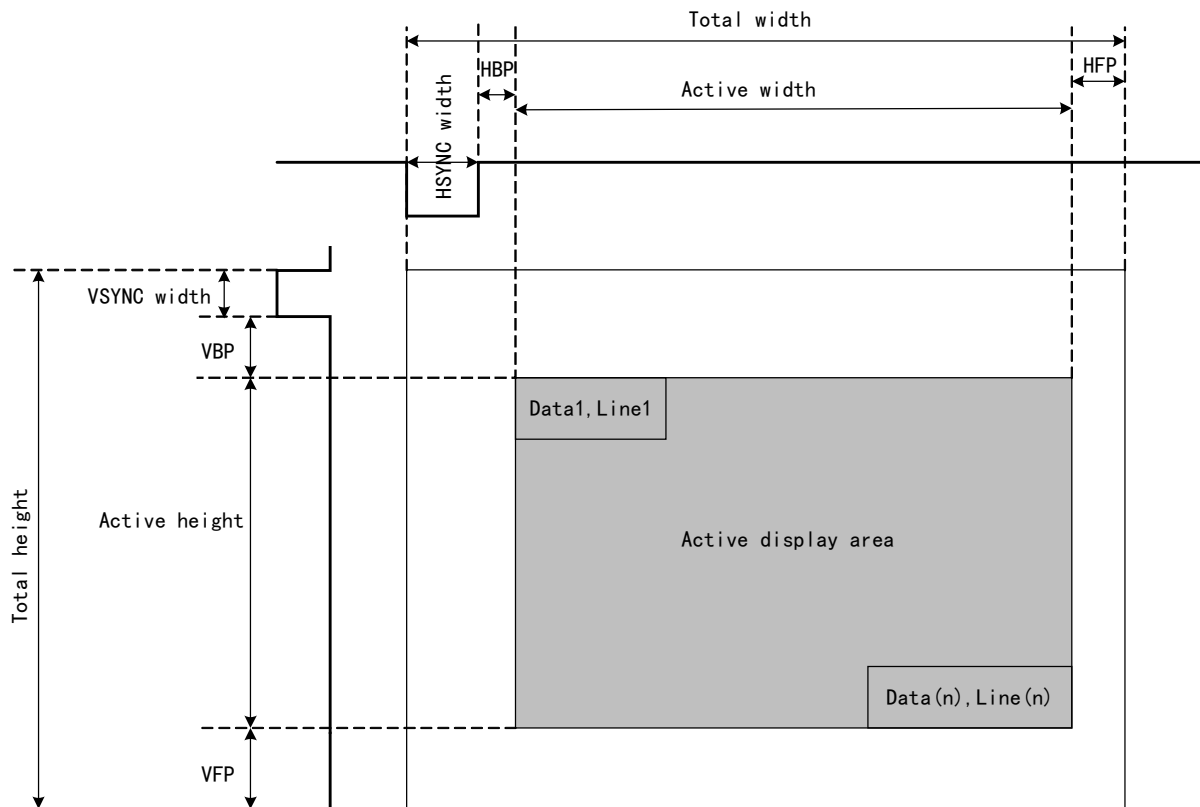
Figure 27-2 LTDC synchronization timing
