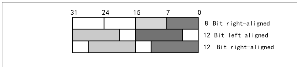
Figure 13-3 Data formats in dual channel mode
