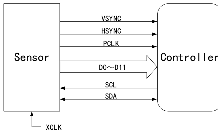
Figure 23-1 DVP interface connection
