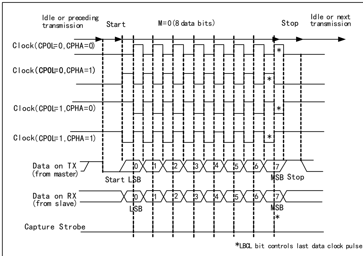
Figure 17-2 Example of USART clock timing (M=0)
