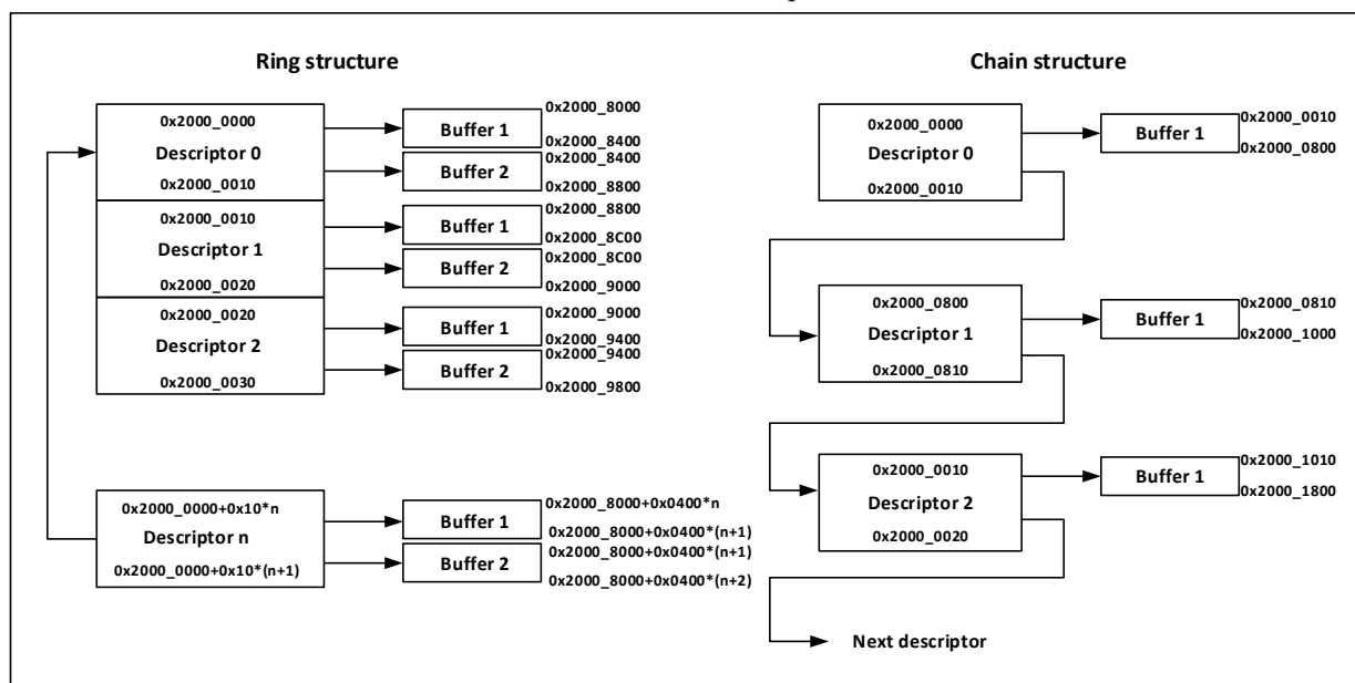
Figure 29-3 A buffer allocation scheme which describes the ring structure and the chain structure for reference when users allocate space.
