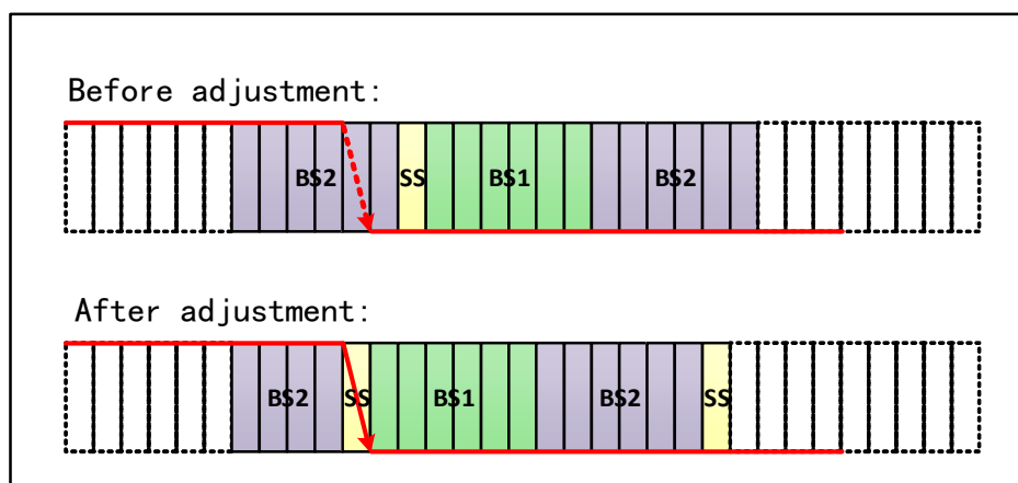
Figure 25-8 The jump appears in BS2
