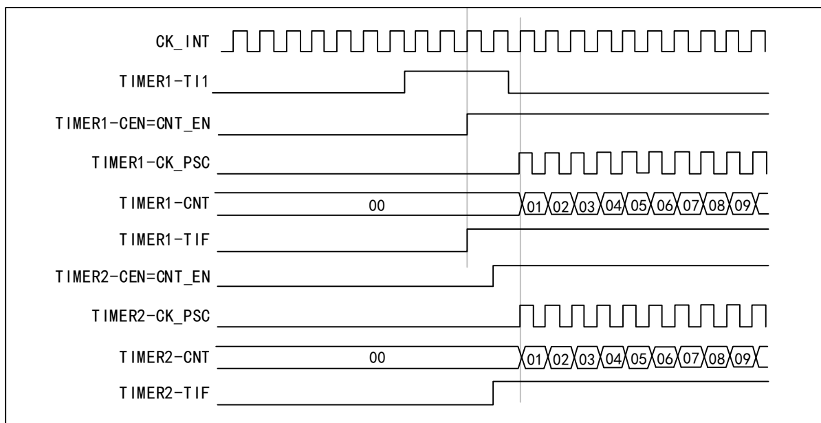
Figure 14-15 Trigger Timer 1 and Timer 2 using the TI1 input of Timer 1
