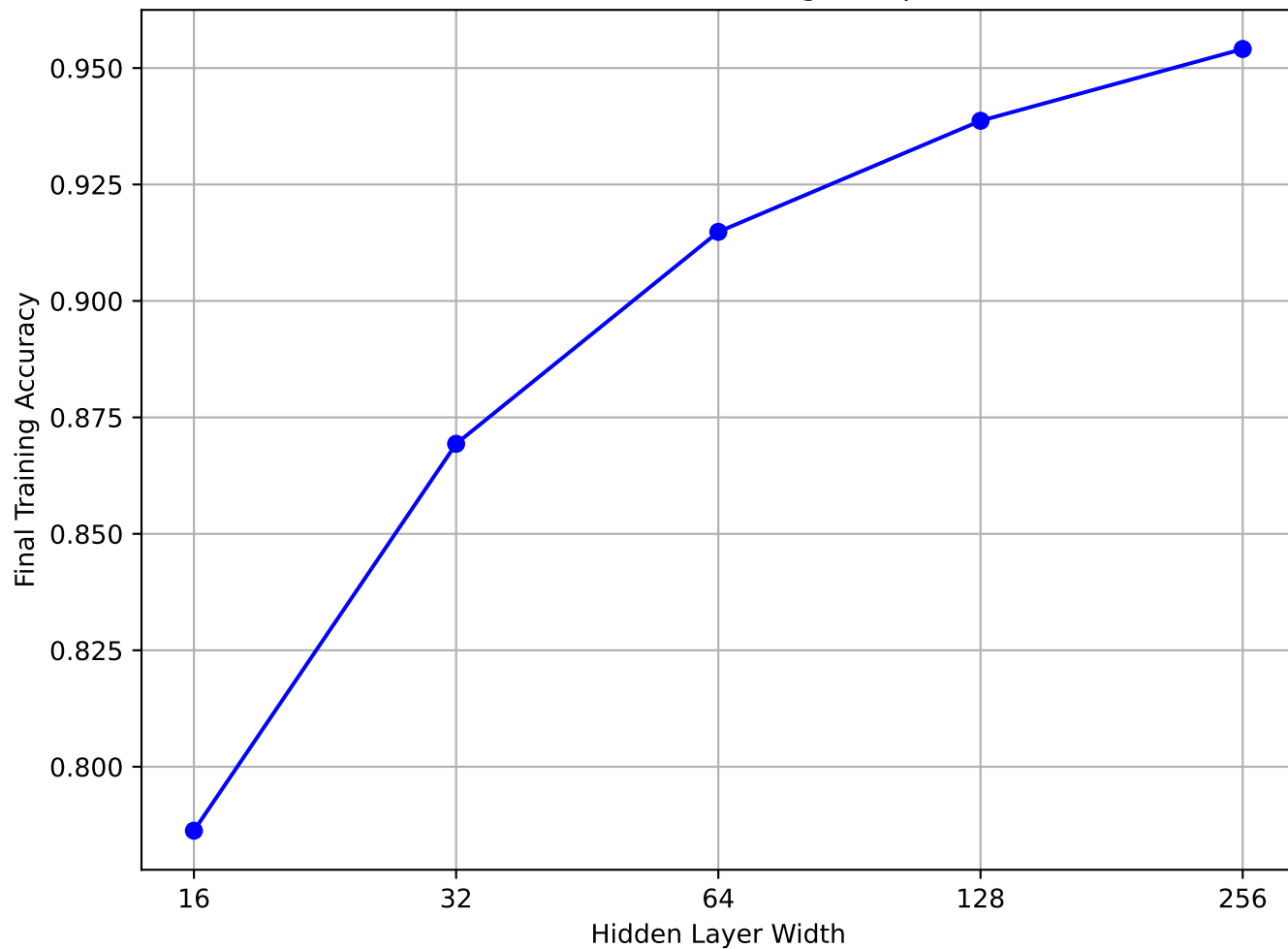
Effect of Width on Training Interpolation
