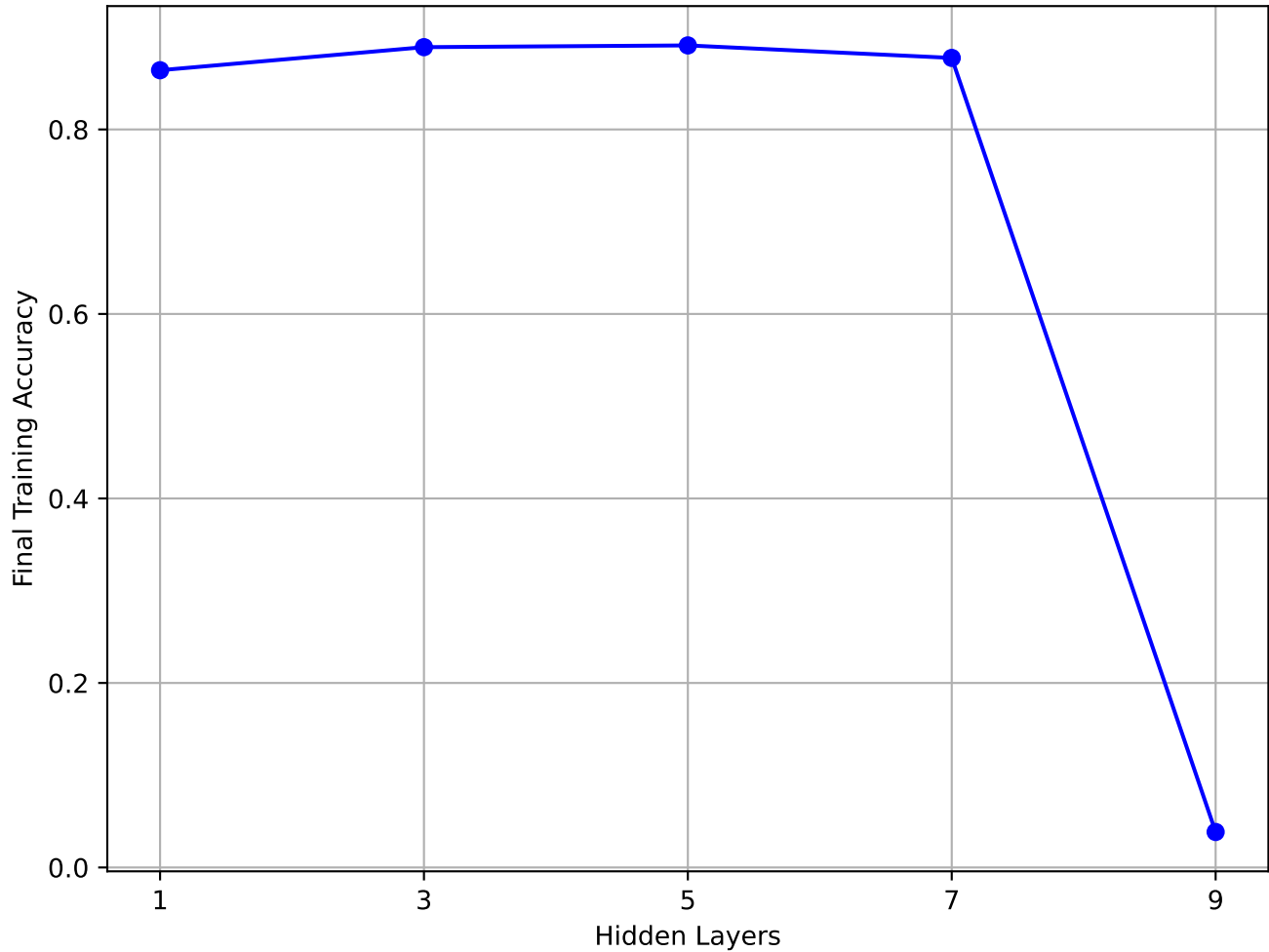
Training accuracy in the function of depth
