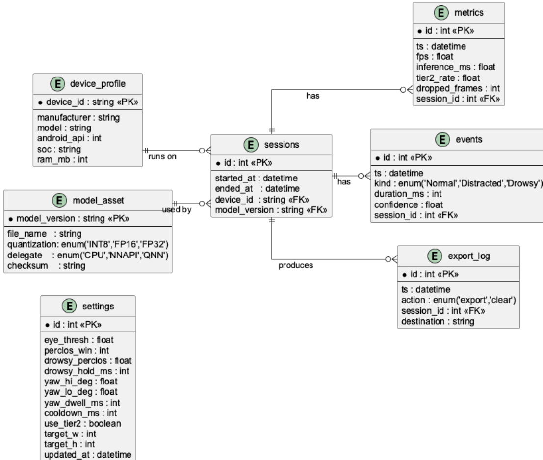
Figure 6.3: Data persistence model: User profiles are stored in the cloud (Firebase), while device-specific settings and calibration baselines are persisted locally.
