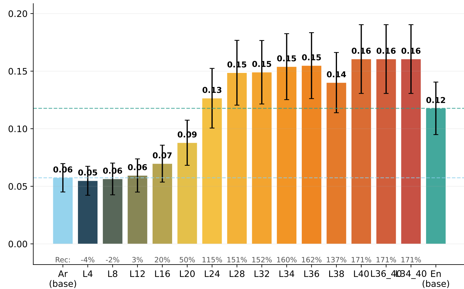
Mistral-Small-3.2-24B
