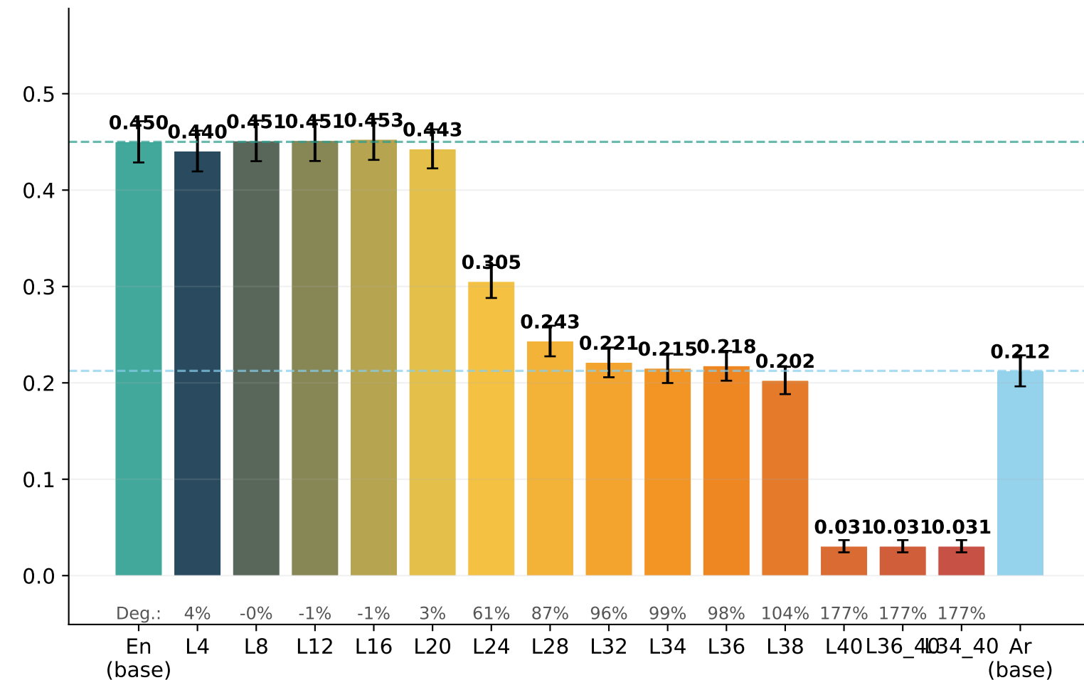
Mistral-Small-3.2-24B
