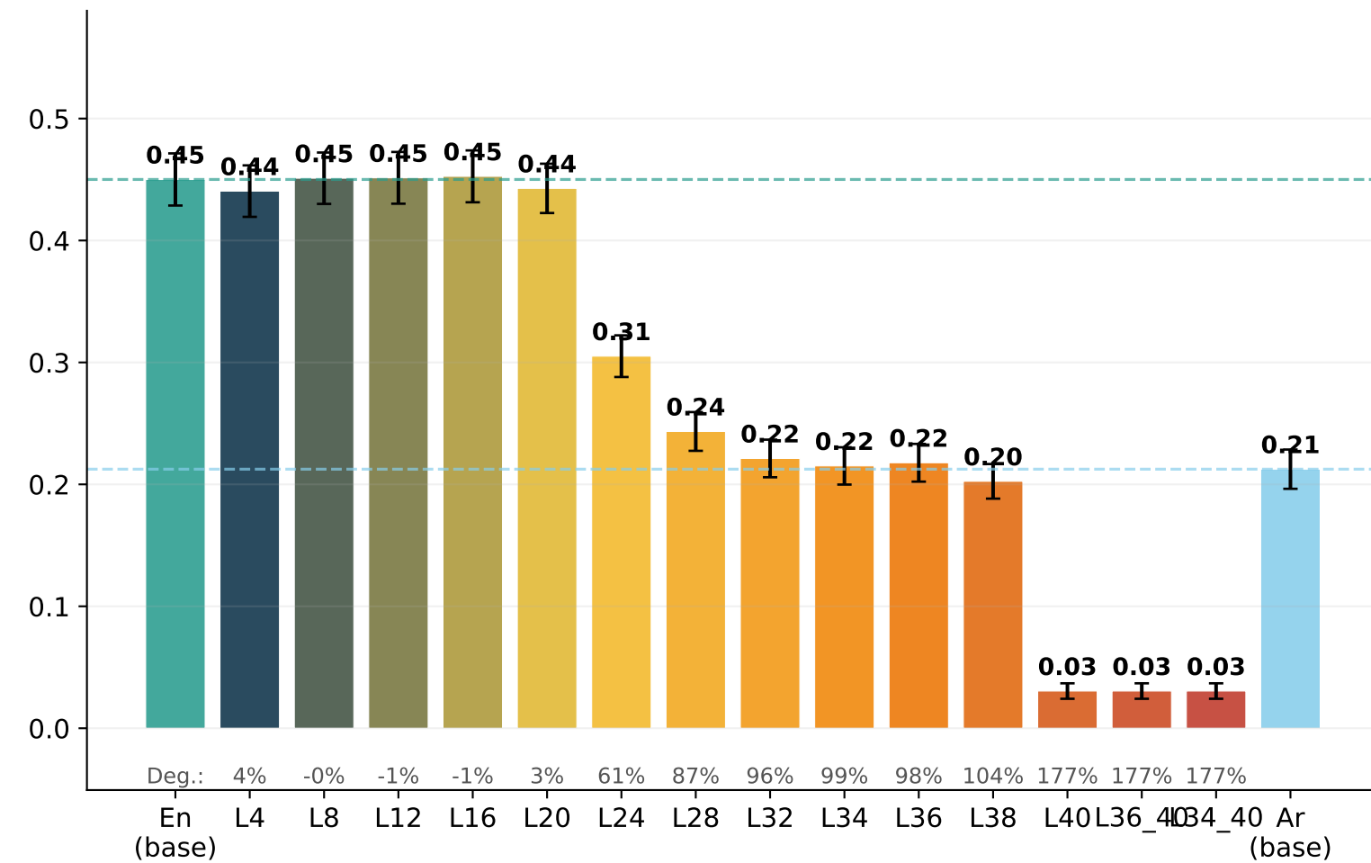
Mistral-Small-3.2-24B
