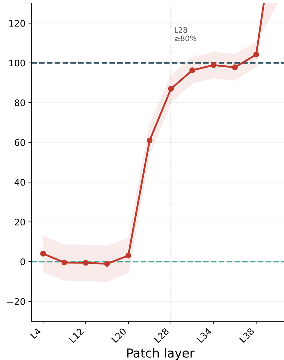
Mistral-Small-3.2-24B
