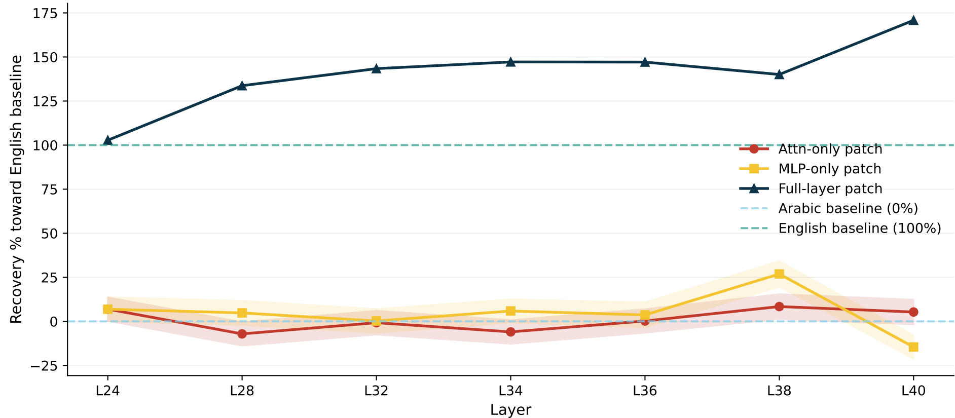
Attention vs MLP Decomposition of Activation Patching Mistral-Small-3.2-24B · MedAraBench · access_gap (En✓ ArX)
