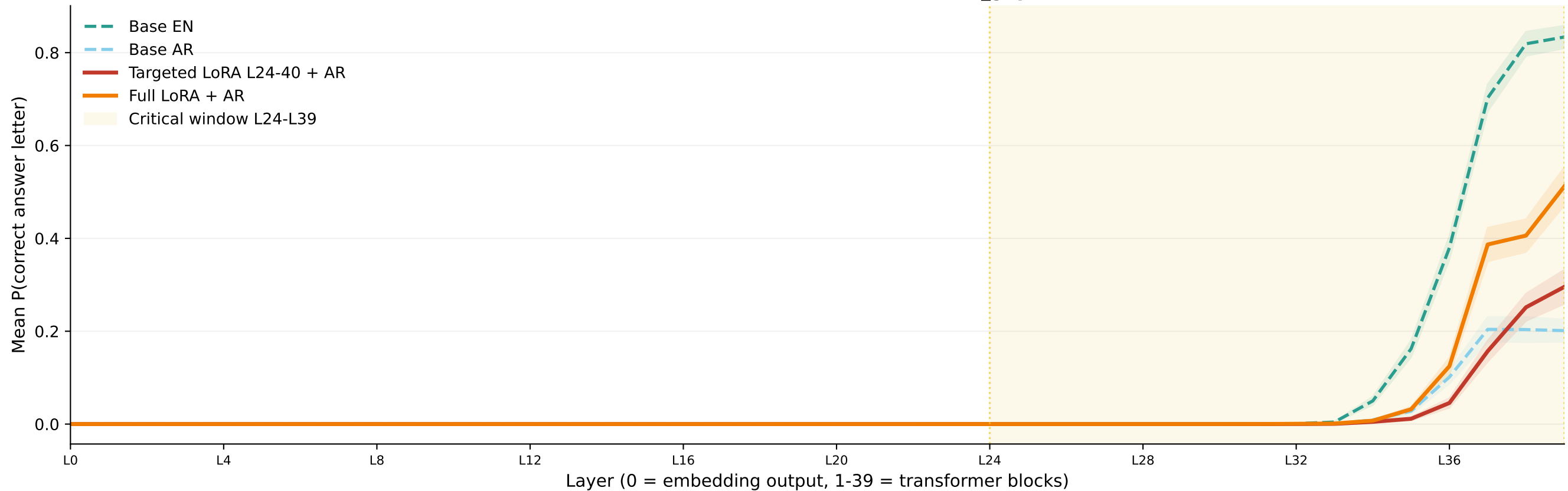
Direct Logit Lens: Full Layer View (L0-L39) Mistral-Small-3.2-24B · MedAraBench · access_gap (En✓ ArX)
