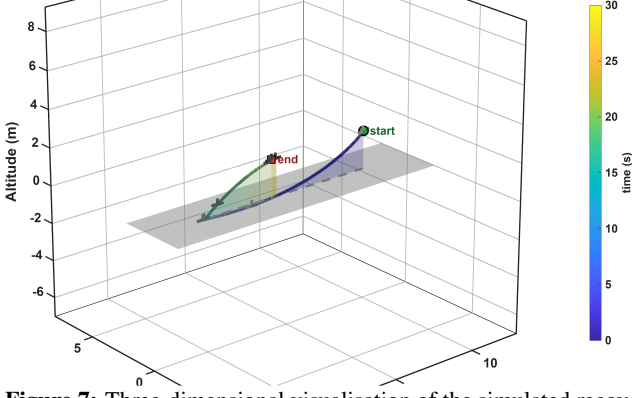
Figure 7: Three-dimensional visualisation of the simulated recovery trajectory.
