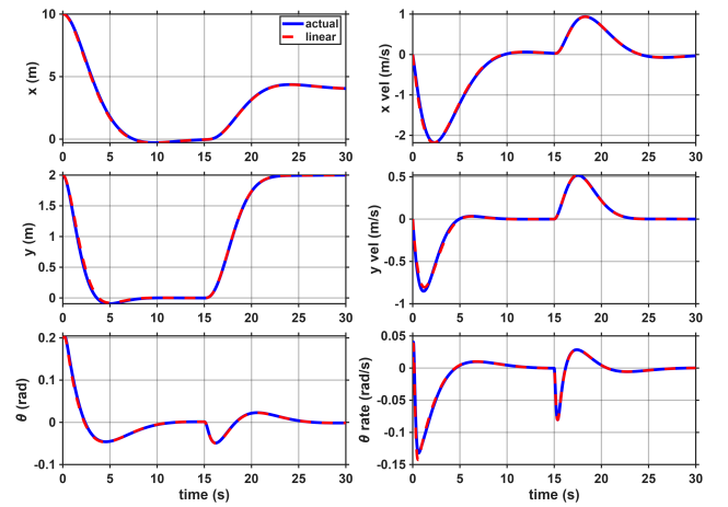
Figure 2: Linearised-model state response compared with the nonlinear plant. The close agreement confirms that the nominal response remains inside the local hover-linearisation region.
