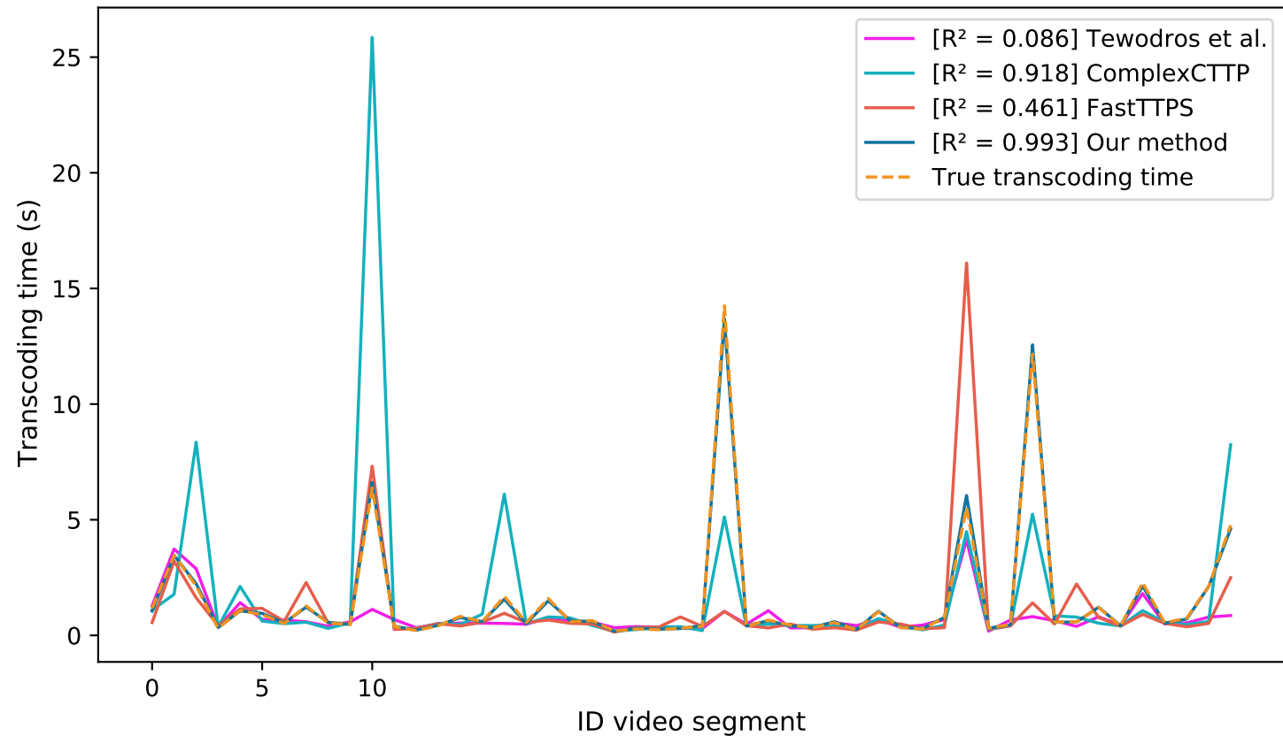
True transcoding time vs Predicted transcoding time
